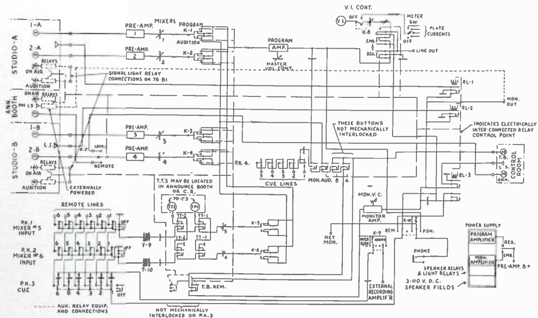
Simplified schematic of the 76-B1.
