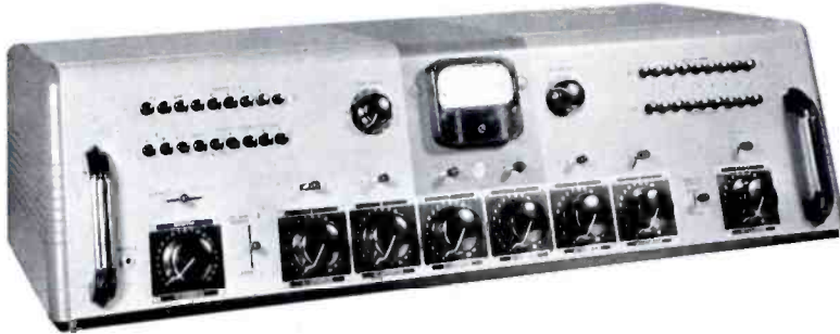
Neat, compact design emphasized in the RCA 76 B1 Consolelette.
