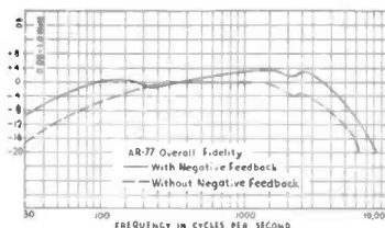
Performance Curve plotted on the AR 77.
