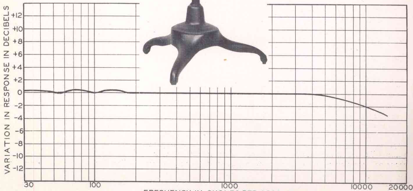
FIG. 6 TYPE 44-AP PROGRAM VELOCITY MICROPHONE
