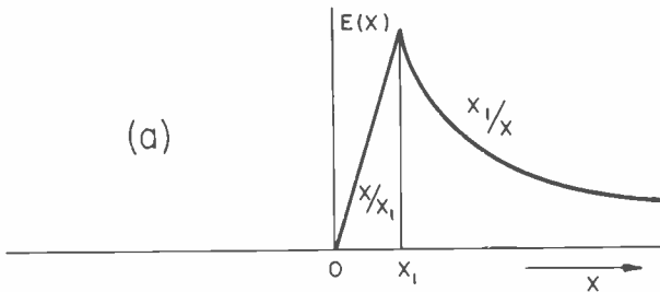
FIG. 13a. A cosecant field distribution.
