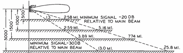
MINIMUM SIGNAL LOCATIONS UHF ANTENNA TYPE TFU-24-8H 18-BAY CHANNEL 76 84.4 MC
