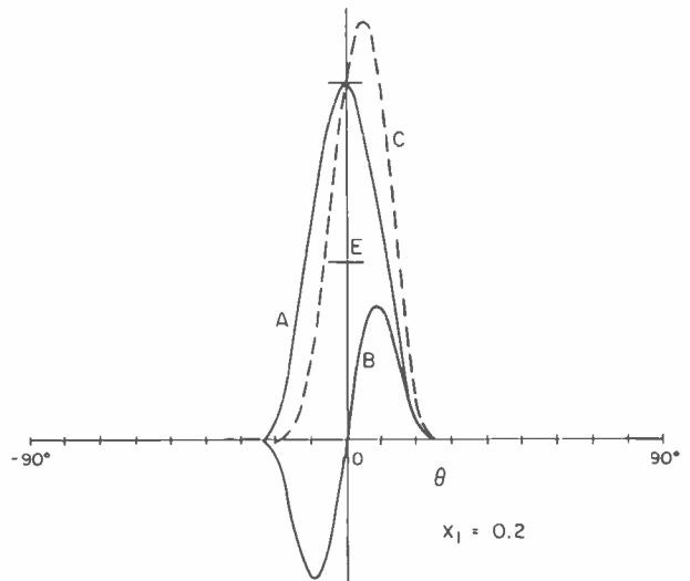
FIG. 8. Lobe-switching antenna patterns similar to Fig. 6. ( x_1 = 0.2 )
