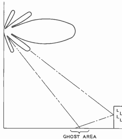
FIG. 11. This shows how large variations in a null-filled pattern could cause severe "ghosting" under certain conditions when the reflected signal from a peak is of the same order as the direct signal from a valley in the pattern.
