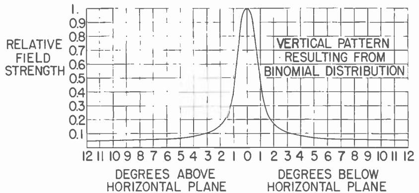
FIG. 13. A null-free pattern resulting from binomial distribution.
