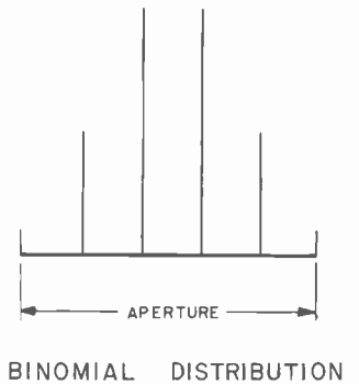
BINOMIAL DISTRIBUTION FIG. 12. When the amplitude in successive radiators is varied as shown, a null-free pattern results.
