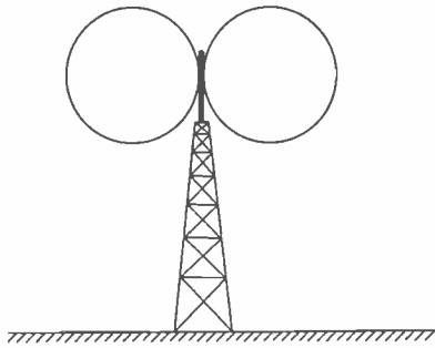
VERTICAL PATTERN SINGLE BAY OMNIDIRECTIONAL ANTENNA POWER GAIN - 1
