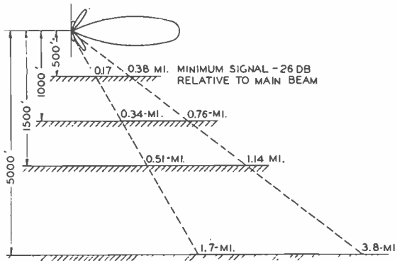
MINIMUM SIGNAL LOCATIONS STACKED OMNIDIRECTIONAL ANTENNA POWER GAIN 5.0
