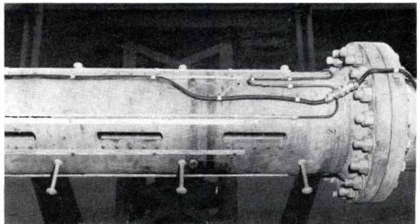
FIG. 7. Cylindrical couplers are mounted in the inside edge of the slot.
