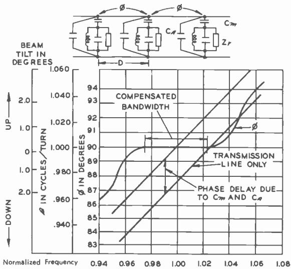
FIG. 5. Compensated phase response across the television channel.
