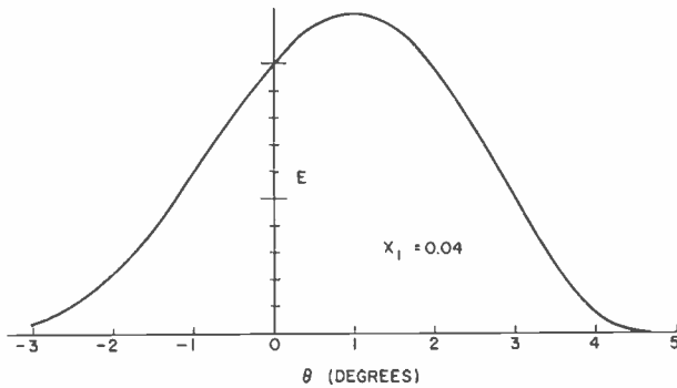
FIG. 10. A very narrow tilted beam. ( x_1 = 0.04 )
