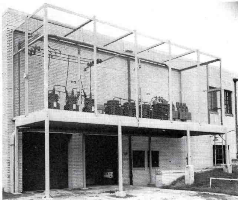
FIG. 5. All station power transformers are mounted on this platform on the side of the building. The three transformers on the left supply 440 volts to the Ampliphase transmitter.
