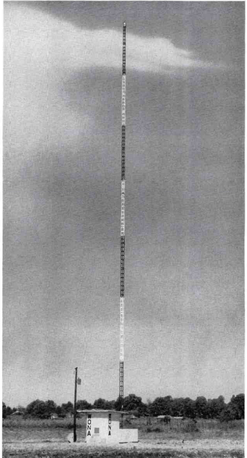
FIG. 8. The 206 foot Stainless steel tower dwarfs the transmitter building. The tower is mounted on a four foot concrete pier, making the total height 210 feet.
