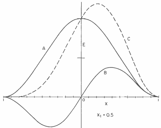
FIG. 7. The field distributions of Fig. 6 replotted as a function of x ( x = \sin \theta ).
