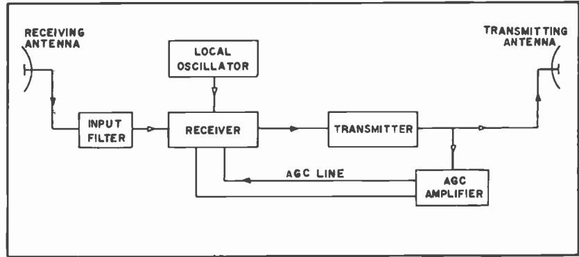
FIG. 2. Block Diagram Television Relay Unit, TVR-1.
