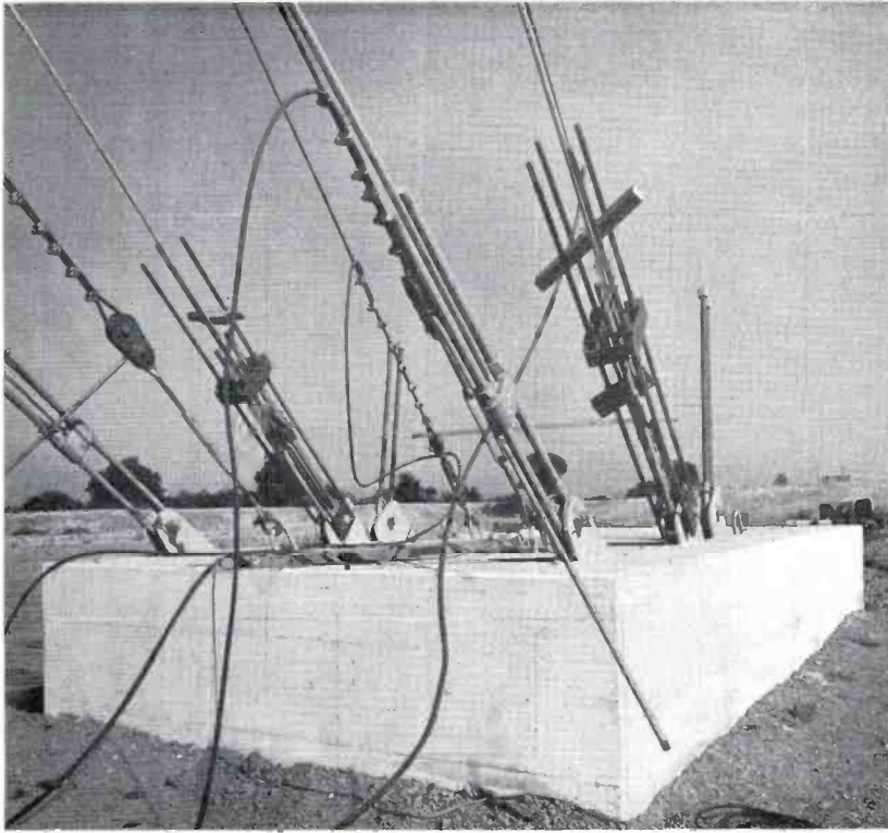
▲ FIG. 6. One of the guy anchors during construction. The "haywire" guys are temporary and were removed after tower completion. The permanent guys are identified by their considerably thicker cross-section.
