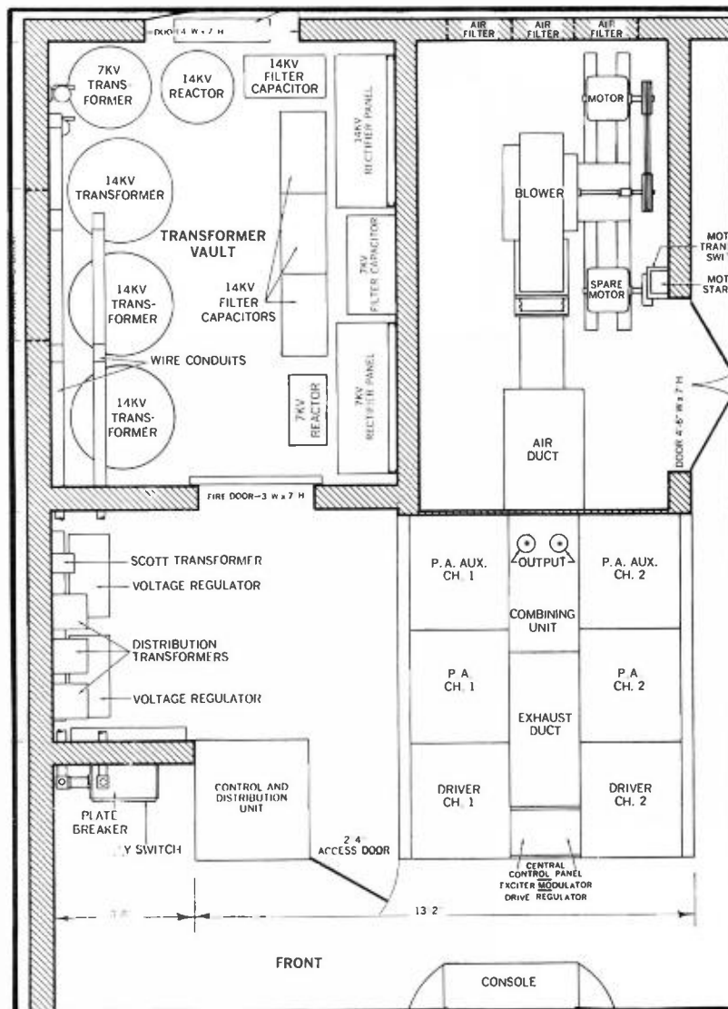
FIG. 2. Typical floor plan for BHF-100A ("old" 50-kw had a floor area—shown by heavy lines—approximately 25 per cent greater than the "new").
