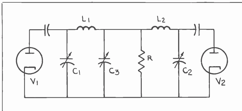
FIG. 3. Simplified PA output circuit.
