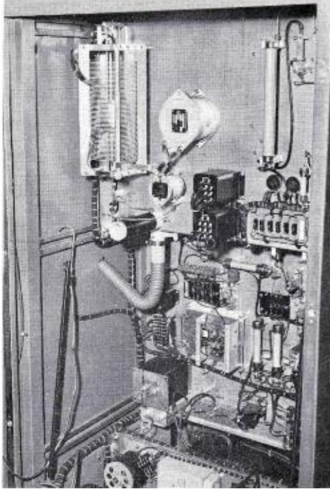
FIG. 5. The rear of the exciter/driver cabinet. The large coil in the upper left is the broadbanded tank for the 4-400A tetrode driver. Note the "potted" transformers, snap-in power resistors, etched-wiring oscillator circuit and the laced-harness wiring.
