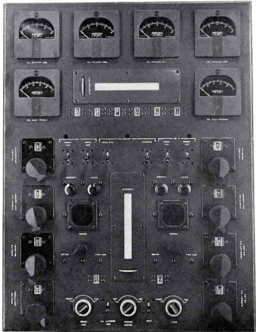
FIG. 6. Central control panel.
