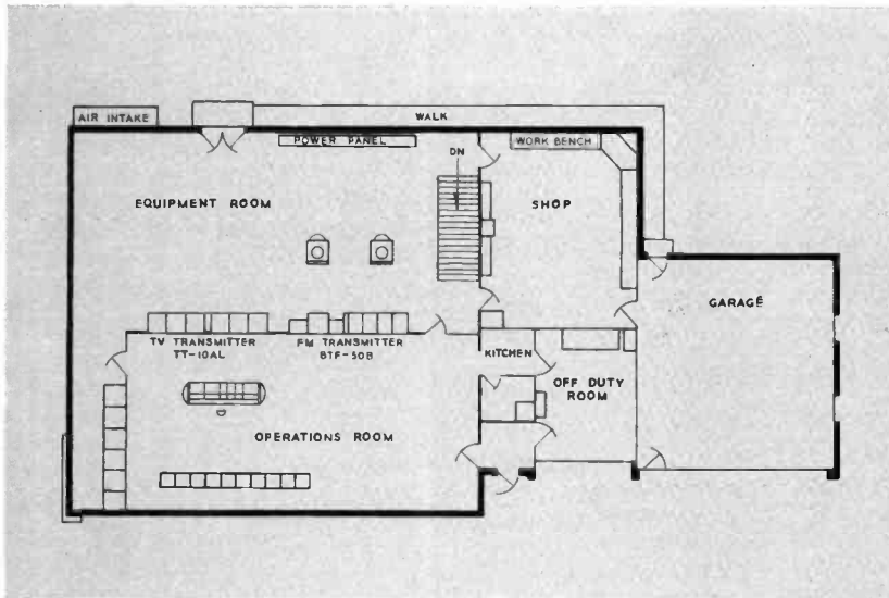
▲ FIG. 13. Floor plan of transmitter building, first floor. These spacious quarters house the TT-10AL television transmitter and BTF-50B FM transmitter. Ample shop space, an off-duty area and garage are included.
