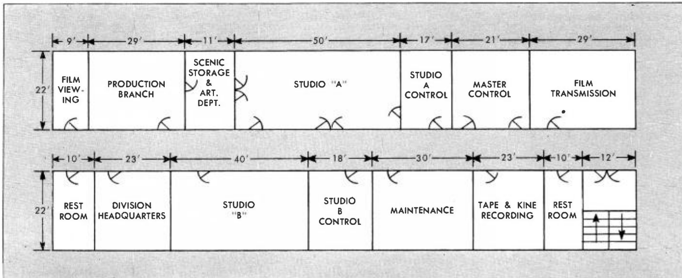
FIG. 21. Floor plan Ft. Monmouth Educational Television System.
