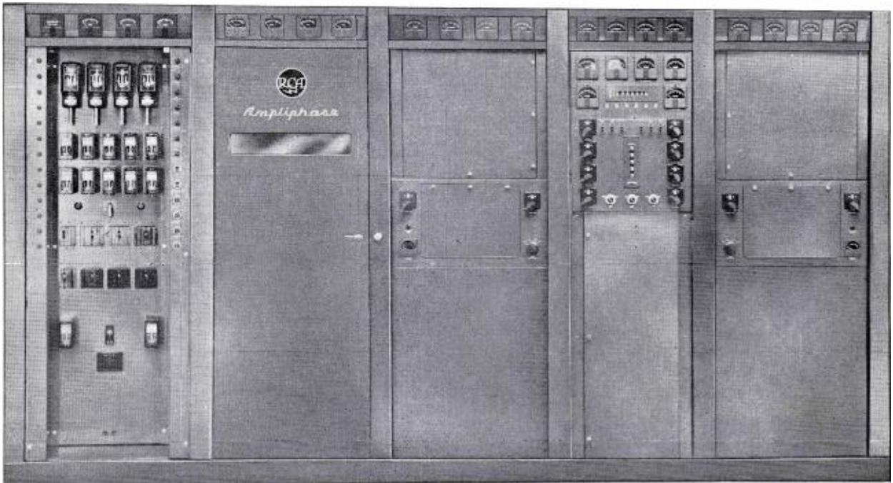
FIG. 1. Front view Type BHF-100A 100-kw Shortwave Transmitter.
