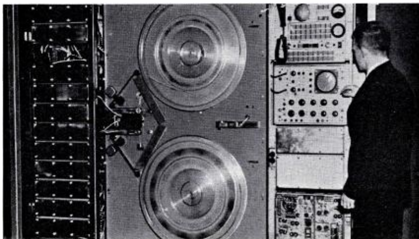
Thirty-inch reels of new recorder uses one mile of tape to reach top speed, another mile to brake down.
