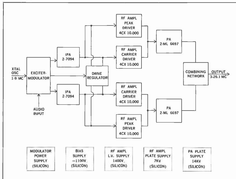
FIG. 4. Block diagram of 100-kw transmitter.
