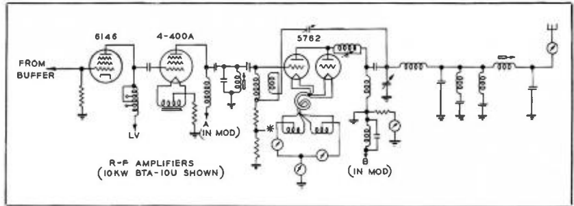
FIG. 6. Simplified schematic, r-f chain. Note the L/C circuits in the plate and cathode legs of the power amplifier. These are the high-efficiency resonators which boost plate efficiency to approximately 90 per cent.
