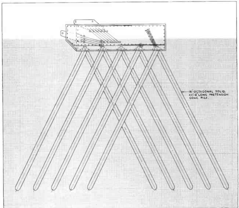
FIG. 7. Simplified drawing, guy-anchor pier elevation. Owing to the sea-level altitude of the site, piles—61 under the lower pier and a total of 136 under the guy-anchor piers—provide the firm base required. The ultimate settling of the structure, fully loaded, is determined to be less than one-tenth inch! ▼
