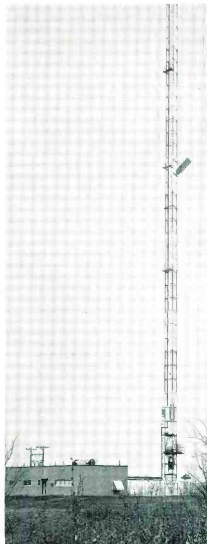
FIG. 22. Transmitter building and tower at Orion, 14 miles from studio. Type TW-15A Traveling Wave antenna covers the signal area.
