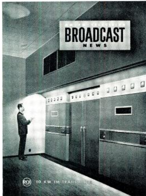
"A" SERIES of RCA FM Transmitters was introduced before the war, including the FM-1-A in 1939, the FM-3-A in 1940 and FM-10-A (10 KW) in 1941. Latter is shown above on the cover of our January 1944 issue. This transmitter was 18 feet wide, 84 inches high, required 54 square feet of floor space. The 10-E Transmitter, shown on the cover of this issue is 4 feet wide, 78 inches high, requires 13 square feet of floor space (less power supply).
