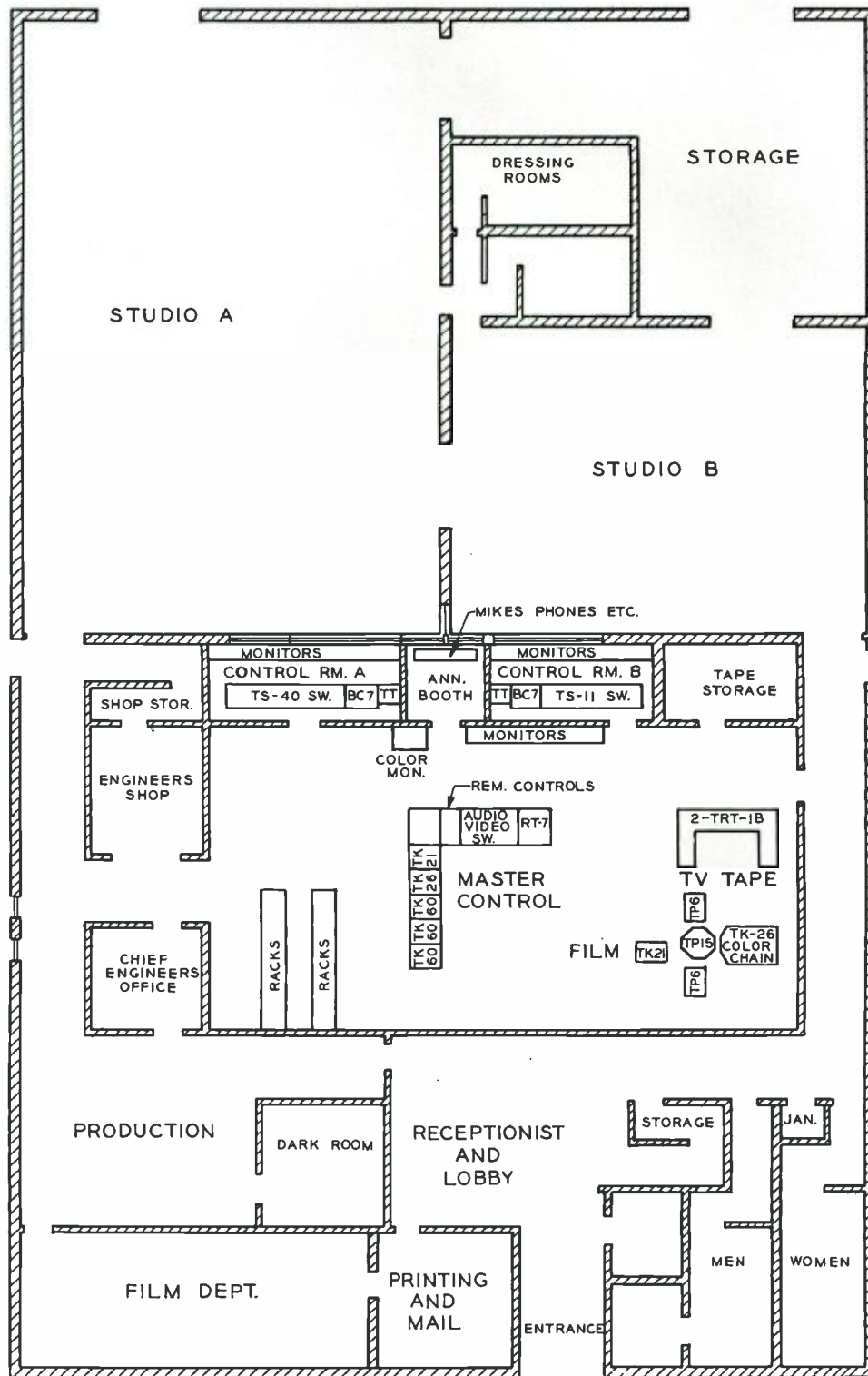
FIG. 20. Layout of first floor showing complete technical facilities for efficient production.
