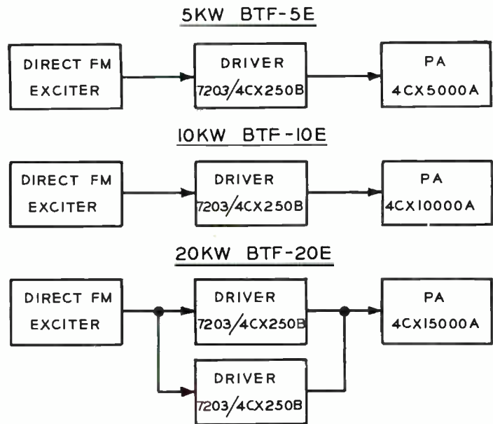
FIG. 3. Block diagrams show simplicity of three RCA FM transmitters.
