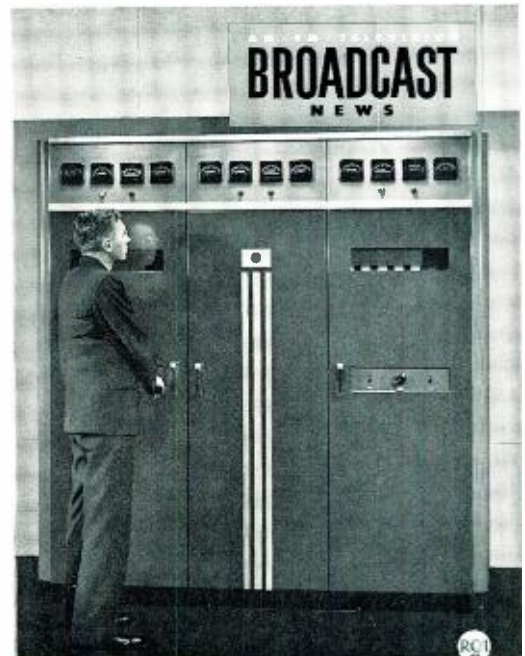
"B" SERIES of RCA FM Transmitters was introduced soon after the war. The RCA BIF-3B Transmitter is shown above on the cover of our January 1946 issue. These were the first transmitters of the new unit-design type. In the mid-fifties RCA introduced its C Series of FM Transmitters, and a few years later the D Series. The newly announced E Series is completely new inside and out but bears heavily on RCA's 25 years of experience in FM Transmitter design.
