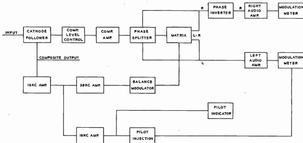
FIG. 2. BW-74 functional diagram. Receiving a demodulated signal, the monitor separates the left-and-right audio plus the pilot. See text.
