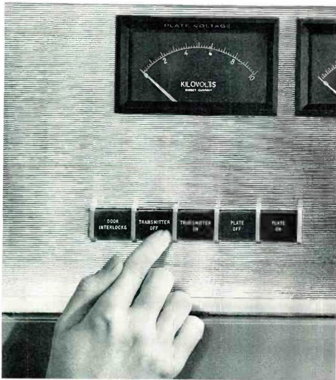
FIG. 4. Illuminated finger tip controls and tallies give instant circuit status.
