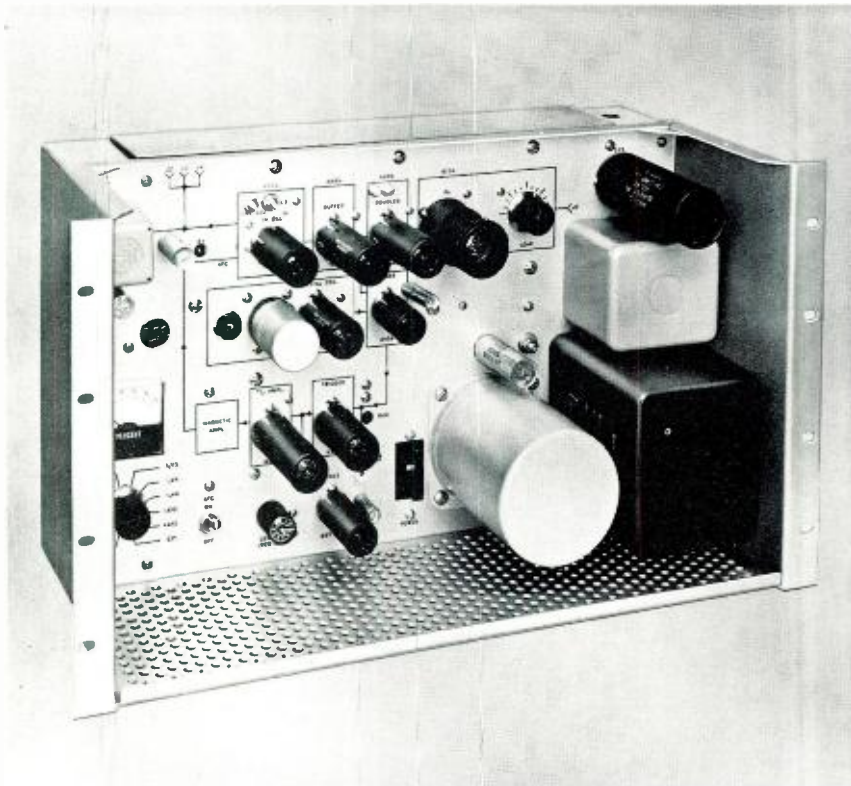
FIG. 10. Besides simplicity, BTE-10C FM Exciter features exceptionally wide temperature operating range. Power supply and test multimeter are built in.
