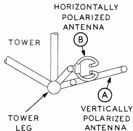
FIG. 4. Top view of the "best" arrangement recommended for a "H" and "V" array mounted on a tower leg. The presence of a guywire (not shown) requires the offset arrangement indicated here.
