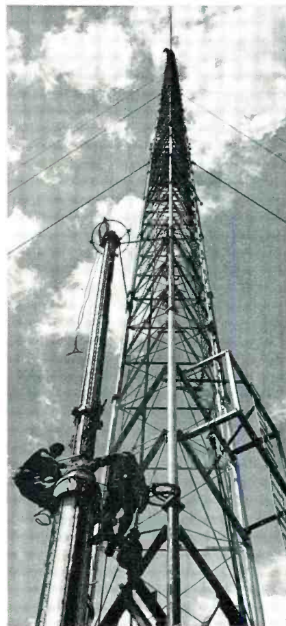
FIG. 6. The RCA Traveling Wave Antenna shown being hauled to top of tower.
