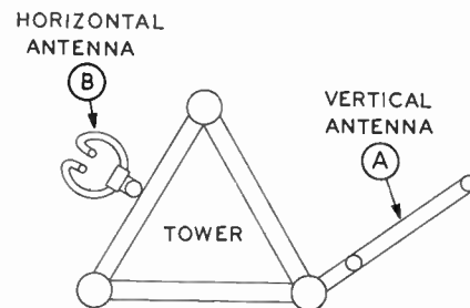
FIG. 5. A typical back-to-back arrangement when the existing "H" antenna is face-mounted on the tower. The rotation of the "V" antenna as shown here minimizes interference with the guy-wire system (not shown) of the tower.
