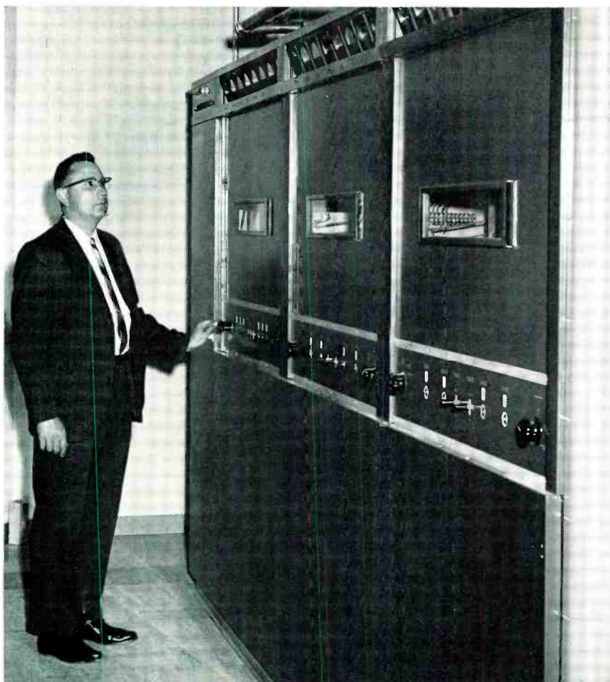
FIG. 21. Chief engineer, Ray Krueger at RCA TT-25DH 25-KW TV Transmitter. This unit is designed for color television and gives high quality monochrome performance.
