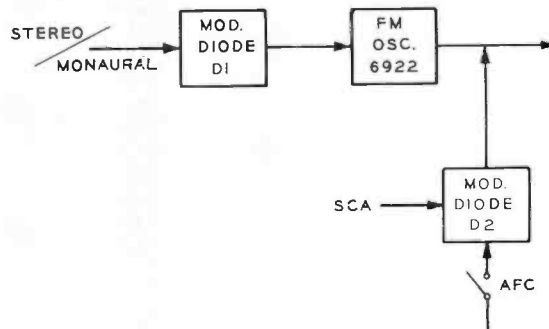
FIG. 14. Stereo/monaural and SCA programming are fed to independent diode modulators to provide utmost isolation between channels.
