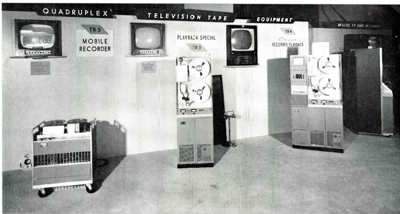
Three compact tv tape equipments . . . a TR-5 mobile recorder . . . a TR-3 playback machine . . . and a TR-4 economy recorder.
