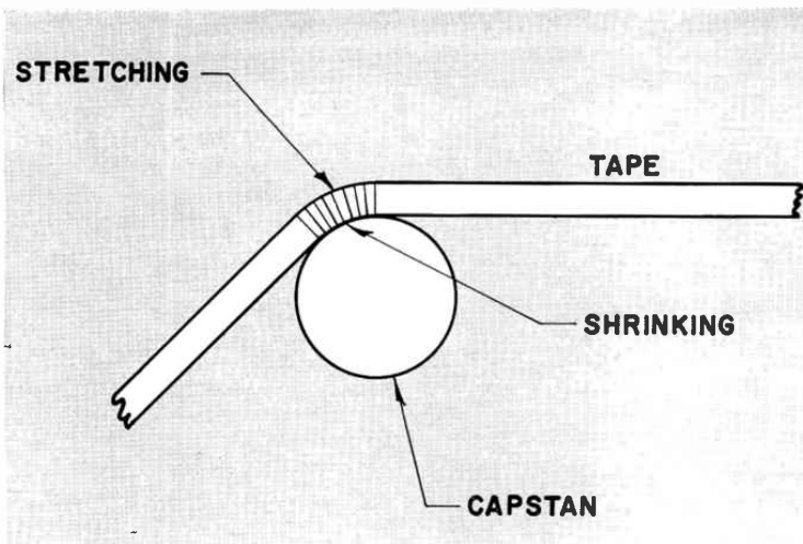
FIG. 2. Tape wrap around capstan showing stretching and shrinking.
