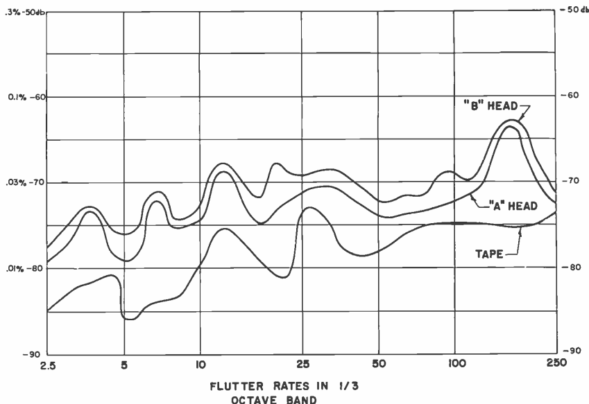
FIG. 4. Flutter content at various flutter rates.
