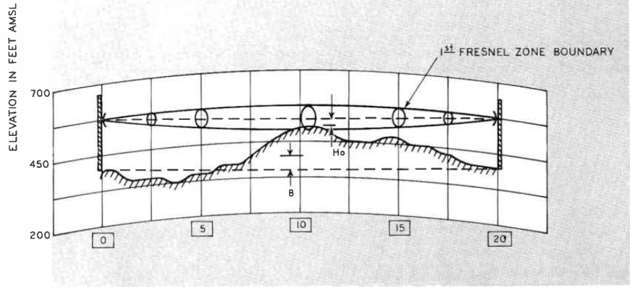
FIG. 2. A typical microwave path profile showing the first fresnel zone at 12 gc/s.
