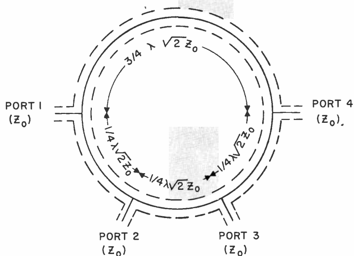
FIG. 7. Schematic diagram of power splitter.
