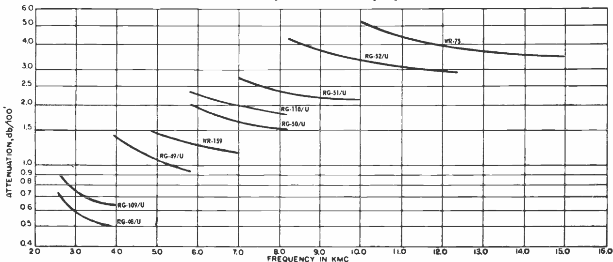
FIG. 7. Waveguide attenuation vs. frequency.
