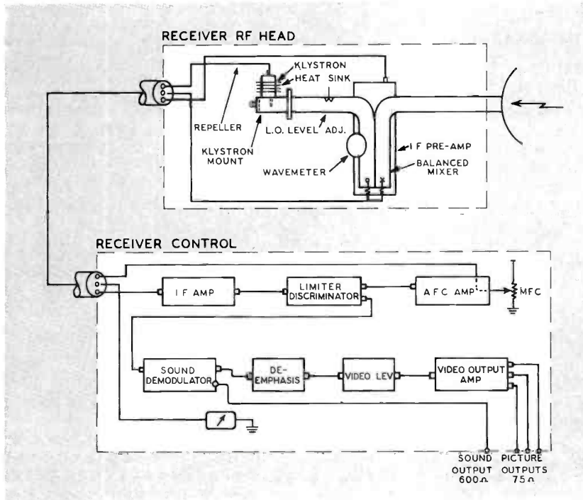
FIG. 12. Block diagram, TVM-3B receiver.
