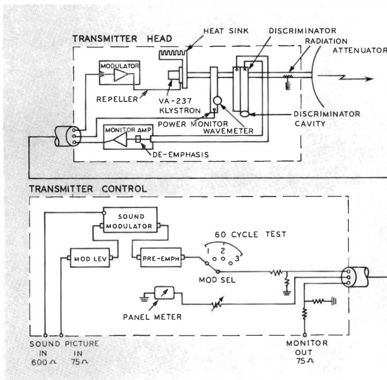
FIG. 9. Block diagram. TVM-3B transmitter.
