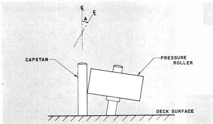
FIG. 7. Shaft misalignment normal to the tape plane.
