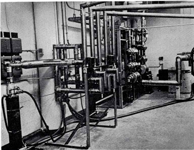
FIG. 12. View behind transmitters at WNAC-TV showing patch panels (center) which, in the event of failure of one transmitter, permit connection of operating transmitter directly to antenna. One of two water-cooled reject loads can be seen at extreme left (below diplexer). At right center is the filterplexer, feeding output line at extreme right.
