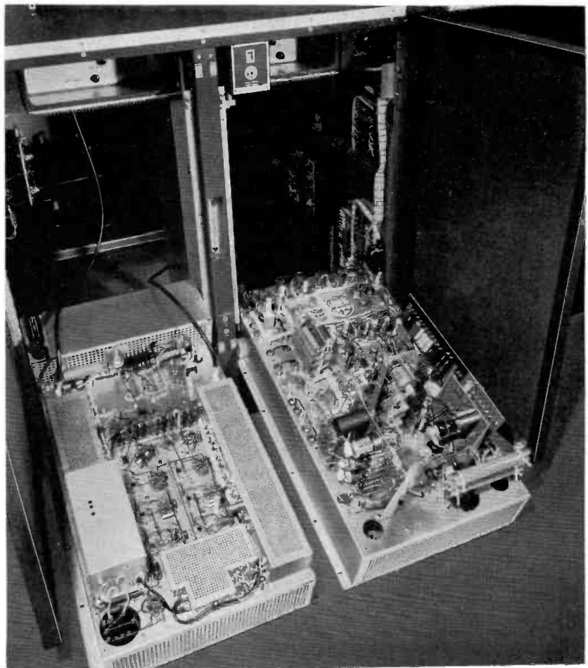
FIG. 6. Transmitter aural and visual exciter (left) and modulator are mounted on hinged chassis allowing the units to tilt forward for accessibility.
