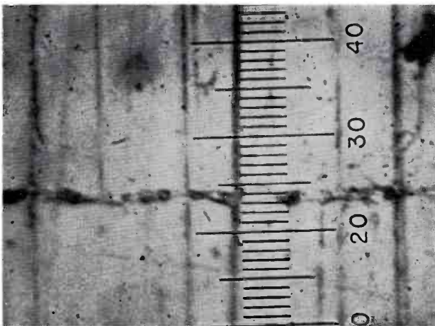
FIG. 12c. Gap Photomicrograph (gap smearing).
