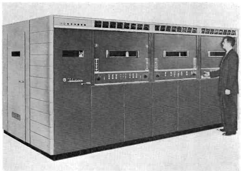
FIG. 2. RCA TT-25DH 25 KW transmitter of the type used in the WNAC-TV parallel transmitter installation. Two of these transmitters were recently ordered by KCRG for a similar parallel transmitter system in Cedar Rapids, Iowa.
