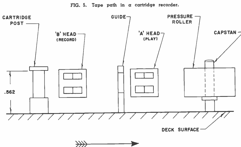
FIG. 5. Tape path in a cartridge recorder.
