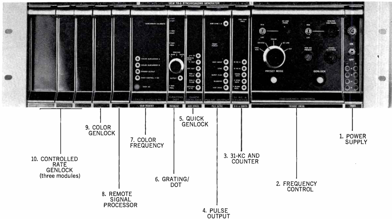
FIG. 1. TG-3 Sync Generator with all modules in place.
