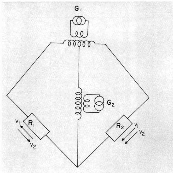
FIG. 9. Simplified schematic diagram of diplexer system.
