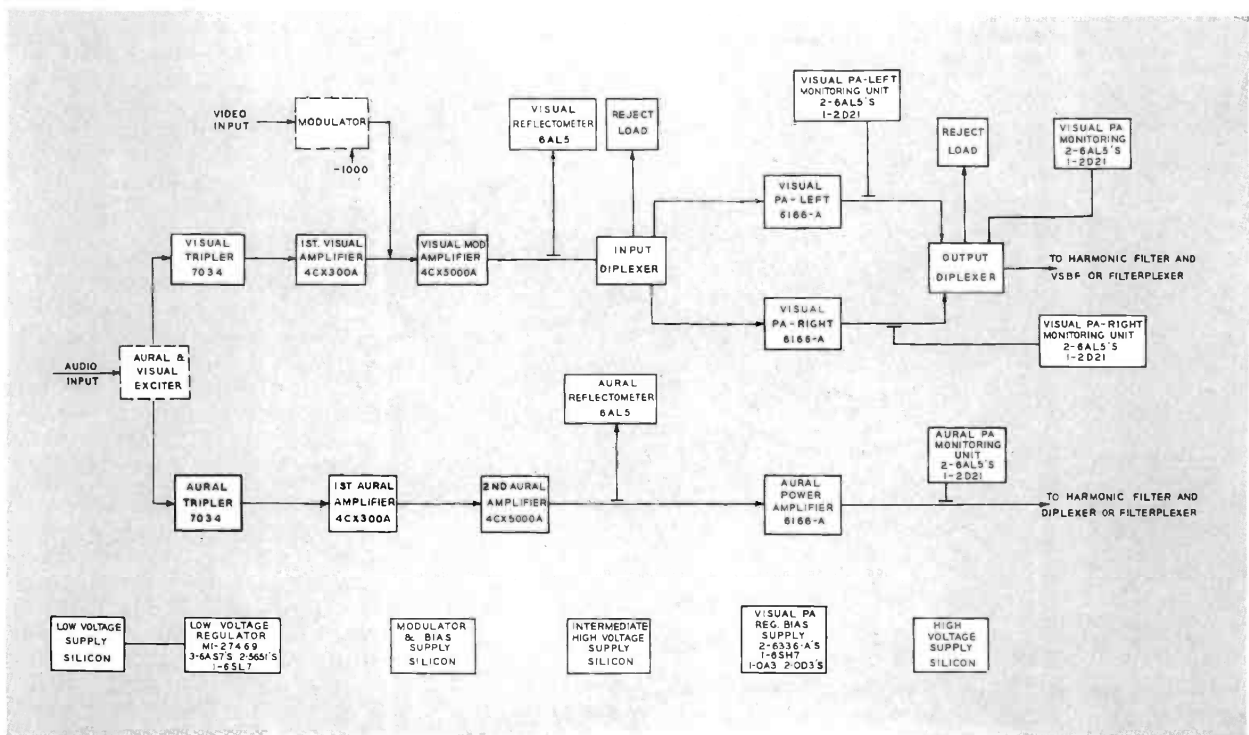
FIG. 5. Simplified block diagram of one TT-25DH 25 KW Transmitter.
