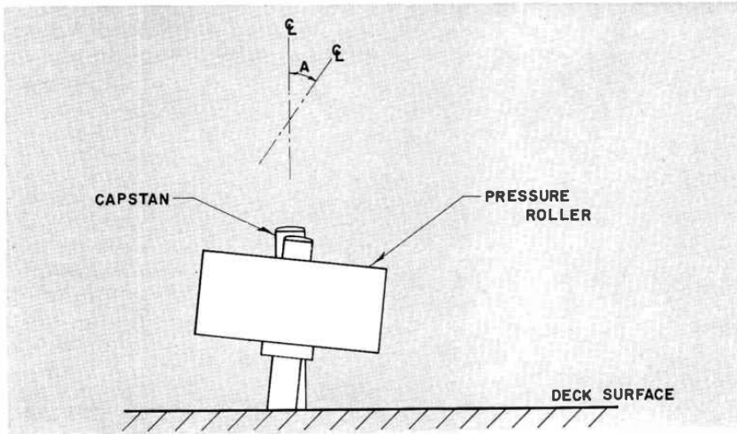
FIG. 6. Shaft misalignment in the tape plane.
