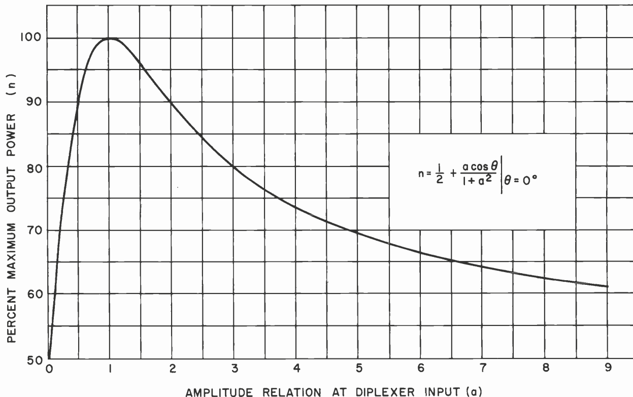
FIG. 10. Curve showing diplexer output for various ratios in amplitudes of input signals.
