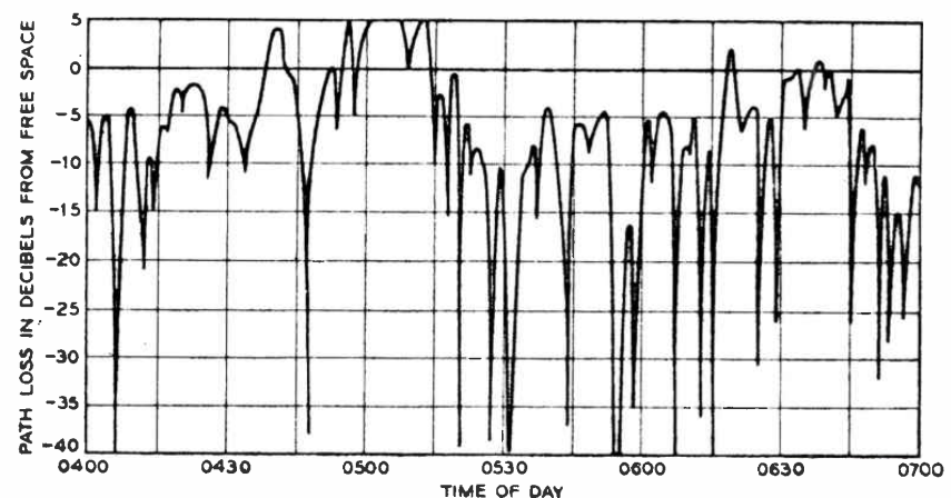
FIG. 8b. Typical multipath fading at 11 gc/s.
