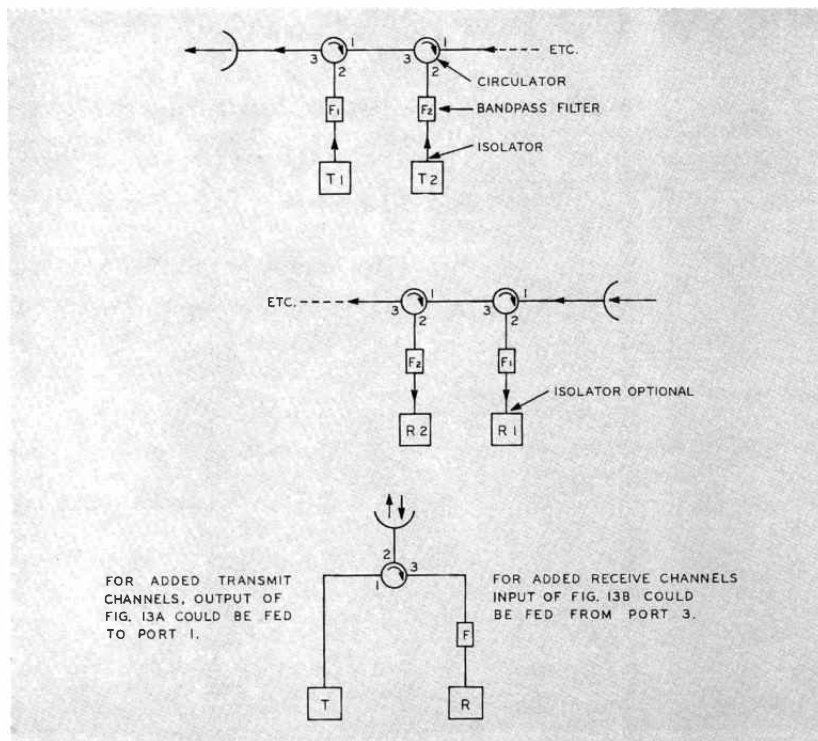
FIG. 13. A. (top) Transmitter multiplexing on common antenna. B. (center) Receiver multiplexing on common antenna. C. (bottom) Antenna diplexing for two-way transmission.
