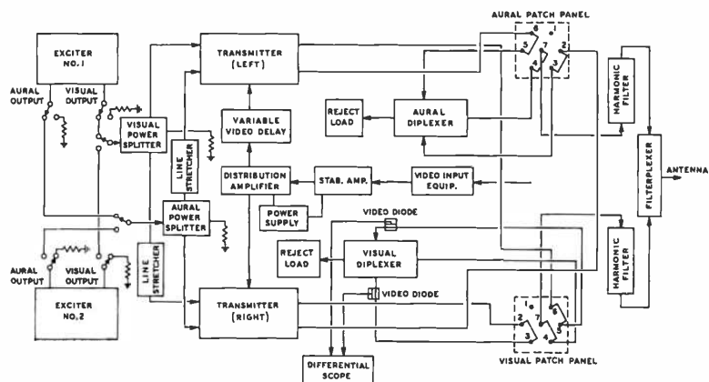
FIG. 4. Simplified block diagram of WNAC-TV parallel transmitter system.
