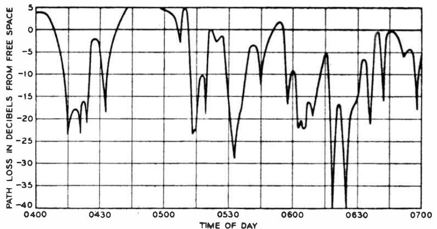
FIG. 8a. Typical multipath fading at 4 gc/s.
