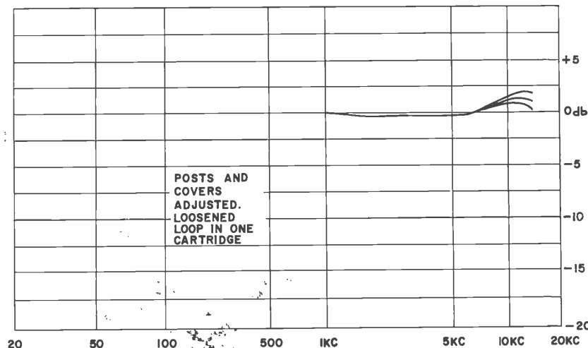
FIG. 11. Frequency response after adjusting posts, covers and loops.
