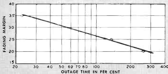
FIG. 6C. Added precipitation outage expected with fade margins less than 40 db.
