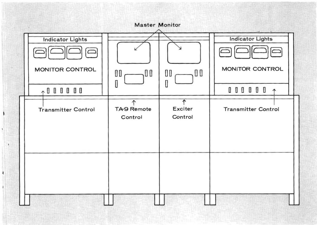
FIG. 13. Diagram showing WNAC-TV transmitter control console equipment for parallel transmitter operation.
