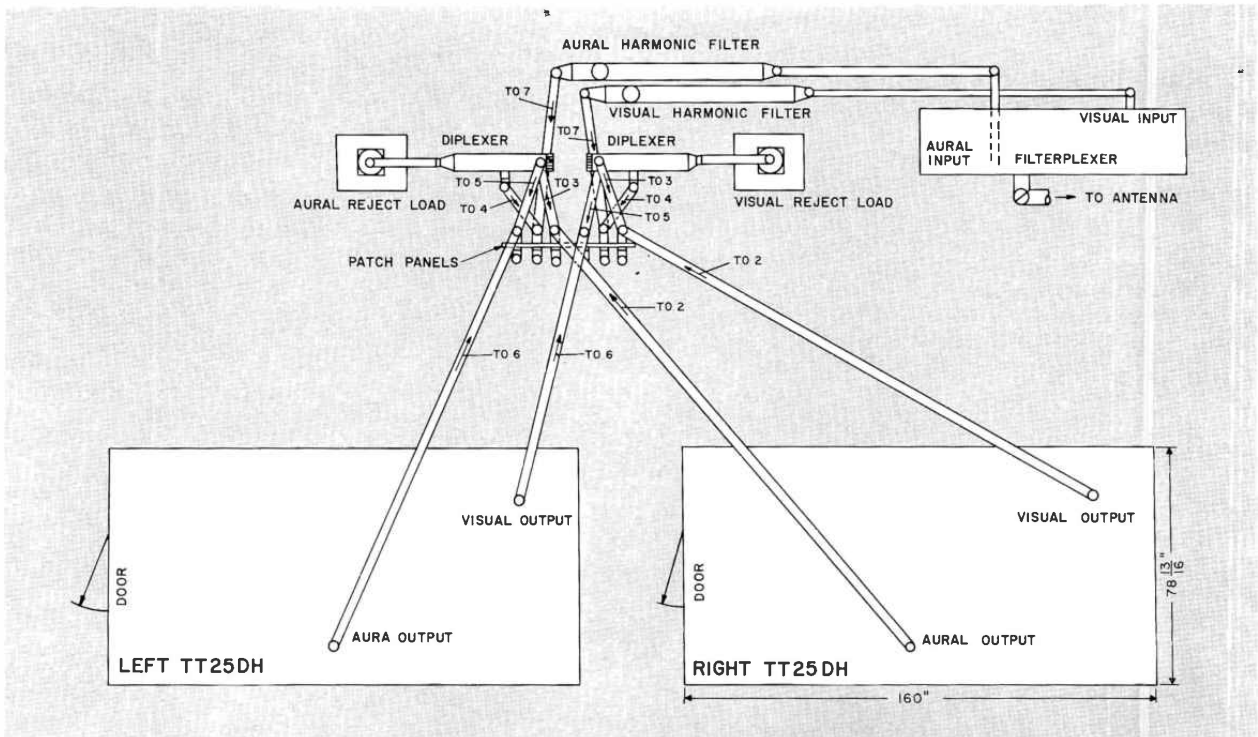
FIG. 3. Floor plan, showing parallel transmitter equipment layout at WNAC-TV.
