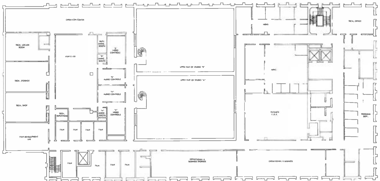
FIG. 11. Fourth-floor plan — new KRON-TV Building.
