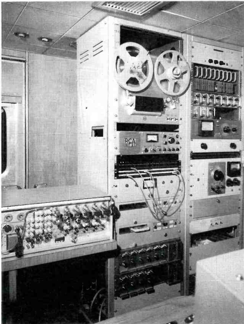
FIG. 11. The main audio racks: illustrating RT-21 reel-to-reel tape, and two cartridge tape units (1 record and replay, and 1 replay only.)
