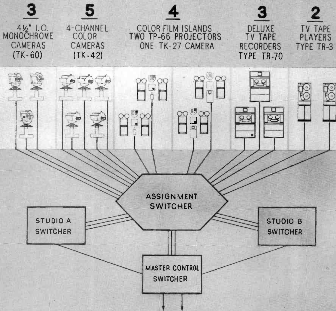
FIG. 17. A simplified Block diagram of the equipment being installed in the new KRON-TV Building.
