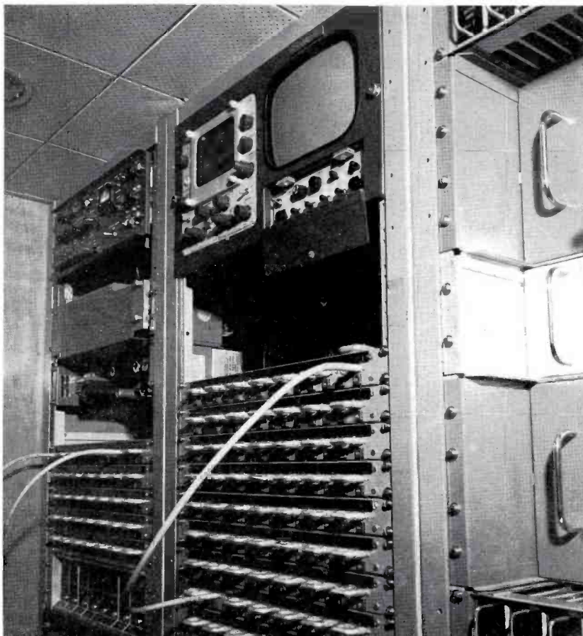
FIG. 9. Near the maintenance area and behind the camera controller, are the equipment racks housing the video switching modules, power supplies, video patch bays, video test equipment, VHF tuners, and microwave equipment.
