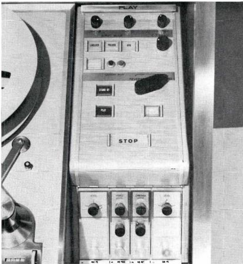
FIG. 5. Output/Playback controls are positioned at right of tape deck and Control Center, separating them from the recording function. A special feature here in the TR-70 is the choice of three servo modes: Linelock, Pixlock, NPC. These serve to give selection of conditions for finest color tape reproductions possible — whether mixing is required, fast recovery from disturbances (see text) or replay of heterodyne process tapes. Another new feature is the CT Phase Control. In one position it serves as optimizing control (when correct track has been selected for playback.) In second position, all four tracks are covered to seek the correct track. Another exclusive feature of the TR-70 is the continuously variable speed wind control.
