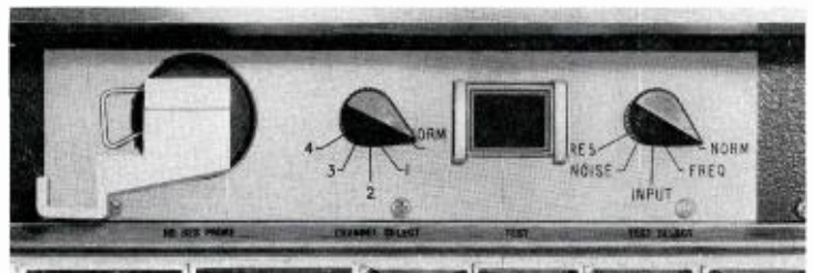
FIG. 8. FM test facility incorporated in TR-70 employs signal from built-in module to optimize the headwheel. This assists operator in set up, making measurements, and matching. It assists production of tapes without annoying disturbances. Automatic safety feature disconnects test mode if operator inadvertently selects another mode.
