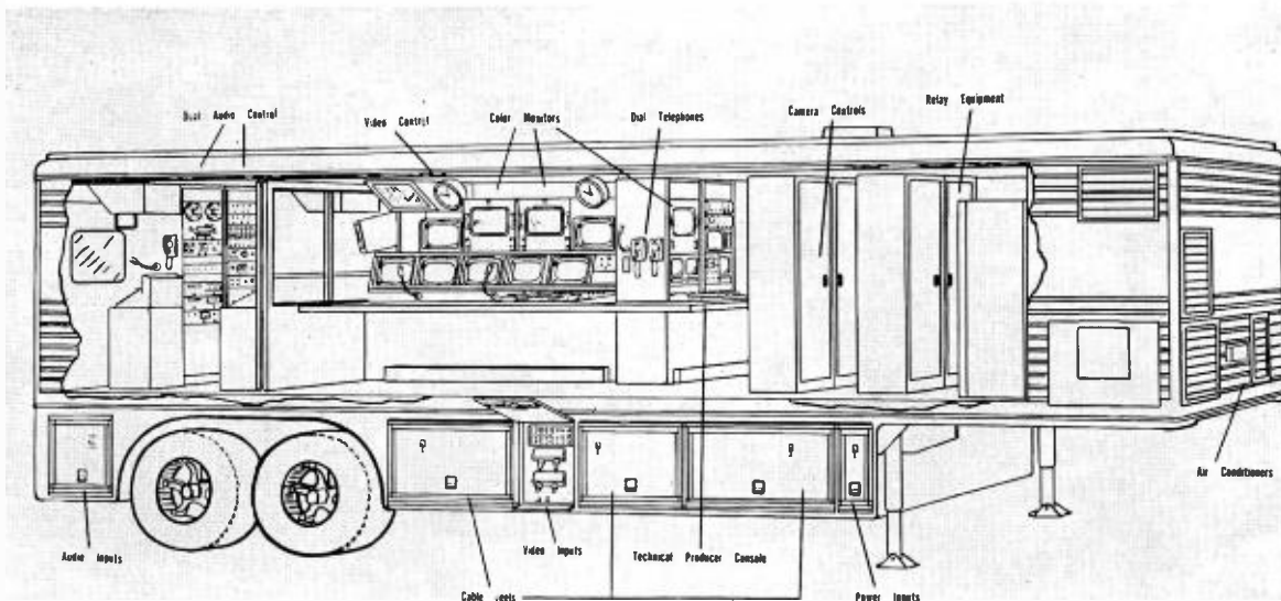
FIG. 4. Cutaway drawing of CBC Color Mobile Van showing audio and video production facilities.
