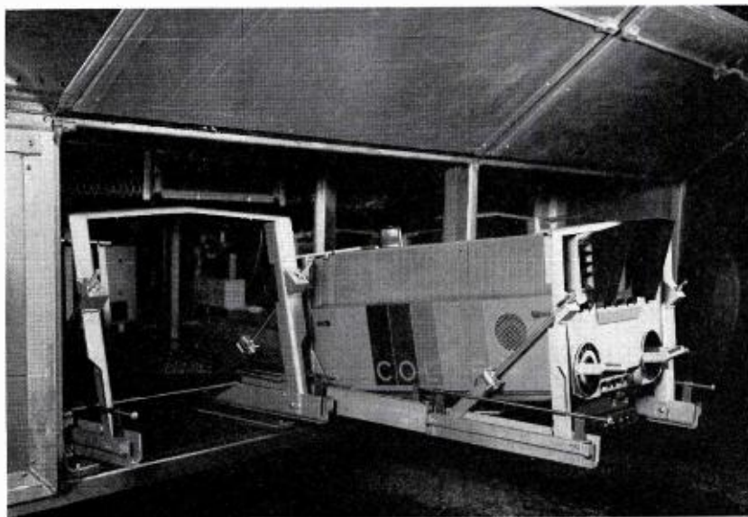
FIG. 5. One of four TK-42 cameras secured to the roll out undercarriage camera tray. Above the camera is the main cable duct.
