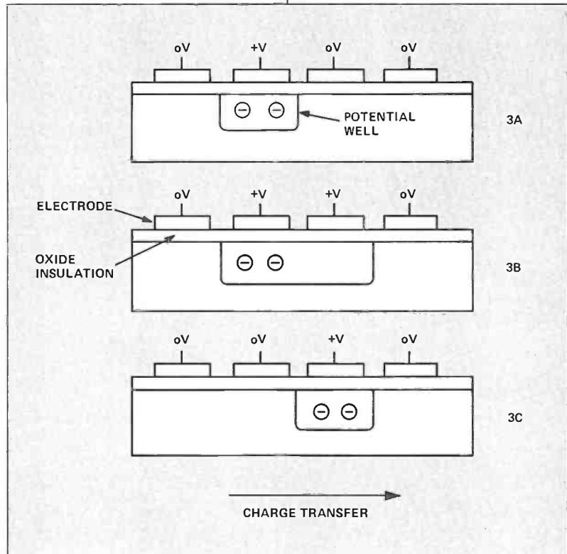
Fig. 3A, 3B, 3C (Right): simplified graphic displays of how charge transfer works in a charge coupled device.
