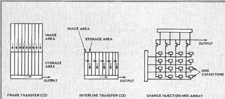
Fig. 1. Four basic approaches to CCD Sensors.
