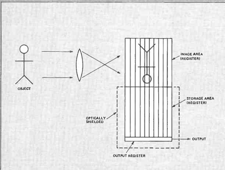
Fig. 2. Frame Transfer CCD.
