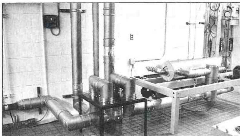
Motorized coaxial switchers are mounted overhead (above) while manual patch panel is floor mounted next to Notch Diplexer (below).
