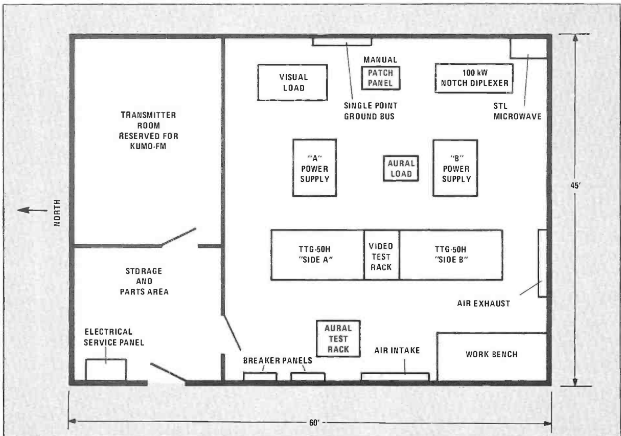
Transmitter Building Floor Plan.
