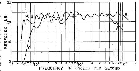
Fig. 5—Experimentally determined response characteristics.
