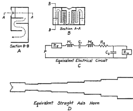
Fig. 1—Combination horn and direct radiator loud speaker. A. Vertical cross-sectional view. B. Horizontal cross-sectional view of the top portion. C. Equivalent electrical circuit of the acoustical system. D. Equivalent straight axis horn.
