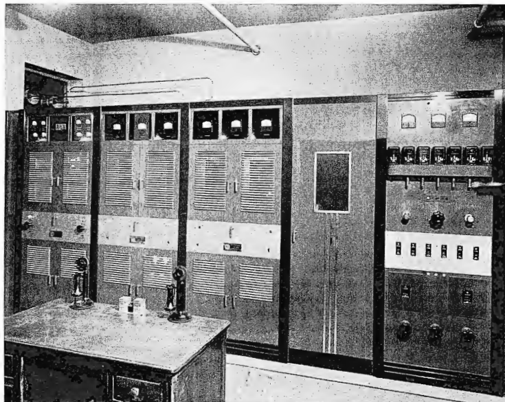
The RCA 5-D transmitter, first air-cooled installation made.
