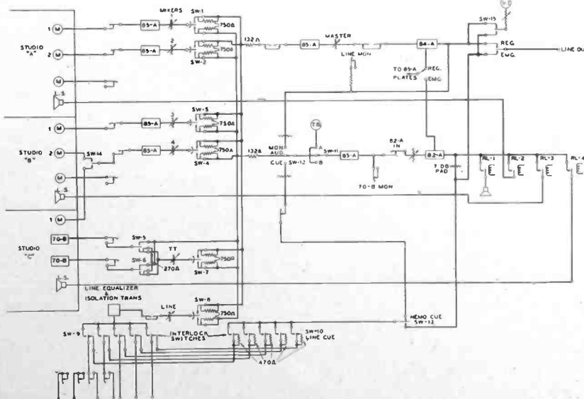
Block diagram of the 80-A.
