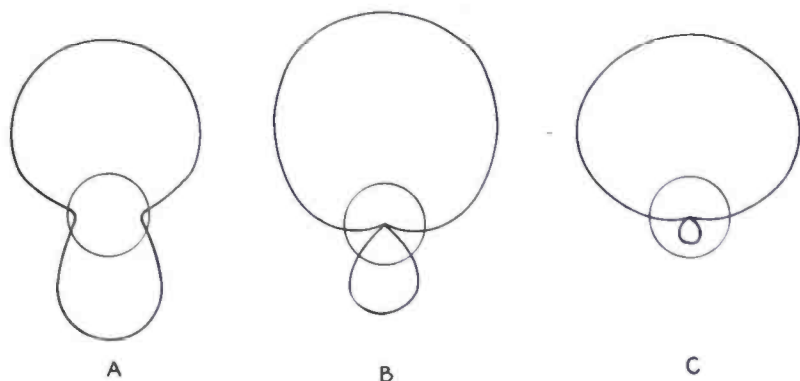
Fig. 40—A. d/\lambda = + 0.1 X_{00} = + 10.3 ohms X_{11} = + 25.0 ohms B. d/\lambda = 0.05
