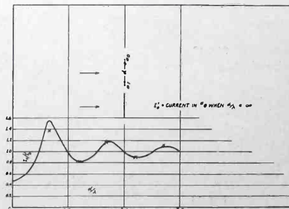
Fig. 31 Two receiving antennas in broadside
