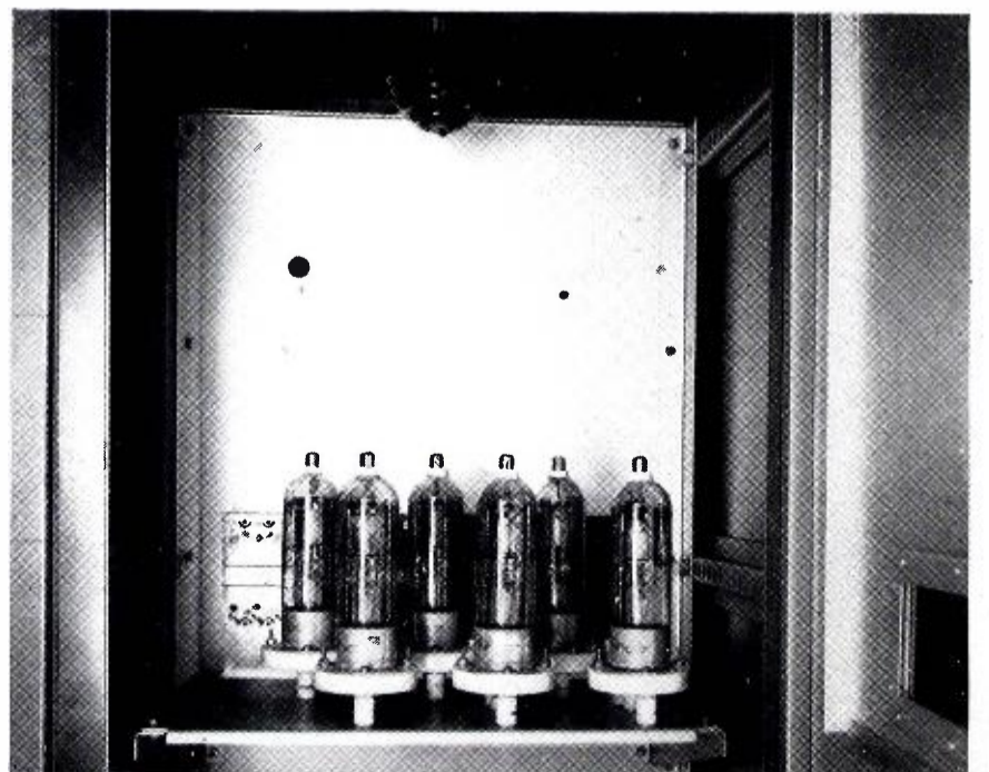
RCA-8008 Rectifier tubes are used in 3 KW and higher powered transmitters.
