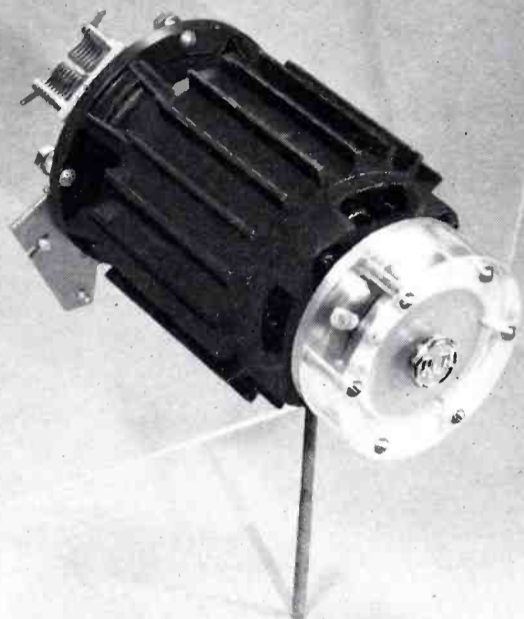
FIG. 8. Front and rear views of the two-phase motor with the frequency-determining capacitor mounted directly on the motor shaft. On the front end of the shaft (enclosed in the Lucite case) is an oil dampening unit which prevents overshooting.
