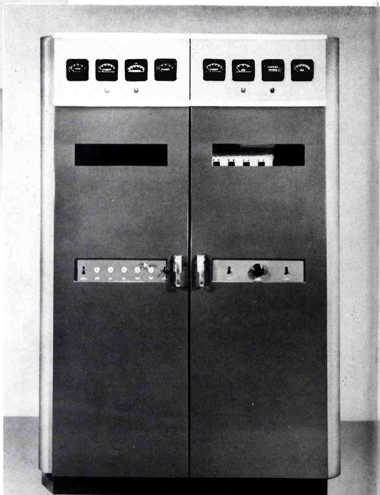
(Right)—The new RCA Type BTF-1C Transmitter for 1000-Watt FM station. For specifications, dimensions, etc., see Page 20.
