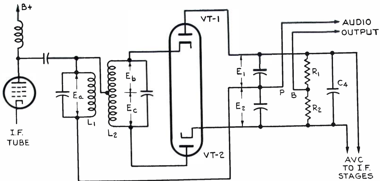
FIG. 2. Ratio Detector.
