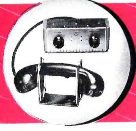
10. Mobile Handset and Control Unit: Furnished with the FM Mobile transmitters shown above. The two units can be conveniently mounted on the dash in any desired position. Control includes "volume" and "squelch." Signal lights indicate "transmit" and "stand-by."
