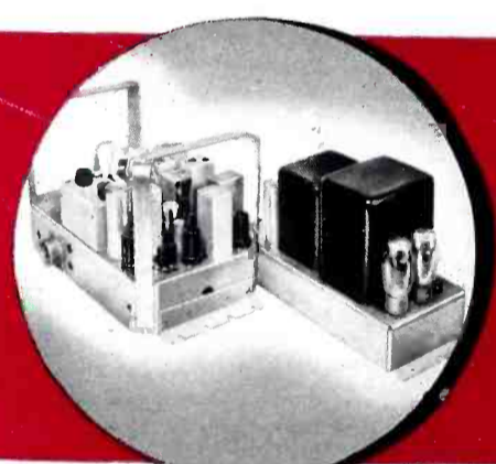
7. 60-Watt FM Station Transmitter: Uses same chassis as #5, but is furnished with chassis brackets for rack-mounting. A.C. power supply is a separate chassis unit. Not furnished for shelf-mounting.
