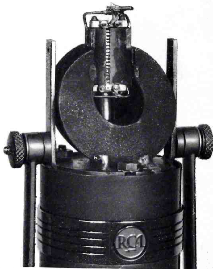
FIG. 3. Front interior view showing ribbon construction.
