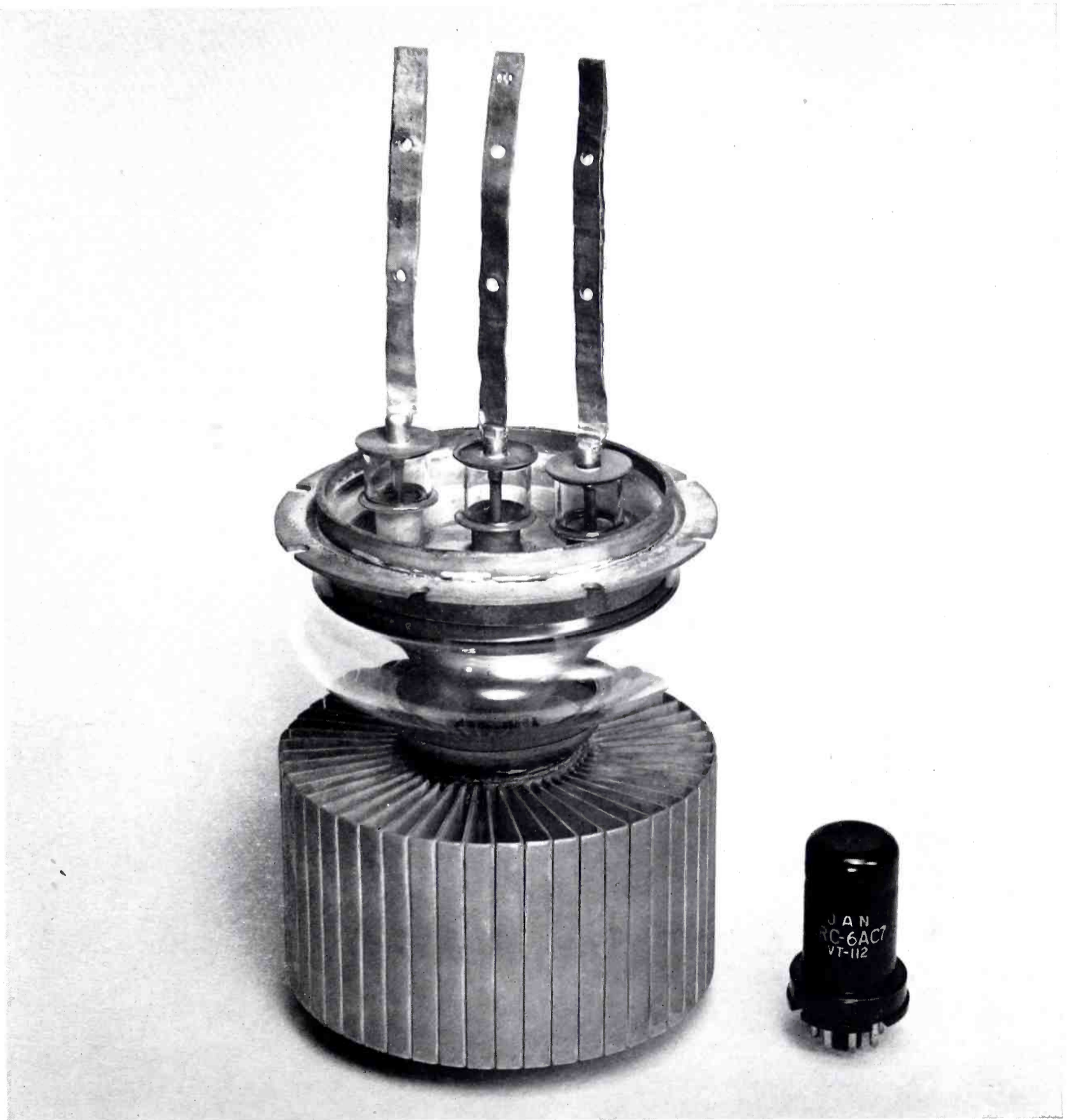
The new RCA 7C24, a tube especially designed for Grounded-Grid operation (reproduced approximately full size).
