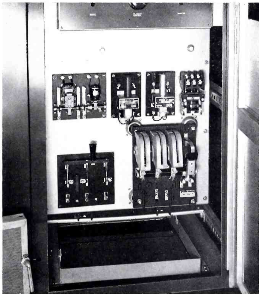
The dust filters mount on top of the base frame. Air is drawn in through openings in the rear of the base frame (or may be supplied by a floor duct).
