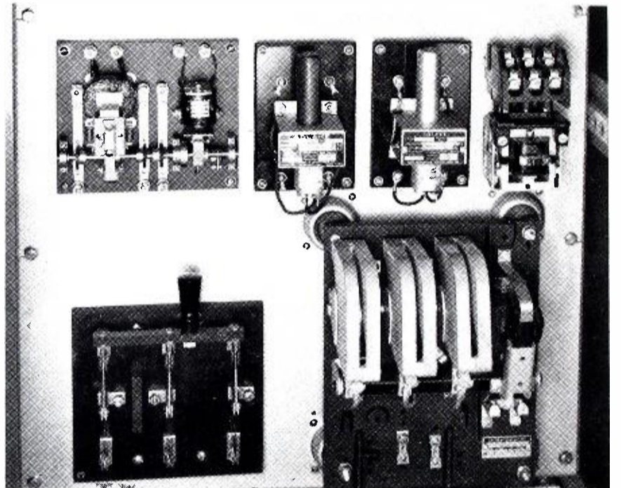
Automatic starting and recycling relays and power reduction switch.
