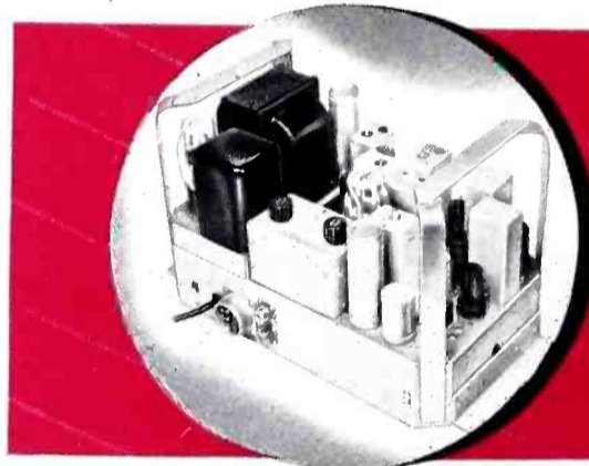
6. 30-Watt FM Station Transmitter: Uses same chassis unit as #4. Can be furnished with dust cover (as shown in #4) for shelf-mounting, or with brackets for mounting in standard RCA cabinet-rack, such as shown in #8.
