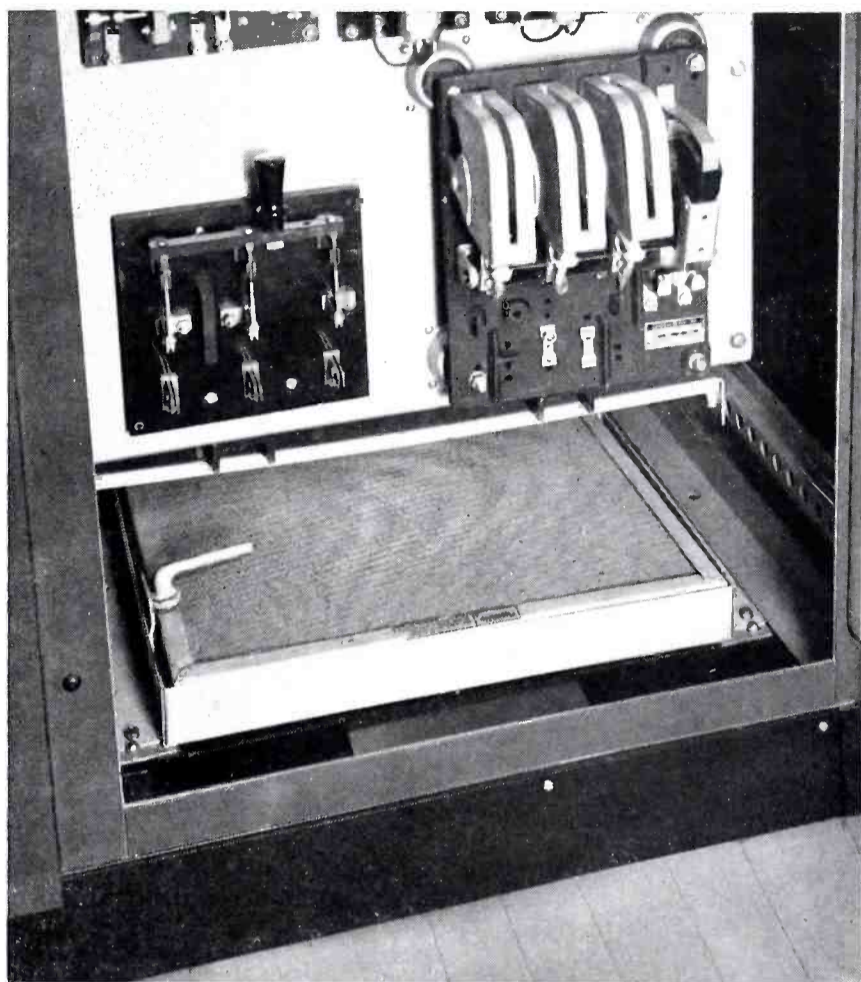
A spun-glass dust filter is located in the base of each unit. A wiring duct (the openings are visible in this view) is located just in front of the filters.
