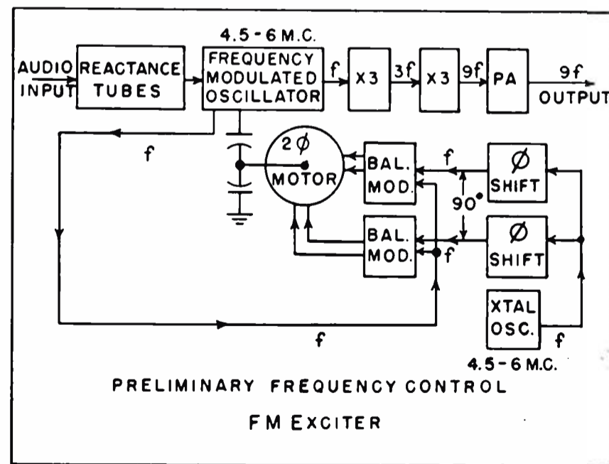
FIG. 7. Block diagram of the preliminary form of the new exciter unit. In this arrangement the crystal-controlled oscillator operates in the 4.5 to 6.0 megacycle band, thus permitting direct comparison with modulated oscillator frequency.
