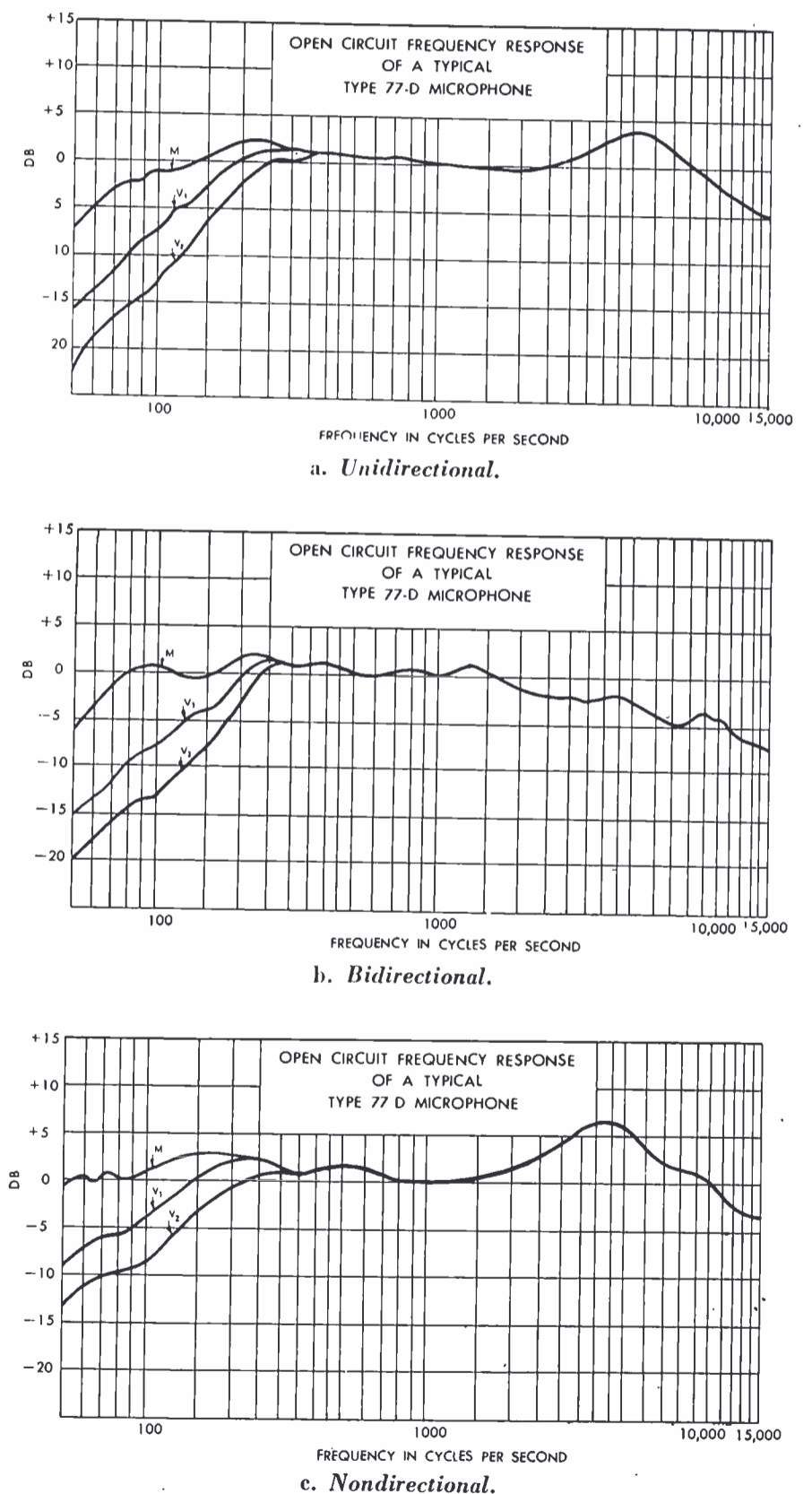
FIG. 10. Frequency response characteristics Type 77-D Microphone.
