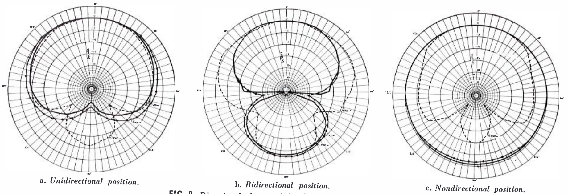
FIG. 9. Directional characteristics Type 77-D Microphone.
