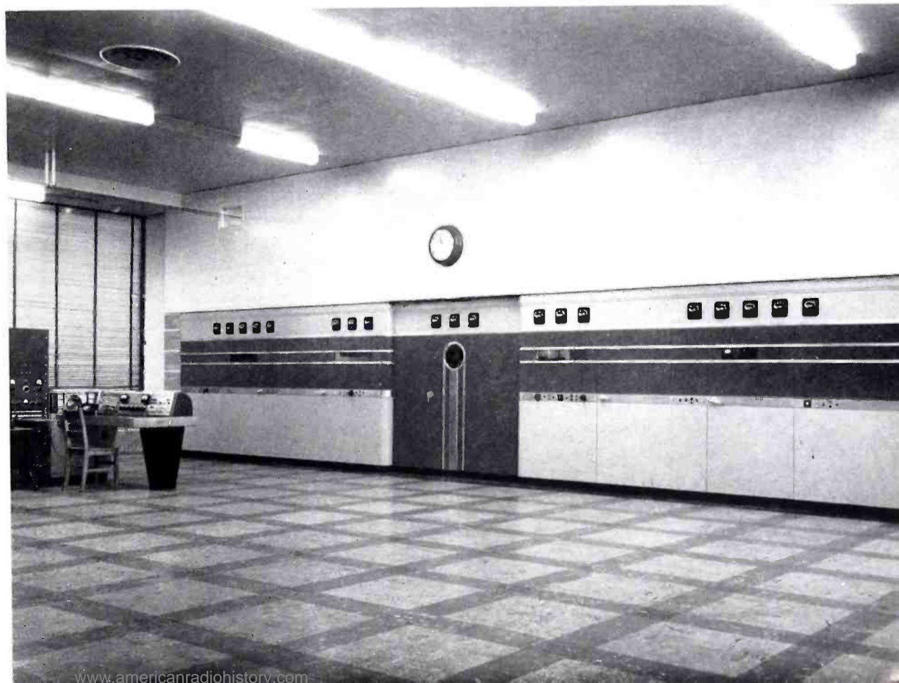
FIG. 6. Front view of RCA Type 50-SW #2 with control console and audio rack at left.
