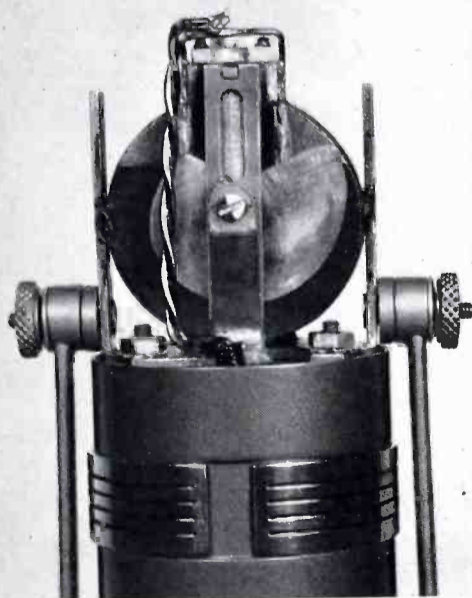
FIG. 5. Rear internal view—aperture wide open.
