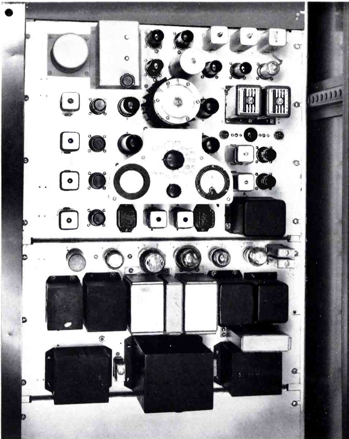
FIG. 1. Front view of the new-type exciter unit used in all of the new RCA FM Transmitters. Other photos of this unit are shown on pages 11 and 14.
