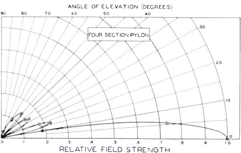
FIG. 9. Vertical field patterns in free space. (FULL length slots, frequency 88 megacycles.) Note how wasteful skywave radiation is reduced by stacking Pylons.
