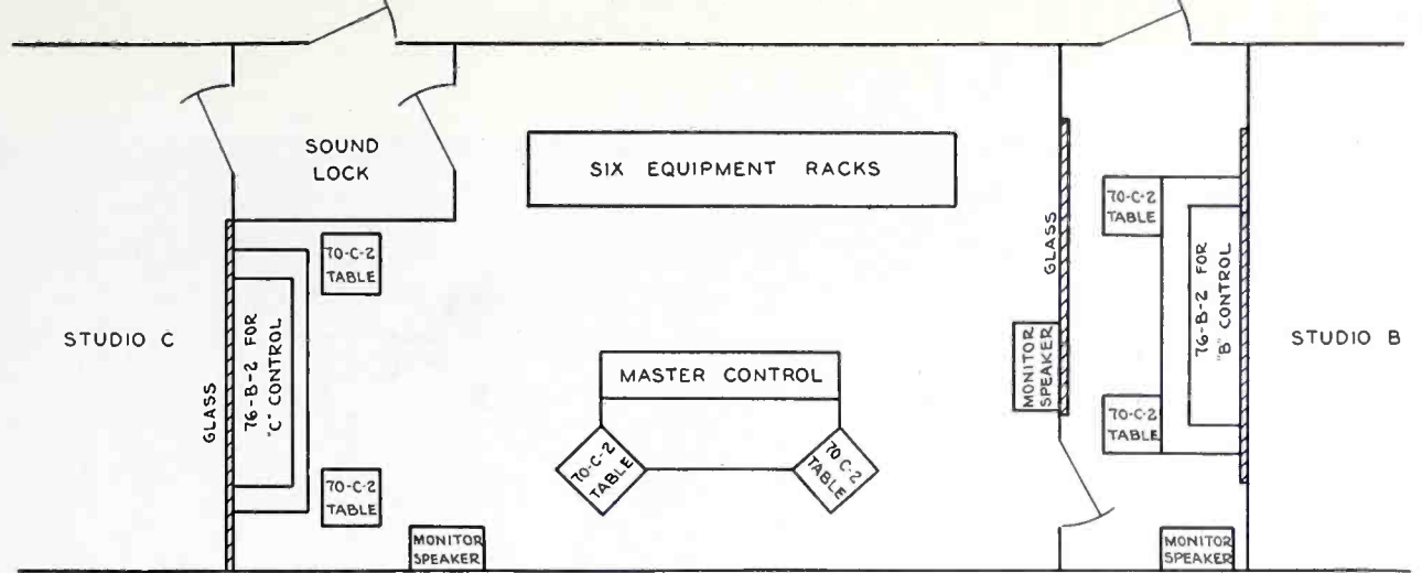
FIG. 2 Floor layout of the WBAL master control room and Studio B control room.
