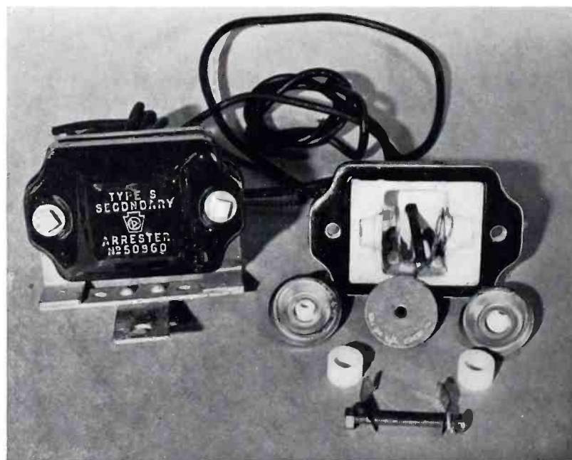
FIG. 11. This photo shows how the lightning discharge affected the arrester which was added to the beacon lighting circuit at the top of the Pylon. Note the scarring or pitting of the three lightning arrester plates. This did not impair the operation of the arrester.
