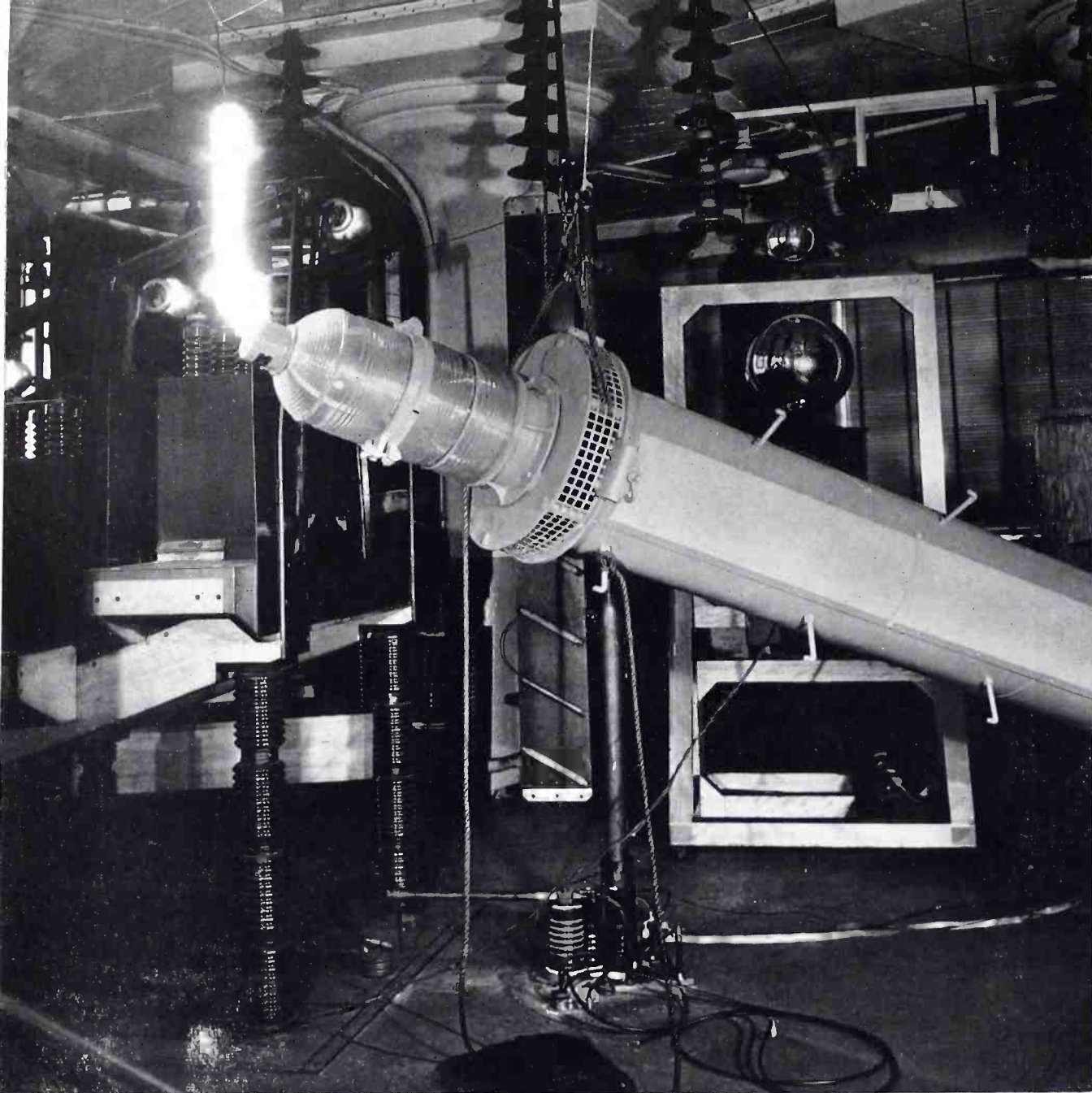
FIG. 1. (left) Pylon antenna being subjected to a 500,000 volt discharge in the high voltage testing laboratory.
