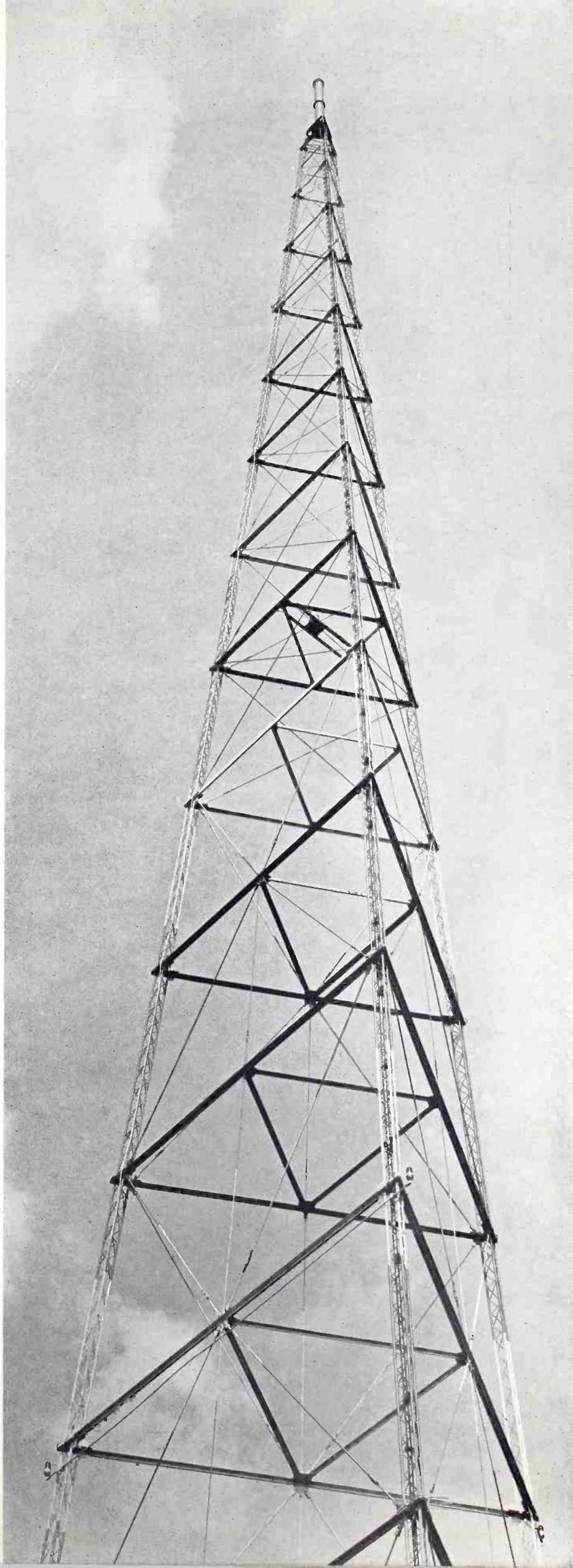
FIG. 8. (right) This is how the WSBA tower appears with the two-section pylon mounted in place. Tower and pylon have a total height of 404 feet.
