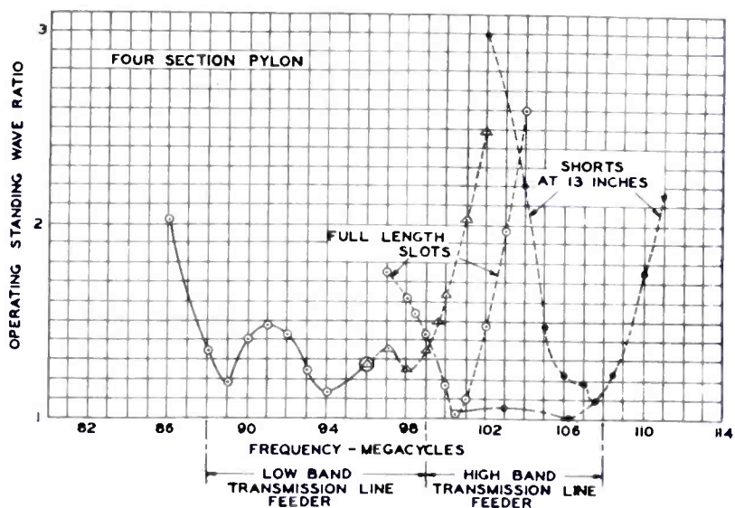
FIG. 4. The curves above show typical operating standing wave ratios for the one-, two-, and four-section Pylon.
