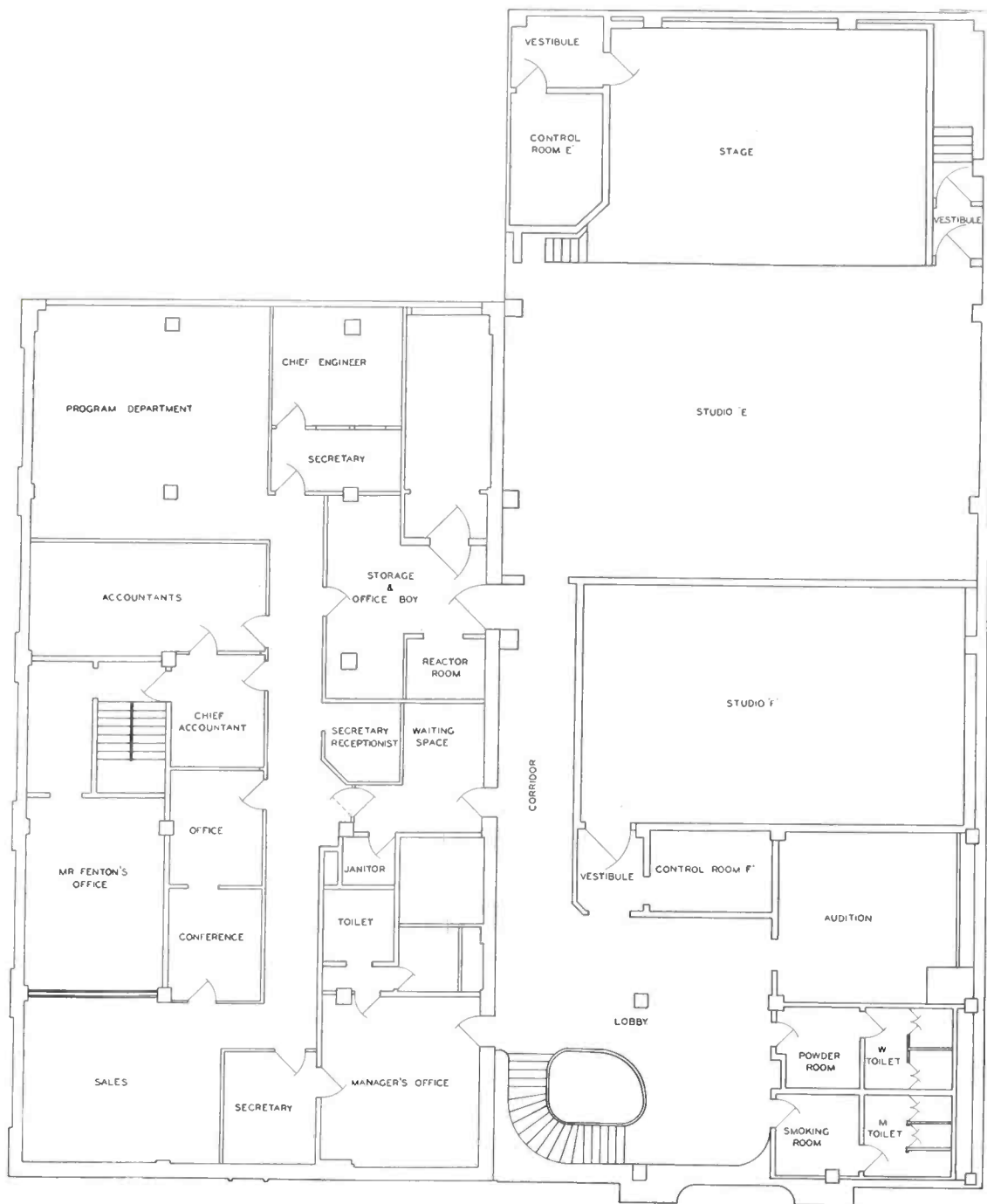
FIG. 4. (left) Arrangement of the second floor of WBAL's new installation. The "Air Theatre" and "Futuristic" studio are on this floor, as well as most of the station offices. Entry to this floor is by means of a wide circle stairway at the front of the building. The lobby is large and luxuriously furnished.
