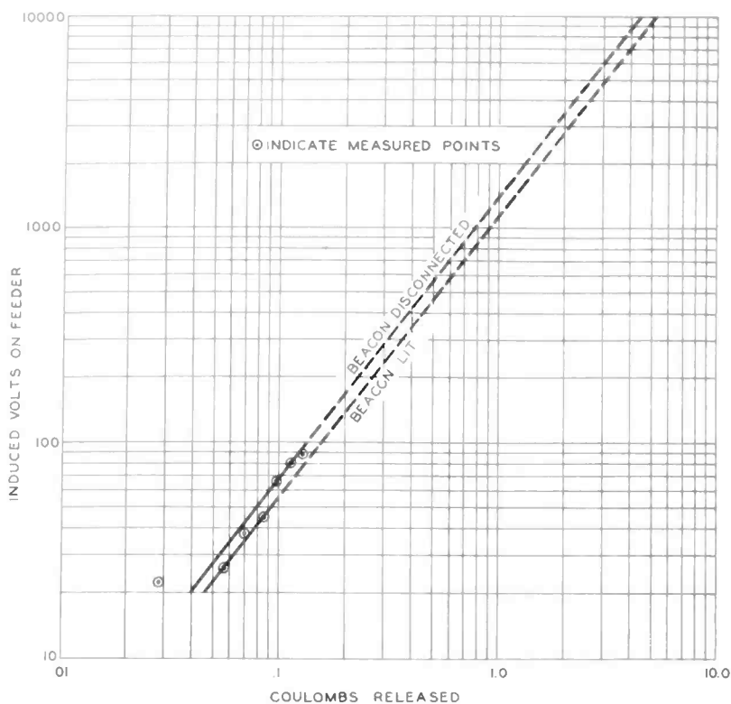
FIG. 8. Curves showing how the induced voltage on the Pylon feeder varies with changes in the charge released in coulombs.
