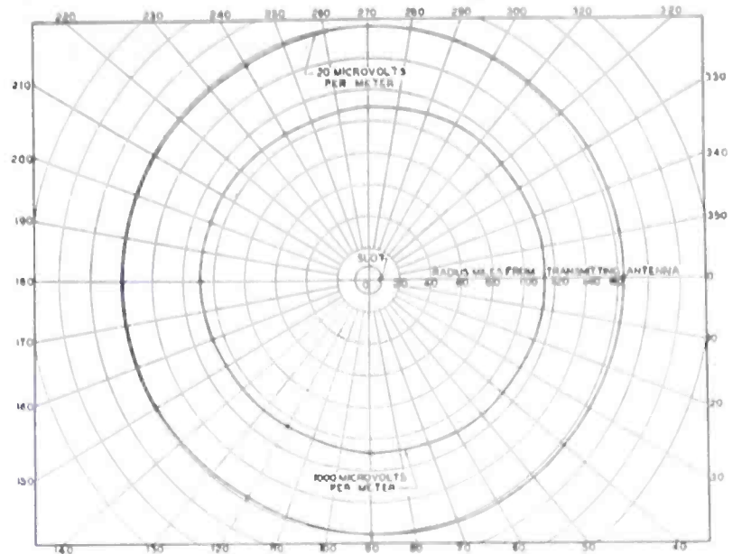
FIG. 7. Typical 50 kw FM transmitter coverage with an eight-section Pylon. (Frequency, 98 megacycles; antenna height, 5000 feet; Receiving Antenna height, 30 feet.) Note primary rural service radius of 160 miles.
