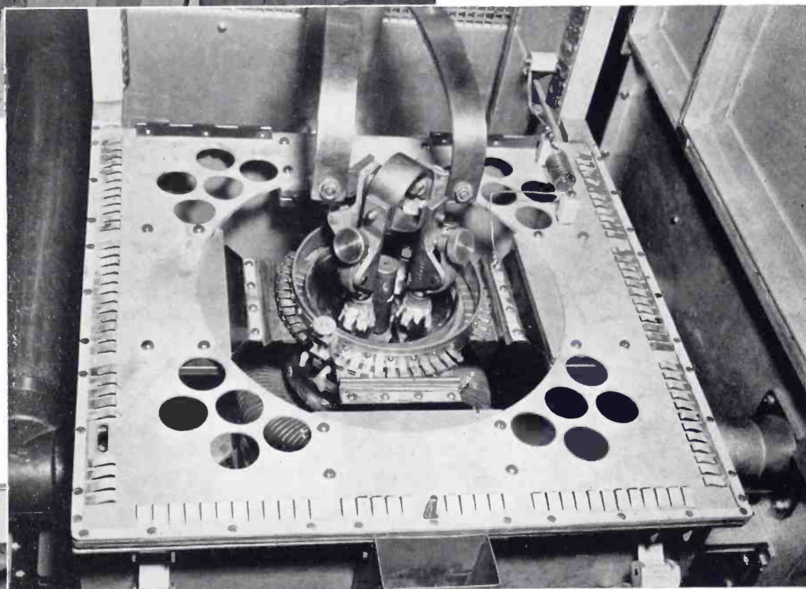
FIG. 6. (right) This is a closeup view of the grid shield in place. The RCA-5592, especially designed for use in grounded-grid circuits, has a grid construction which provides complete internal shielding. The external grid connection is of the disc-seal type. The grid shield shown here extends the internal shielding so that no neutralizing is required. Operation is extremely stable at all FM frequencies.
