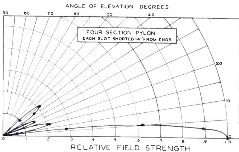
FIG. 10. Vertical Field Patterns in free space. (Slots shorted at optimum positions—frequency, 108 megacycles.)
