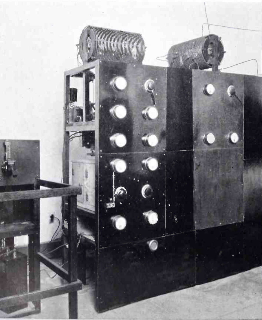
1928 The 5000-watt composite transmitter shown below was built by station engineers in 1928. It made WWL one of the high-power stations of that day.
