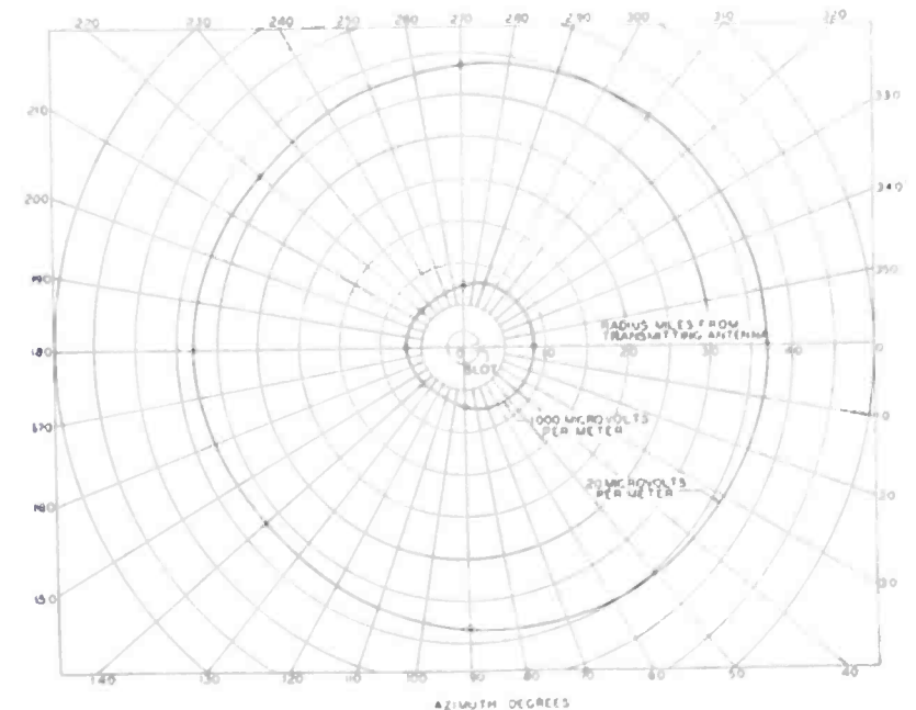
FIG. 8. Typical 250 watt FM transmitter coverage with a single-section Pylon. (Frequency, 98 megacycles; antenna height, 100 feet; Receiving Antenna height, 30 feet.)
