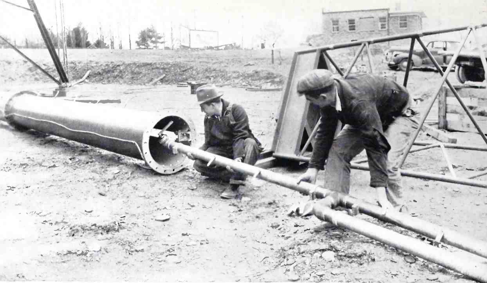
FIG. 5. In this view the two workmen are installing the transmission line harness inside the metal pylon cylinders. With the pylon antenna only one transmission line connection must be made "in the air."
