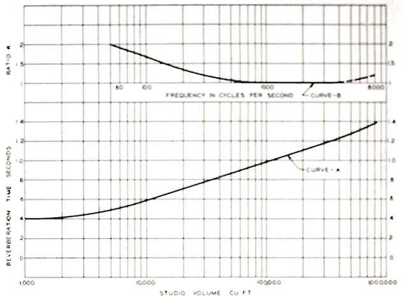
FIG. 16. Optimum reverberation time and frequency characteristics.
