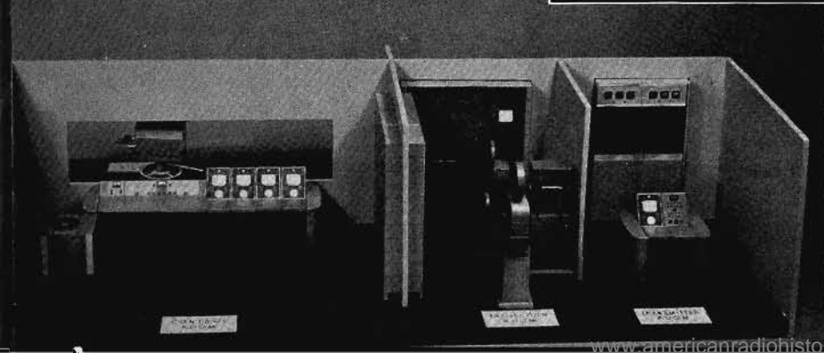
FIG. 13 (left). This model setup simulates a smaller station consisting of a combined studio and master control room, a projection room, and a transmitter room containing a model of the RCA 500-Watt TV Transmitter.
