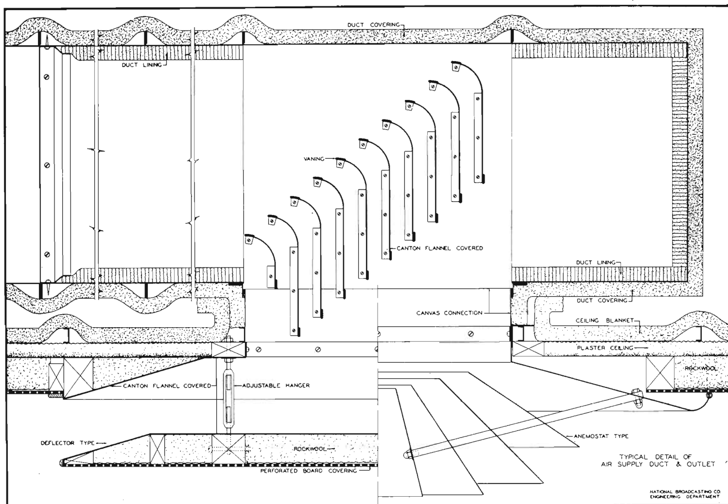
FIG. 10. Mechanical detail of an air supply outlet of deflector or "Anemostat" type.
