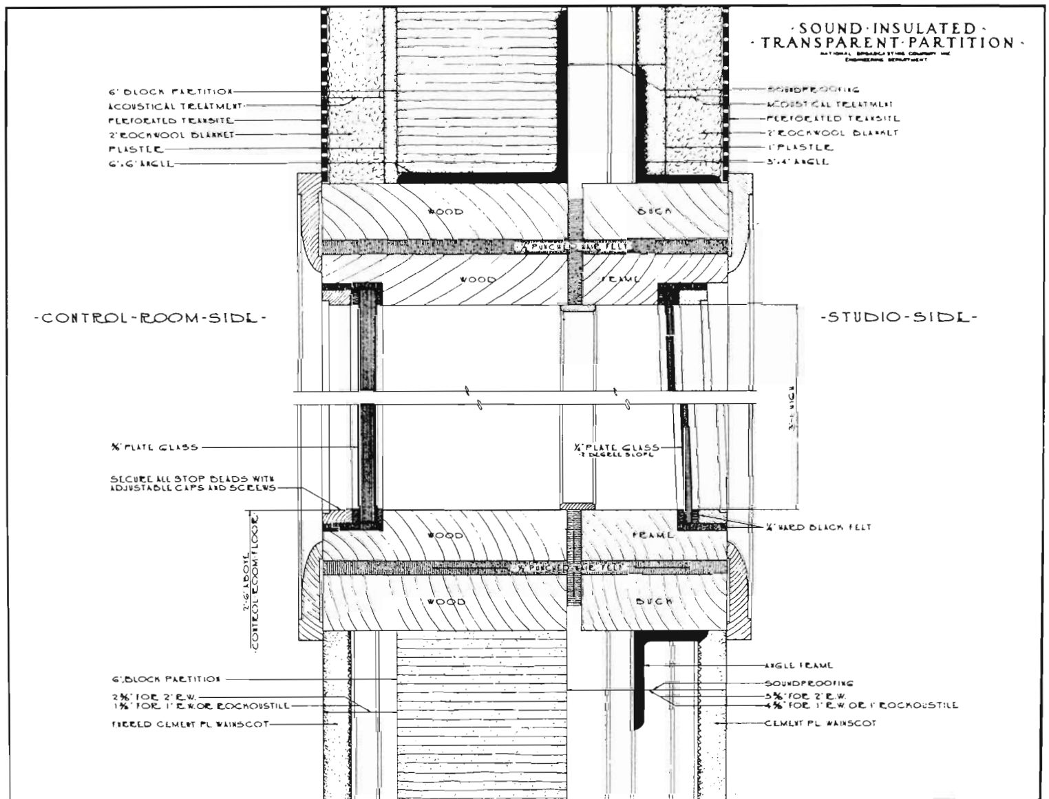
FIG. 9. Details of a sound insulated transparent partition.
