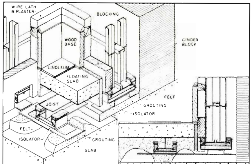
FIG. 6. Typical acoustic treatment for a floor to isolate sound from below.
