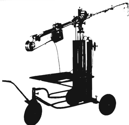
FIG. 4. Microphone Boom and Perambulator. This boom enables the audio man in the studio to pickup the sound while keeping the microphone out of the view of the camera.
