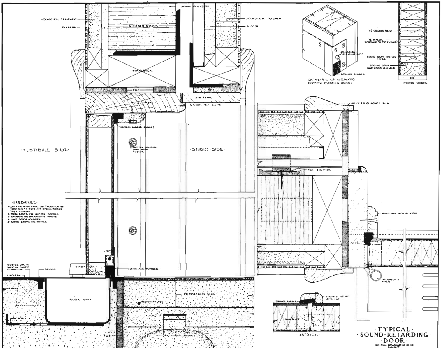
FIG. 8. Construction details of sound retarding studio door.
