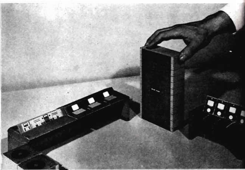
FIG. 9. Initial use of the models may be in the planning of individual rooms. Equipment for a studio control room is shown below in one of several arrangement possible with RCA "unit-built" equipment.
