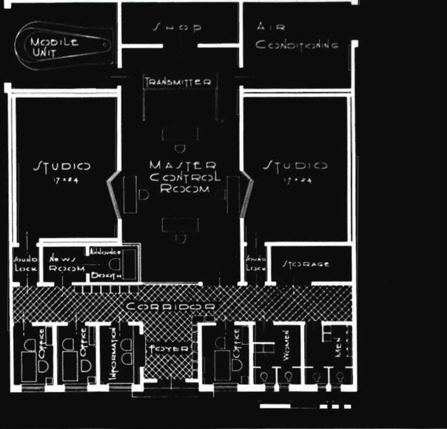
FIG. 1. Floor plan of building designed to house studios, transmitter, offices and other facilities of a small television station.
