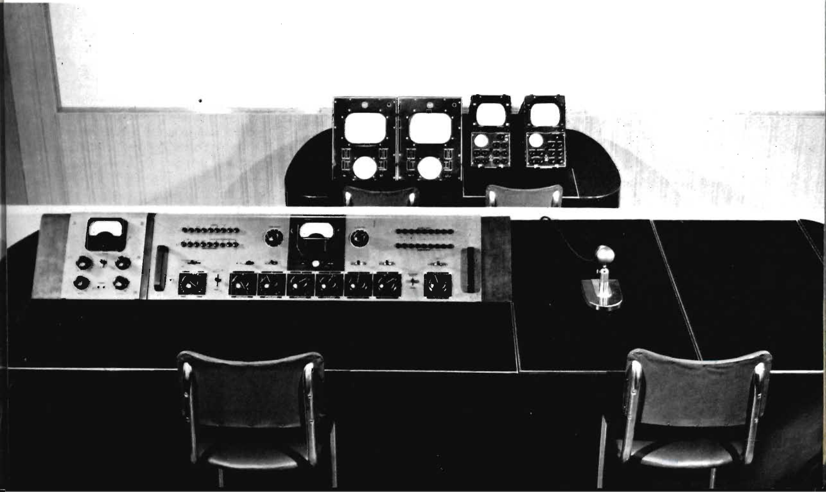
FIG. 24. To provide the director with closer supervision over video switching operations, the TS-10A Camera Switching System can be located on the platform with the audio console, as shown above. Platform setups are possible with any of the equipment layouts described. Photo below shows an arrangement for the Type B station previously described.
