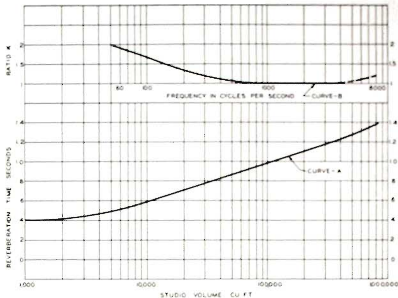
FIG. 16. Optimum reverberation time and frequency characteristics.
