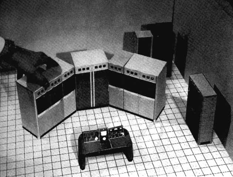
FIG. 10. The models are scaled one inch to the foot. When placed on a card ruled in one inch squares, room dimensions can be determined quickly and easily. Here, the RCA 5 KW transmitter is shown in a "U" arrangement.
