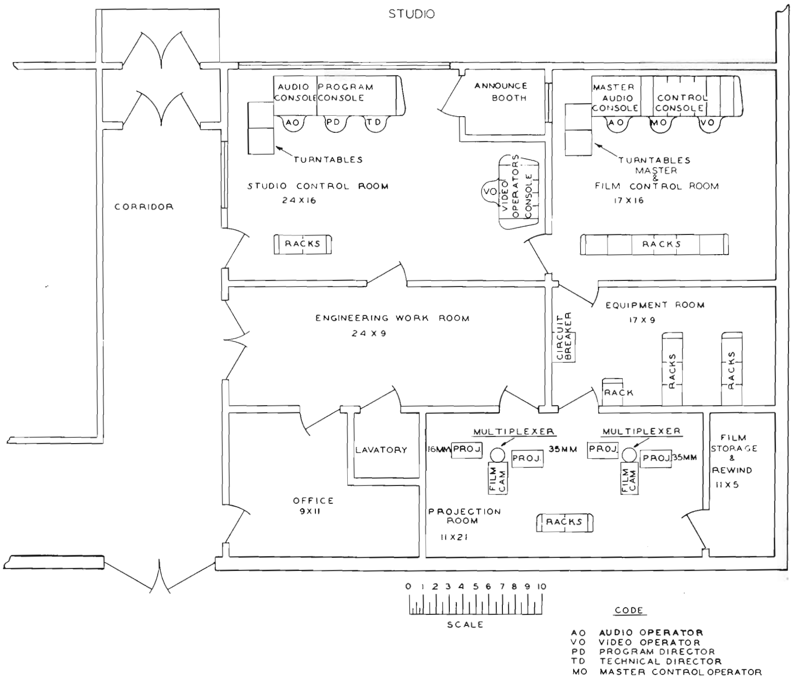
FIG. 28. Partial Floor Plan for the Type D Station. The equipment arrangement shown is for the Type E station described on the following page. The floor plan will serve for both D and E Type layouts. Note location of announce studio so that visual cue can be taken from either control room.
