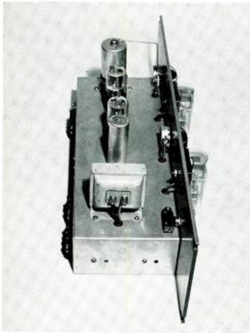
FIG. 2. Chassis view of the KOMO Carrier-audio alarm. It consists of a 5 inch by 14 inch chassis mounted on a standard 19 inch by 5 1/4 inch panel
