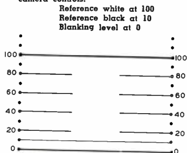
FIG. 2. Operating scale No. 1 for use at camera controls.
