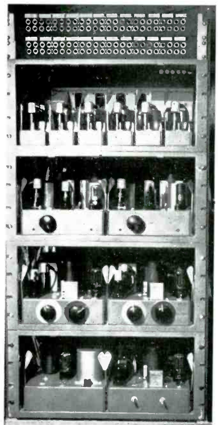
FIG. 24. Partial rear view of the KRON-TV audio console with panels removed to show RCA plug-in amplifiers. Two BA-4A Amplifiers are mounted on front side under operating shelf.
