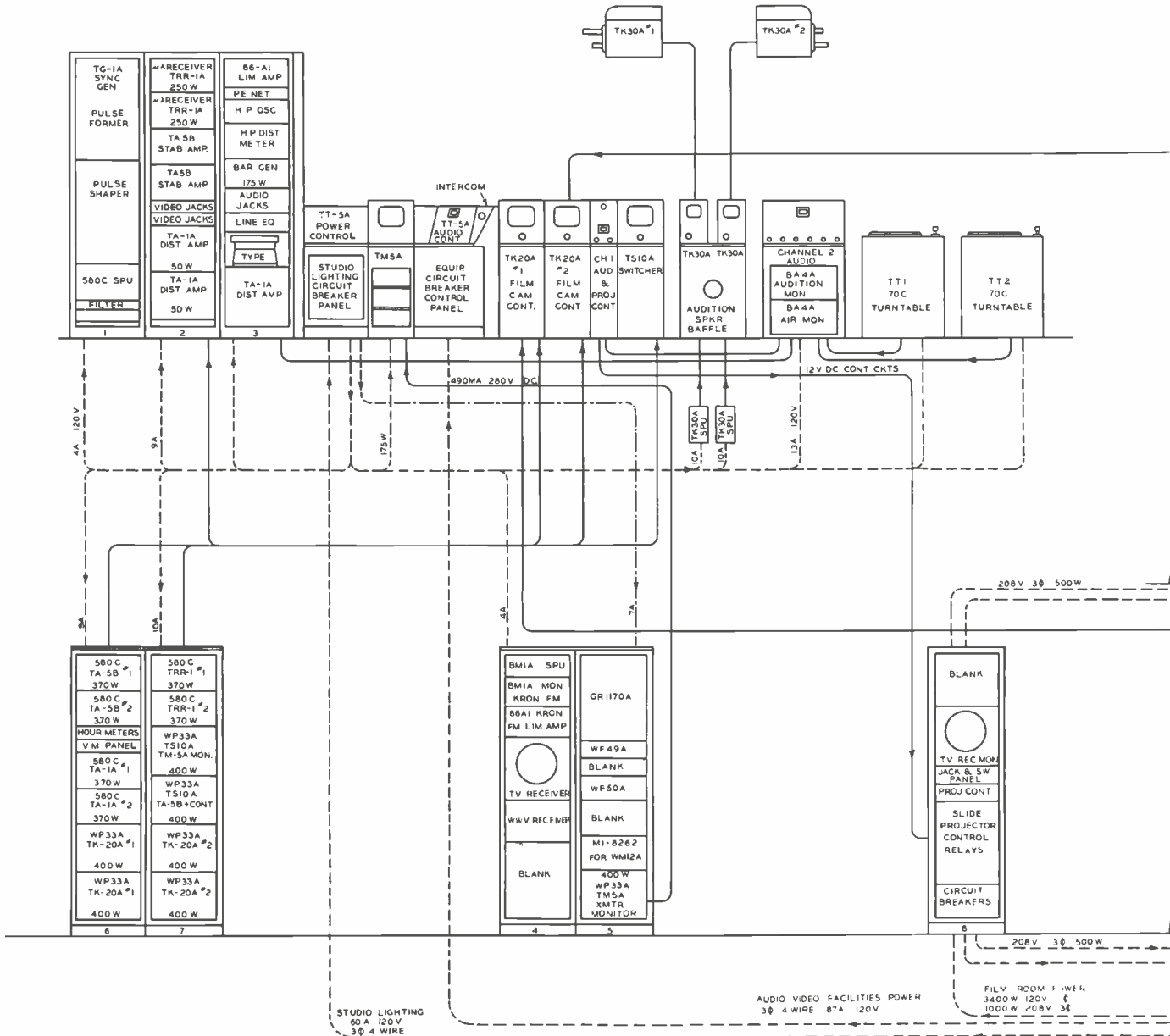
FIG. 18. Simplified diagram showing the interrelated KRON-TV video equipment and facilities employed.
