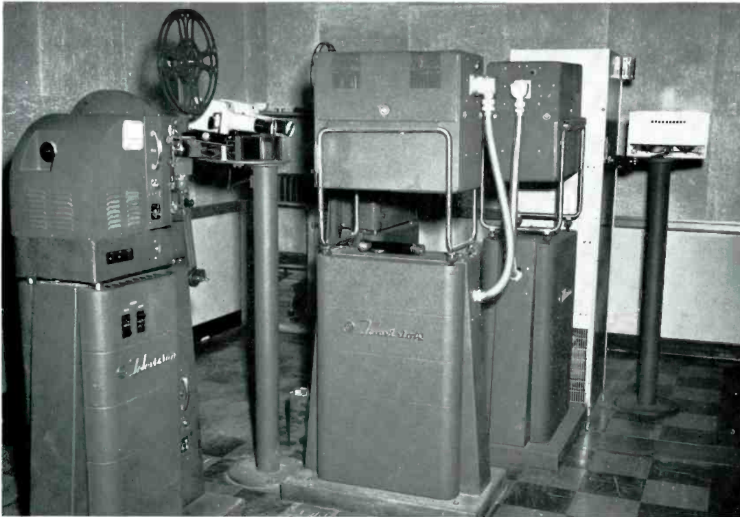
FIG. 14. The projection room directly back of the TV control room. Two RCA TP-16C 16mm projectors, two RCA TK-20 film cameras and a Super Projectal are shown.
