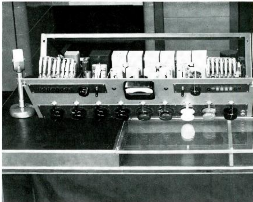
FIG. 4. View of the BC-2B with front panel swung forward to show how every component is accessible.
