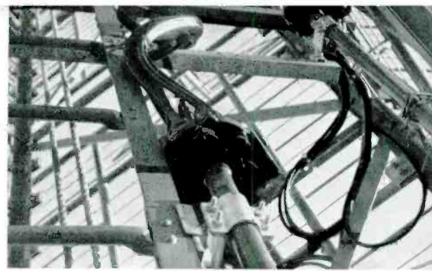
FIG. 10. At right top on N-S transformer and junction box and at center E-W transformer and junction box. Junction boxes are secured by rigid clamp. Cables are dressed and secured so transformers and equalizer may be raised one foot or more for checking transmission line with calibrated termination.
