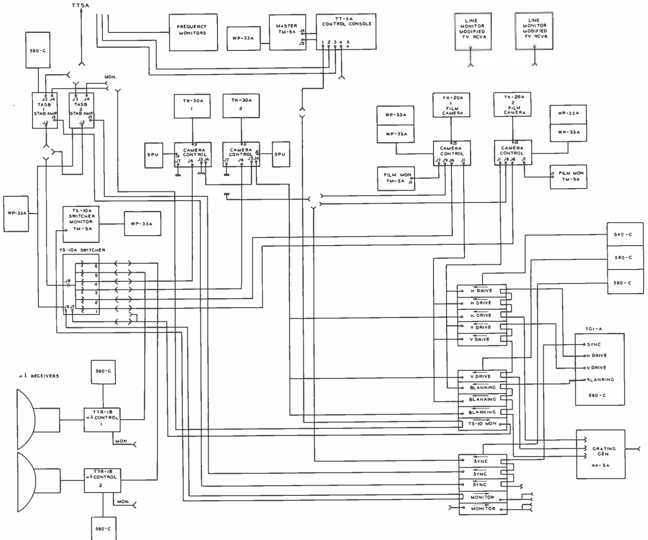
FIG. 20. Block "System" diagram showing the interconnection of KRON video facilities.
