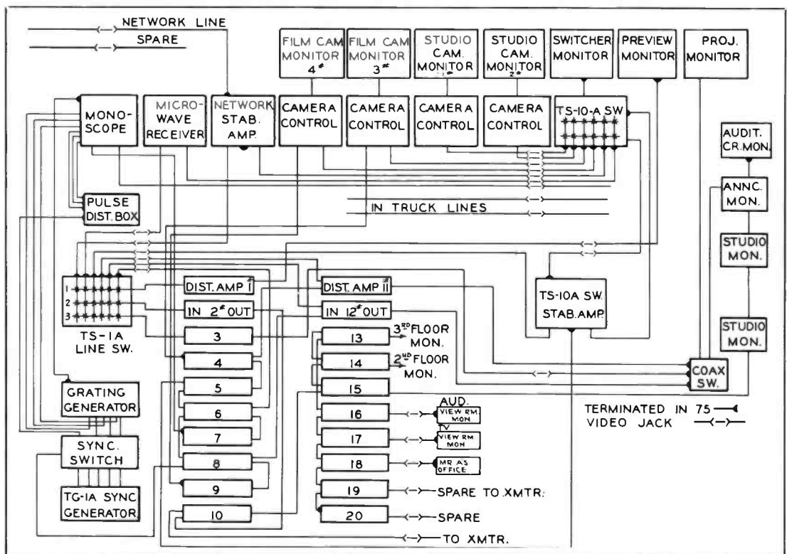
FIG. 11. Block schematic diagram showing WTAR's video system.
