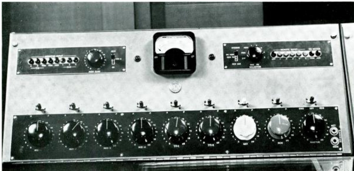
FIG. 1. View of the new BC-2B Console shown in operating position. Eight mixer positions are provided, colored knobs and switches enable quick identification of the important circuits.
