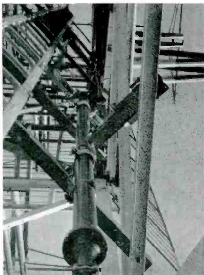
FIG. 5. At top is E-W junction box and at top right, N-S junction with \frac{1}{4} \times straight length of line for 90° phasing. A termination resistor on power equalizer absorbs reflected energy from antenna mismatch to present resistive load to transmission line. This avoids energy reflections back to transmitter.
