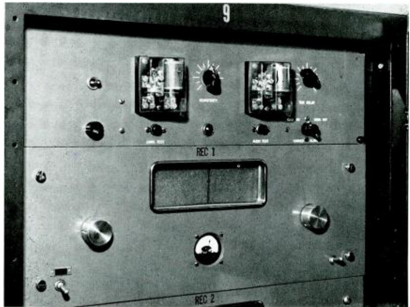
FIG. 1. View of the Carrier-audio alarm (top panel) mounted in KOMO monitoring rack. Bottom panel includes Kappler Hi-fidelity Tuner furnishing "Off-the-air" monitoring plus AVC and audio voltage to the alarm circuit.
