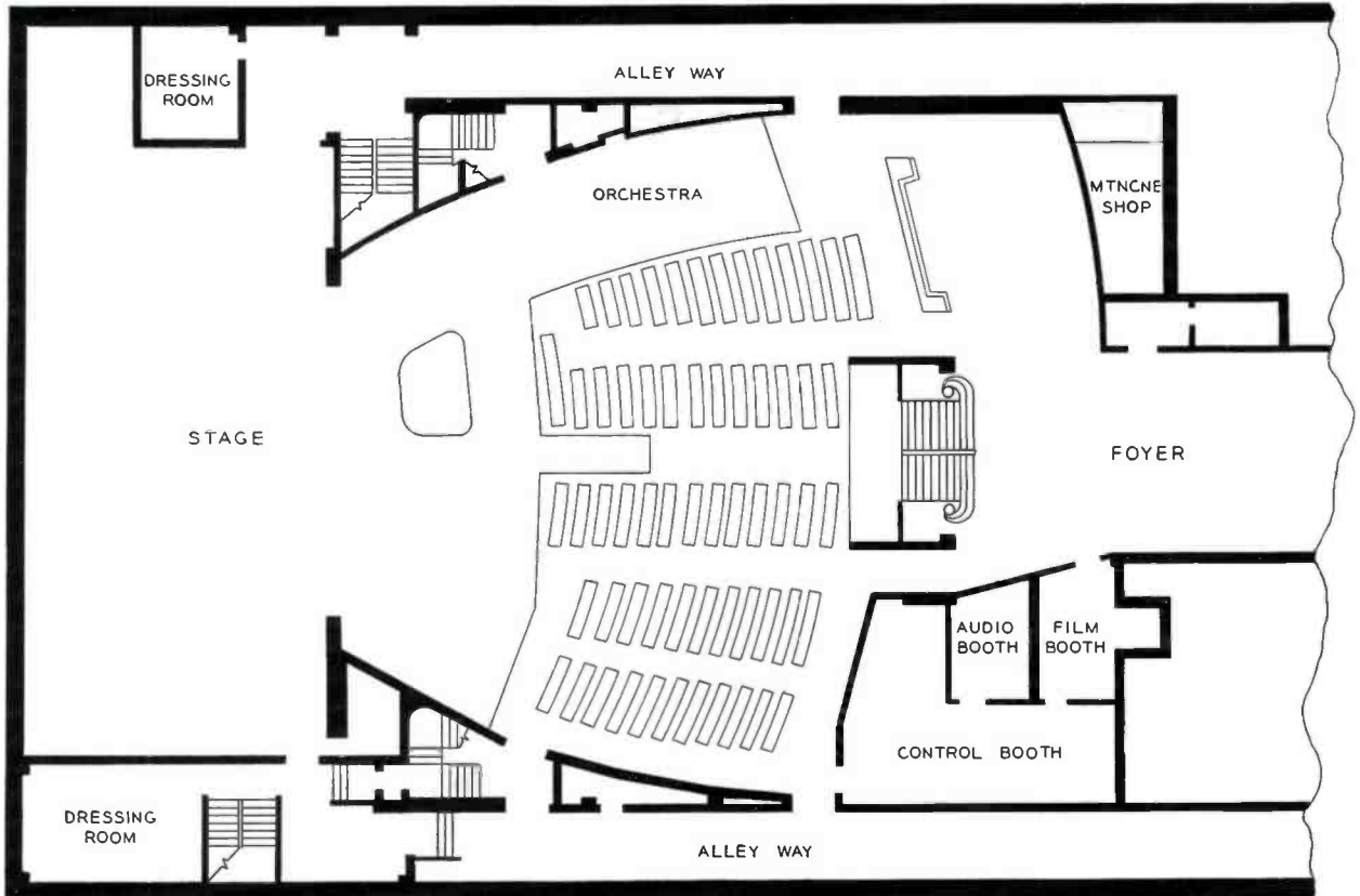
FIG. 3. Floor plan of El Capitan TV "Theatre-Studio."
