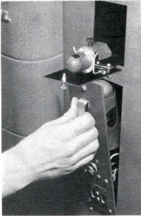
FIG. 8 (left). Shows a closeup of the TP-16D Quick Change Exciter Lamp Assembly. FIG. 9 (right) RCA Type TP-16D 16mm Film Projector features new long-life intermittent. Design advancements include sapphire rails and precision ball bearings to improve picture stability.
