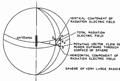
FIG. 1. Antenna in Imaginary Sphere.
