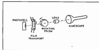
FIG. 15 (above). Continuous Projector using a rotating prism.
