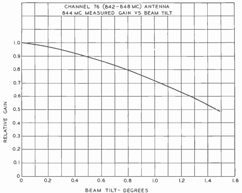
FIG. 23. Curve of Gain vs. Beam Tilt.
