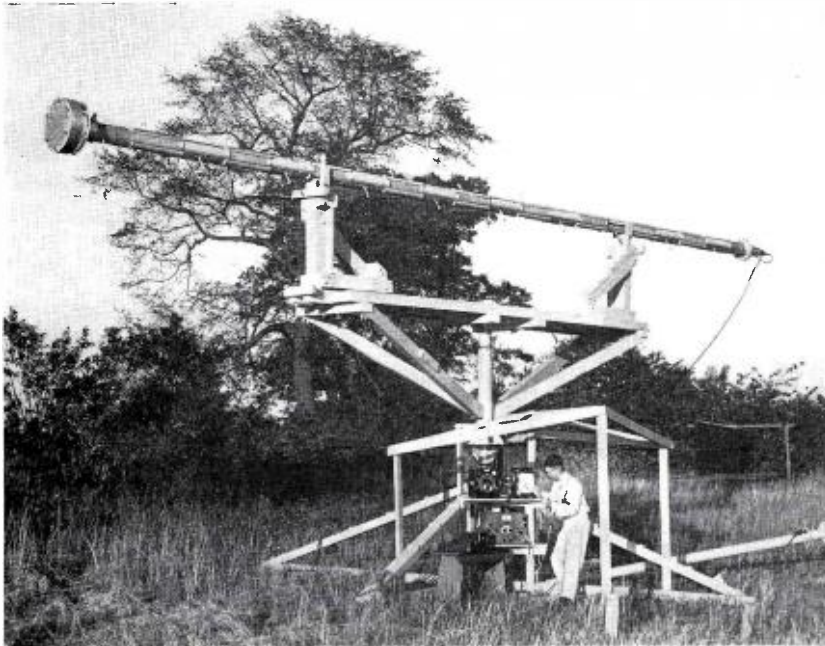
FIG. 4. The Receiving Site with UHF Antenna.
