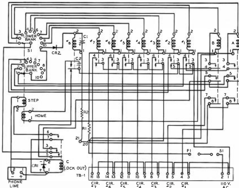
FIG. 8. Schematic Diagram of Telephone Step Equipment.
