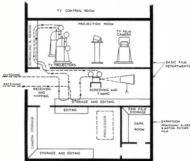
FIG. 17. Routing of film, future expansion, storage and the processing of film are all factors worthy of careful planning.
