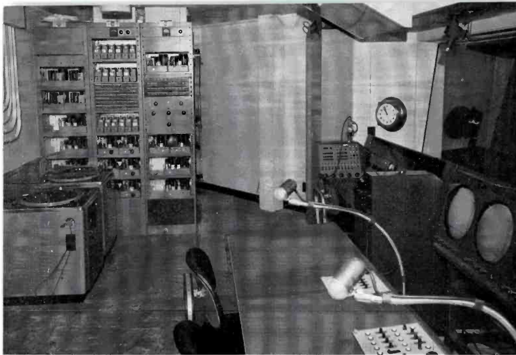
FIG. 10. Visible in this control booth photograph are the Audio Racks (left), the Audio Control Console (right), and part of the Director's Console (lower center).
