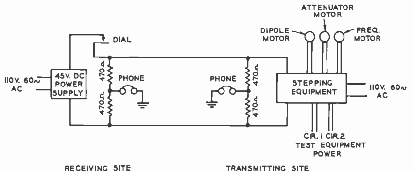
FIG. 9. The Control System.
