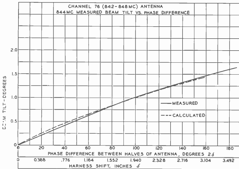
FIG. 22. Curve of Beam Tilt vs. Harness Shift.
