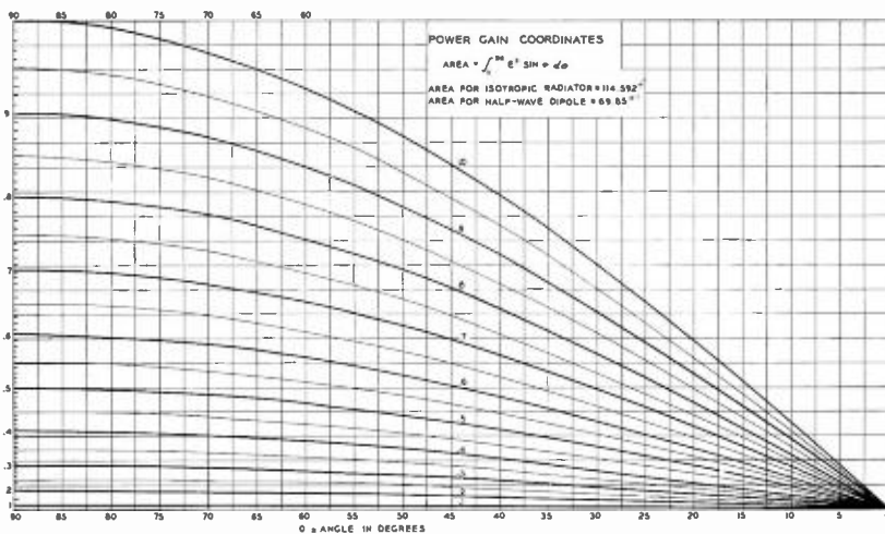
FIG. 18. Power Gain Coordinates.
