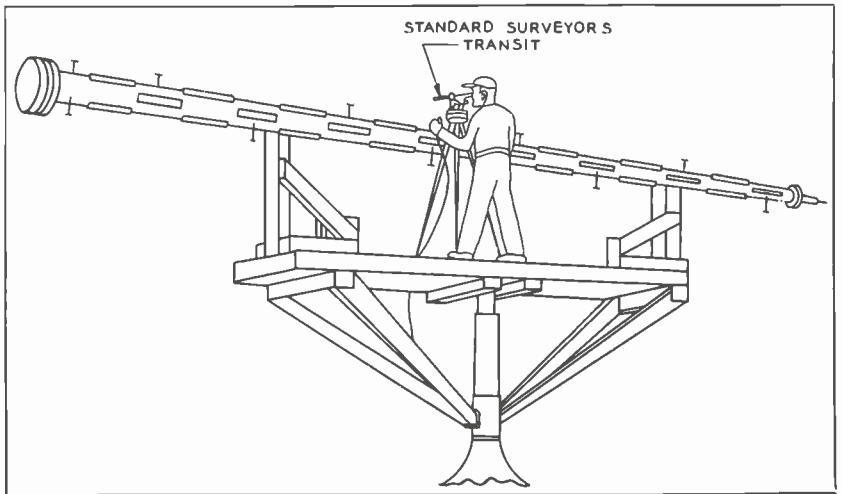
FIG. 16. Transit Test on Overall Recording Accuracy.
