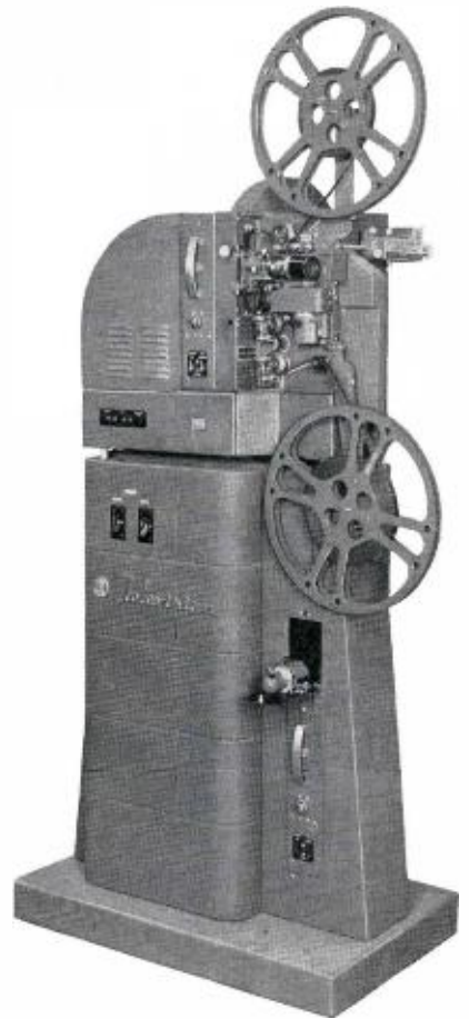
FIG. 8 (left). Shows a closeup of the TP-16D Quick Change Exciter Lamp Assembly. FIG. 9 (right) RCA Type TP-16D 16mm Film Projector features new long-life intermittent. Design advancements include sapphire rails and precision ball bearings to improve picture stability.
