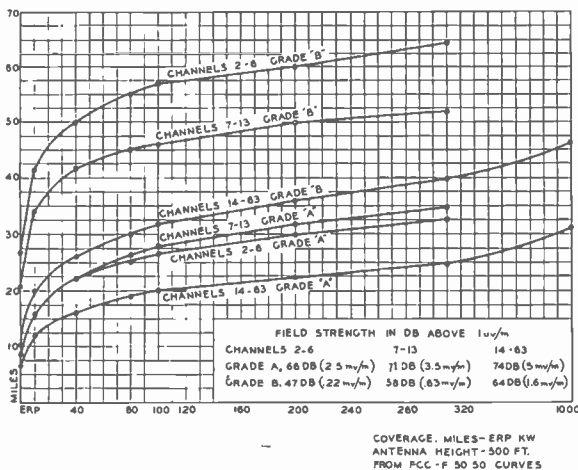
FIG. 10. Coverage curves showing "ERP" versus "Miles Coverage".
