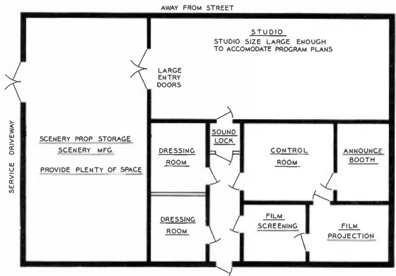
FIG. 13 (at right). Typical TV Studio floor plan.
