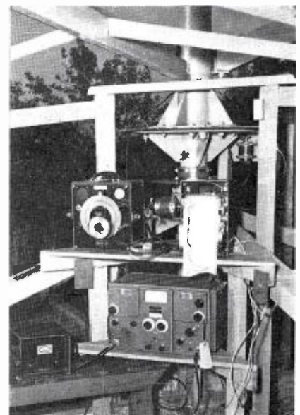
FIG. 5. Test Equipment at the Receiving Site.
