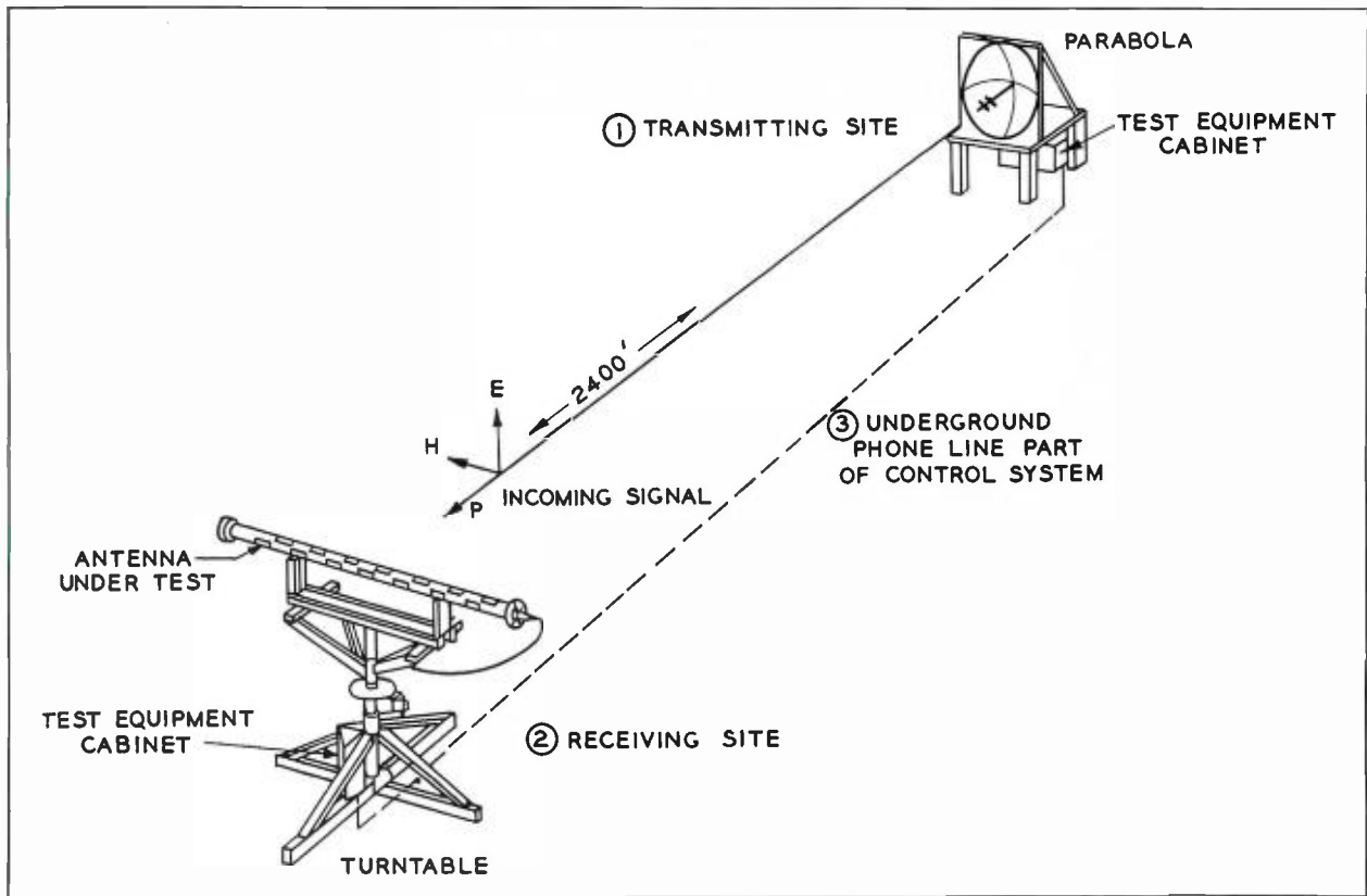
FIG. 3. Pictorial View of Antenna Test Ground.
