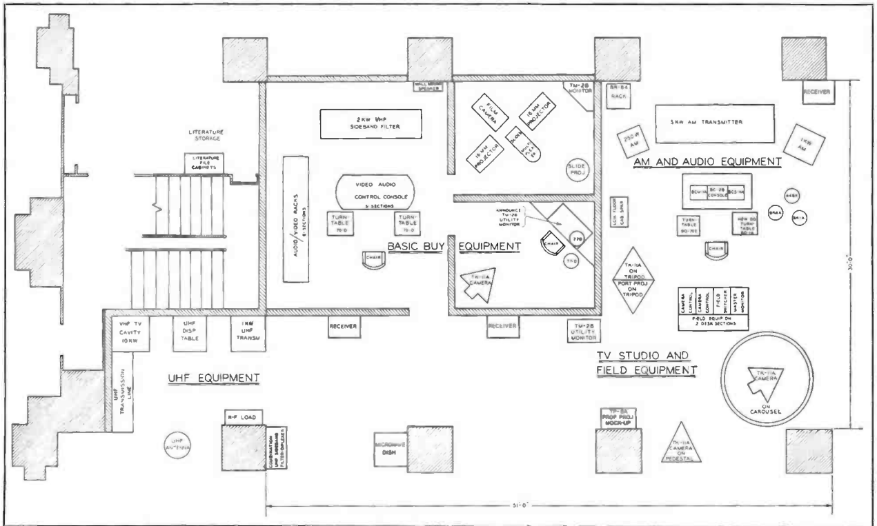
FIG. 2. Floor plan of the RCA exhibit layout.
