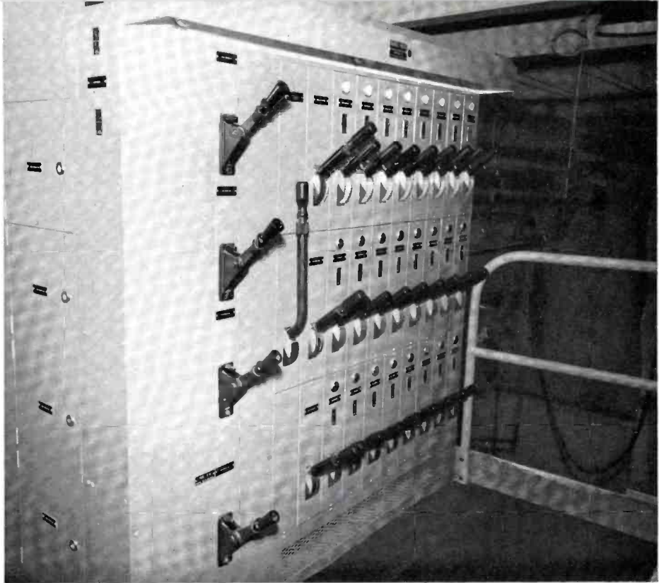
FIG. 5 (right). The Borderlight Dimmer Board. Mechanical interlocking allows simultaneous dimming of borderlight units. The Mezzanine Plan shown in FIG. 6 (middle) illustrates the lighting control equipment layout and is located above the main floor control booth. The Control Dimmer Board, seen in FIG. 7 (bottom), in a manner similar to the Borderlight Dimmer Board allows the simultaneous dimming of all stage circuits.
