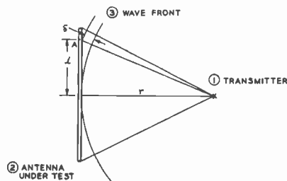
FIG. 10. Geometry of Path-Length Difference.
