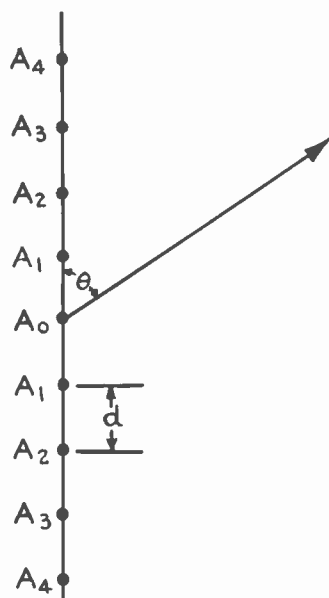
FIG. 11. Array of Point-Sources.
