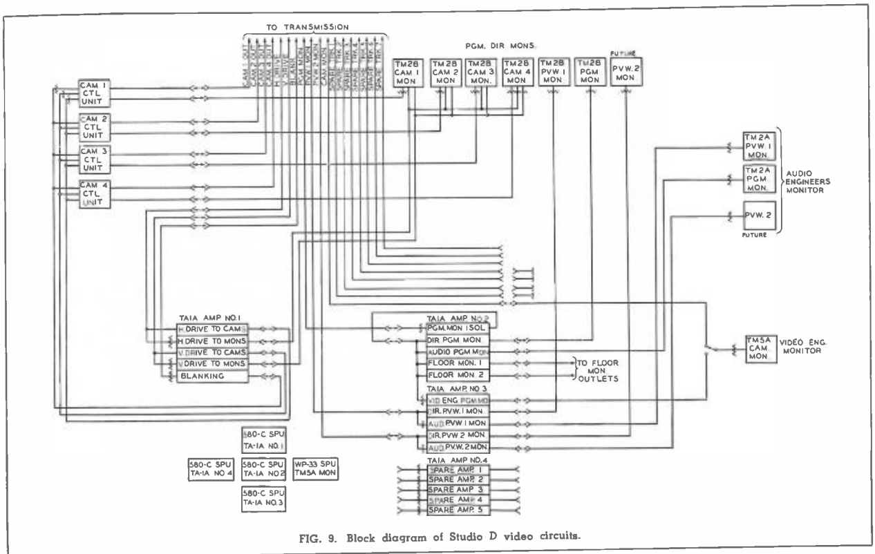
FIG. 8. Studio D switching circuits.
