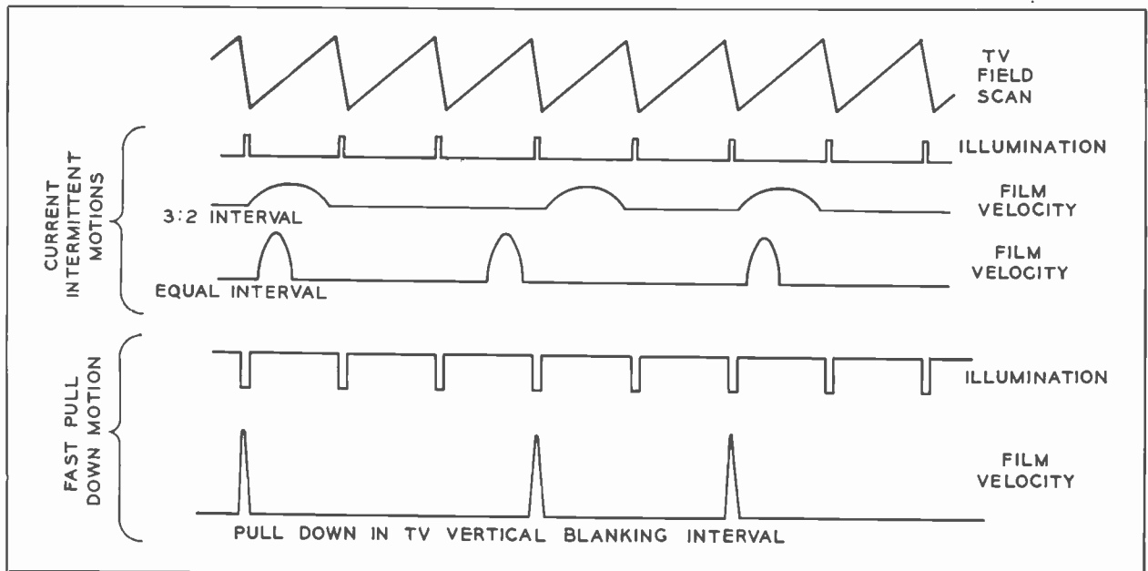
FIG. 5. Timing relationships in TV intermittent projectors.
