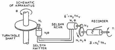
FIG. 15. The Recorder Drive System.
