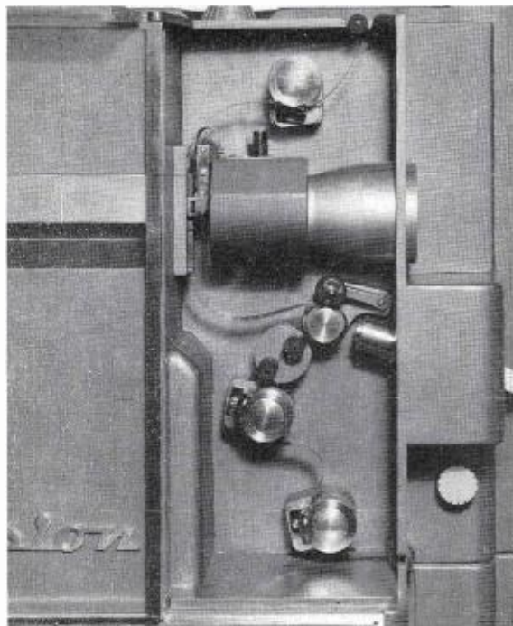
FIG. 6 (left). The Professional 16mm TV Projector which features 2-3 claw pull down, precision optics, and quick-change exciter lamp. This projector accommodates 4000-foot reels and has compensated take-up. FIG. 7 (right) is a closeup of the threading and optical system of the TP-6A 16mm Projector.
