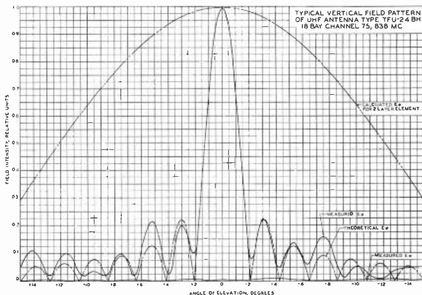
FIG. 12. Vertical Pattern of TFU-24BH.
