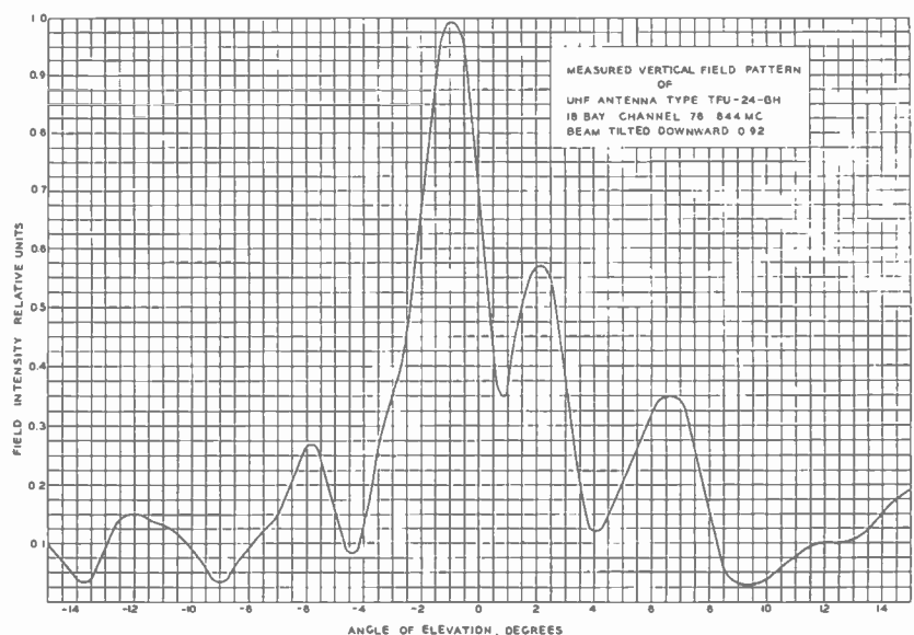
FIG. 14. Tilted Vertical Pattern.
