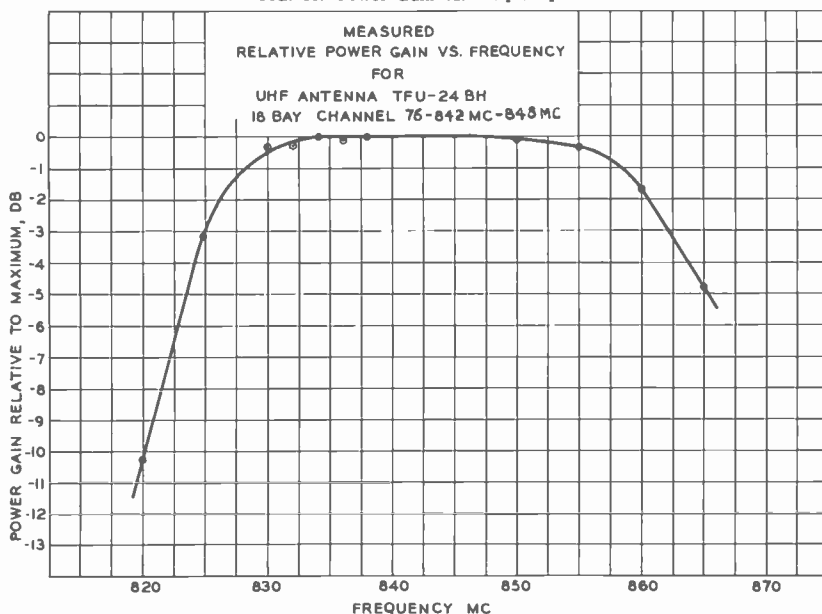
FIG. 19. Power Gain vs. Frequency.
