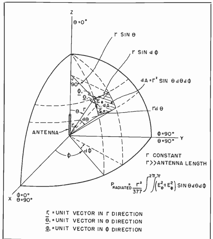
FIG. 2. Spherical Coordinate System.
