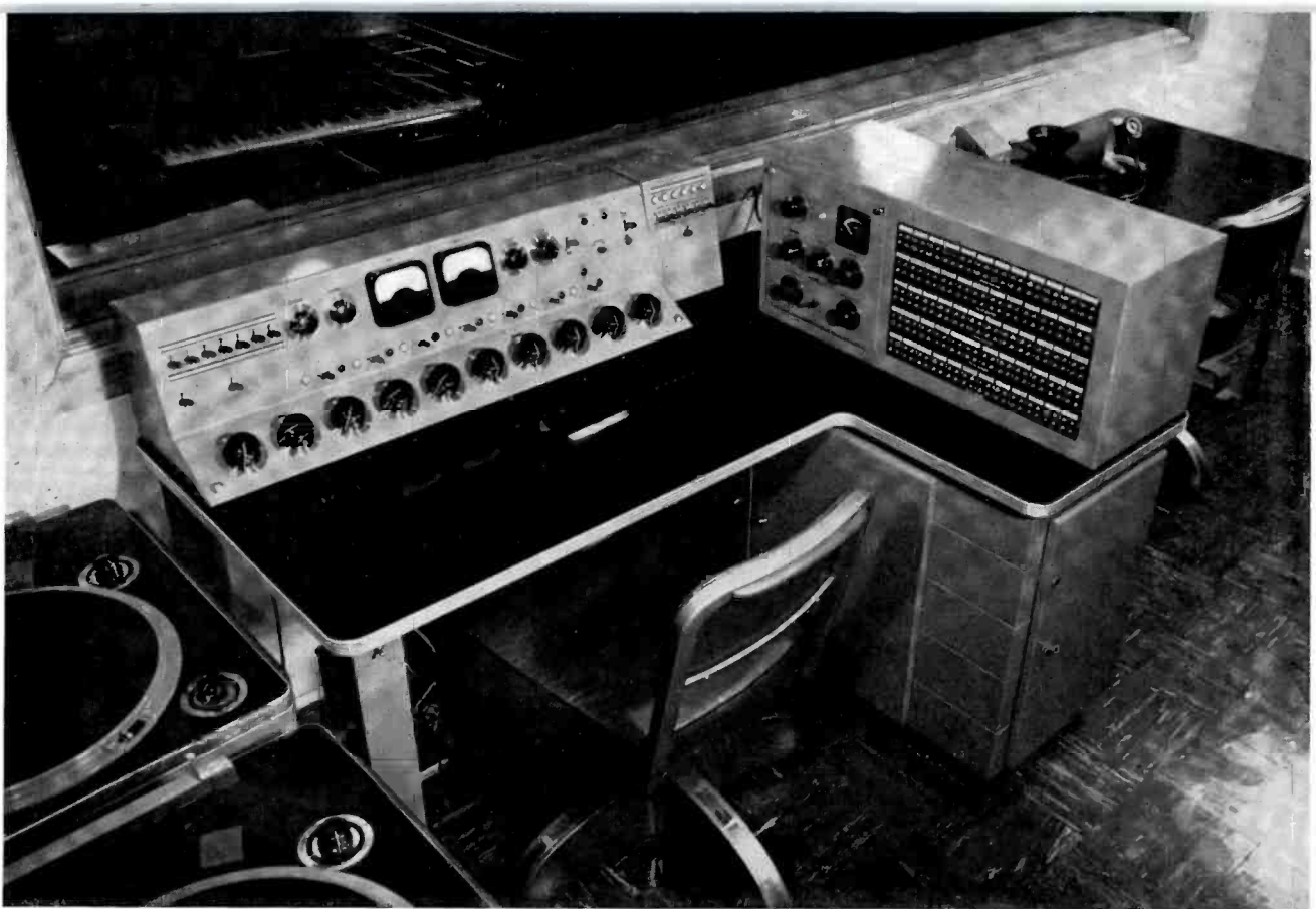
FIG. 30. Each of WBAP's six main AM-FM studios has its own control booth. The booths are identical in size and construction and each is equipped (as shown above) with either two or three RCA Turntables (left), a special RCA custom-built control console (center) and a program director's table (right). The RCA LC-1A Loudspeakers are mounted in the ceiling overhead.
