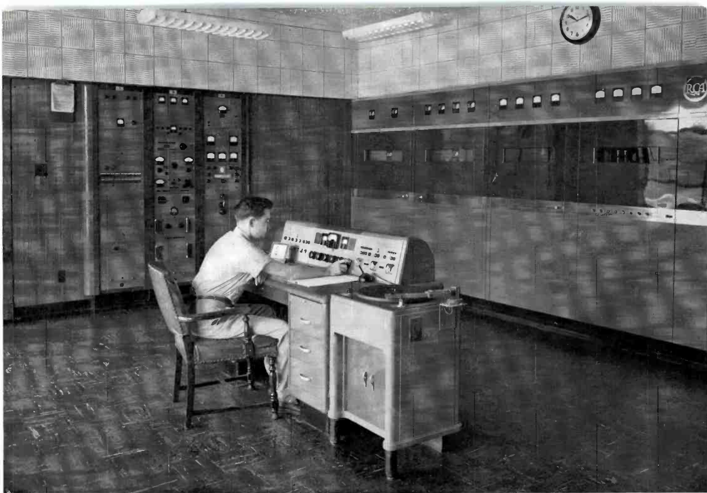
FIG. 4. This is the WHBQ 5000-watt transmitter, and RCA Type BTA-5-F. The first rack on the left contains speech input equipment; the second rack holds test equipment; and the third rack contains frequency phase monitors.
