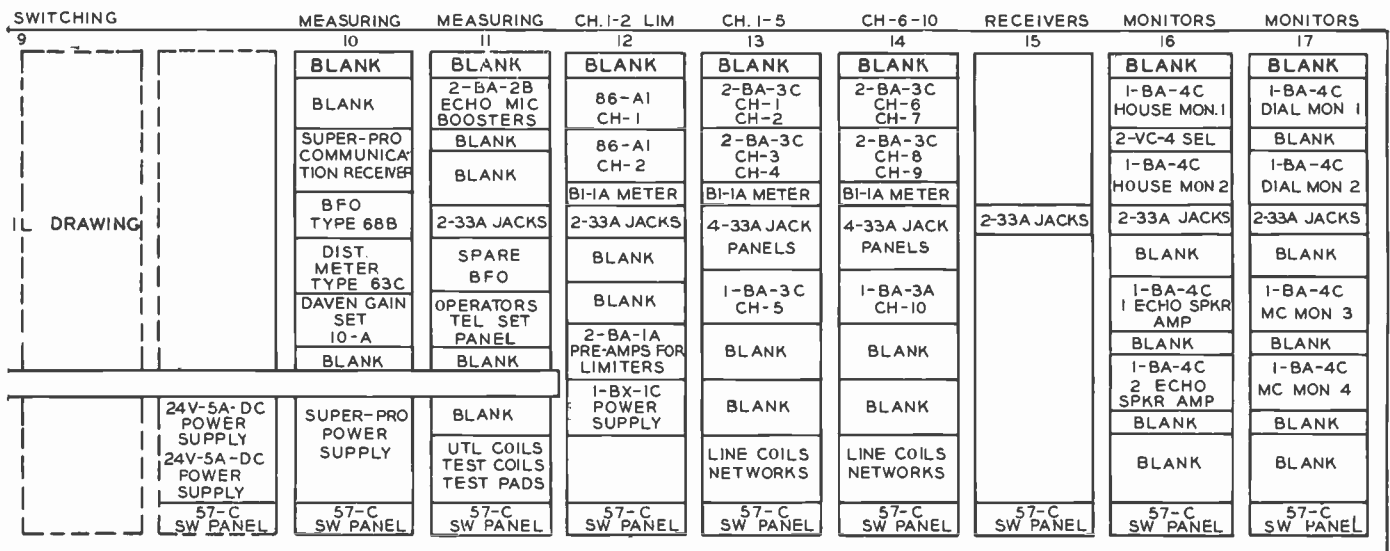
FIG. 1 (opposite page). WBAP's AM-FM Master Control Room equipment consists of sixteen standard racks of equipment units plus special four-rack-wide center section on which main operating controls are grouped. These racks take up one whole side of the forty-foot long control room. The opposite side of the room and one end (far end in this view) consist of floor length windows through which visitors to the building can observe the control operation.
