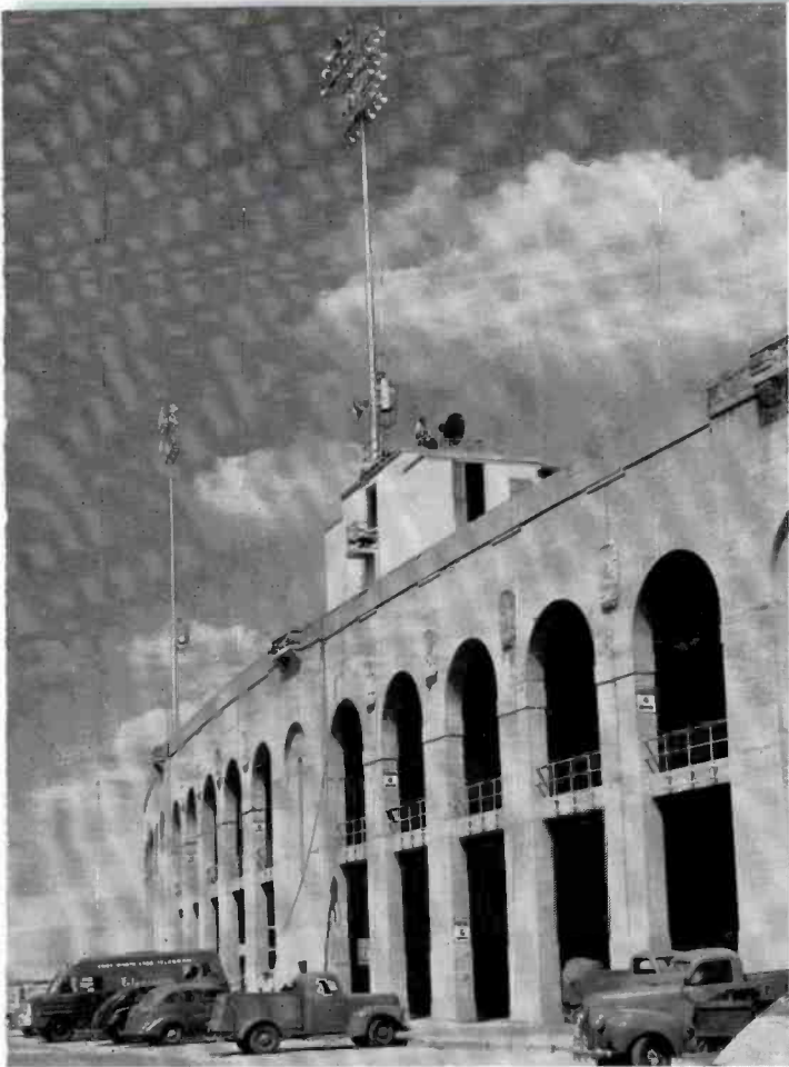
FIG. 23. For pickups at the stadium, ball park and similar events, WBAP leaves the control equipment in the mobile unit, uses long cables to cameras and microwave parabola located at vantage points.
