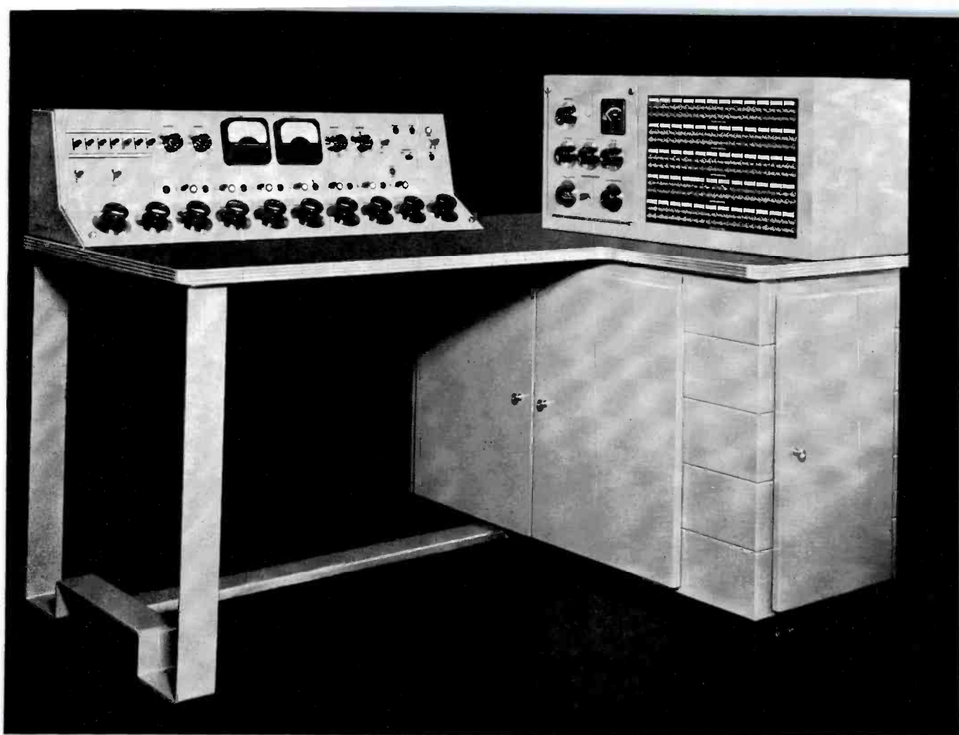
FIG. 1. Each of WBAP's six AM-FM studios has its own control booth, and each booth is provided with a control console like the one shown above. These all-steel consoles, custom-built for WBAP by RCA, contain all the equipment facilities (except microphones, loudspeakers and turntables) which are required for complete independent operation of the studio for all conceivable types of programming. Additional views of console shown on following pages.
