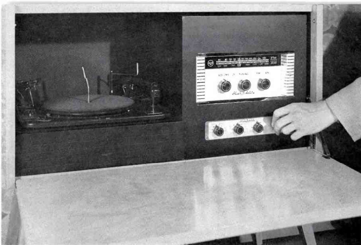
FIG. 5. The player, preamplifier and tuner may be easily mounted in this convenient equipment cabinet. The cabinet shown here has a hinged door. However, production models have a door which slides up under the top. This gets the door out of the way and looks better when cabinet is left open.
