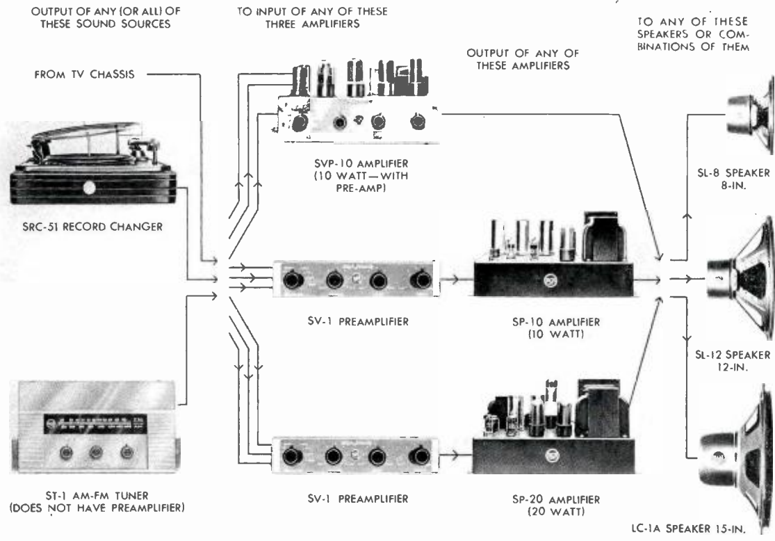
FIG. 6. This diagram indicates possible combinations of RCA Hi-Fi units using the Type ST-1 Tuner. This tuner has sufficient output to drive a power amplifier directly. However it does not include a preamplifier or provisions for handling record player input. It is necessary, therefore, to use with it, either the Type SVP-10 Amplifier (with built-in pre-amp) or the separate Type SV-1 Preamplifier feeding into either an SP-10 or an SP-20 Power Amplifier.
