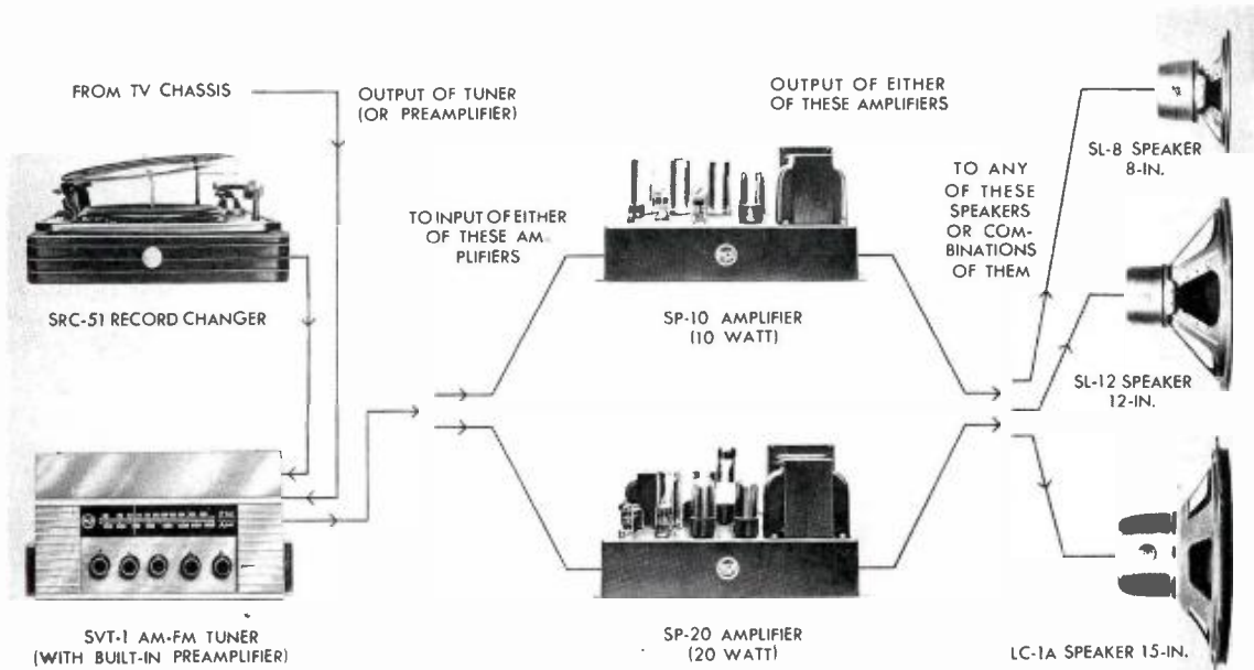
FIG. 7. Possible combinations of RCA Hi-Fi units using the deluxe Type SVT-1 Tuner. This tuner has a built-in preamplifier together with an input selector switch for player, radio, television, auxiliary and tape inputs. Thus its output may be fed directly to the input of an SP-10 or SP-20 Power Amplifier. In these combinations, or those shown above, the output of any amplifier may be fed to any of the three types of speakers.
