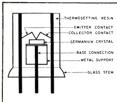
FIG. 2. Construction details of the RCA developmental point-contact transistor.
