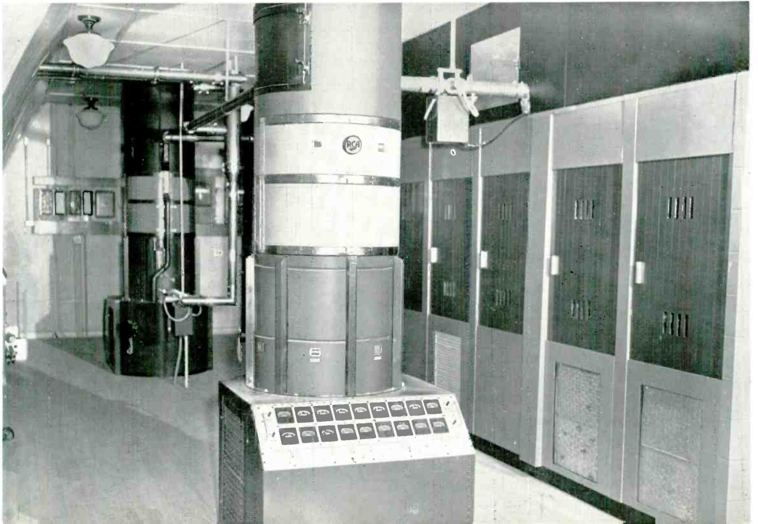
FIG. 6. Shown is a front view of the KBTB 25-KW Aural Power amplifier.
