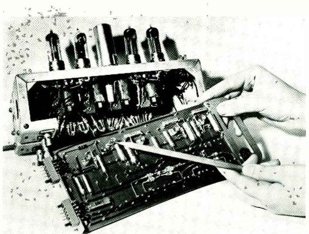
FIG. 16. (Foreground) Transistors point way to new small-size units in electronic computers. Pencil points to one of five developmental point-contact transistors which do the job of the four tubes and four transformers of the rear unit.
