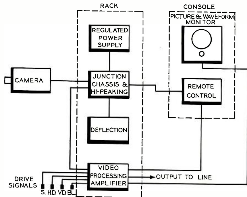
FIG. 7. Block diagram illustrating the components making up the Vidicon Camera Chain. Although shown by two boxes, the Junction Chassis and Video Processing Amplifier are physically one unit.
