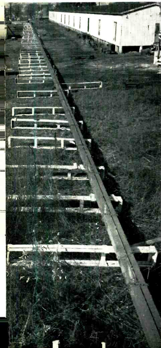
FIG. 3. At RCA Camden plant a 700-foot test length of waveguide is used to obtain VSWR and attenuation data.
