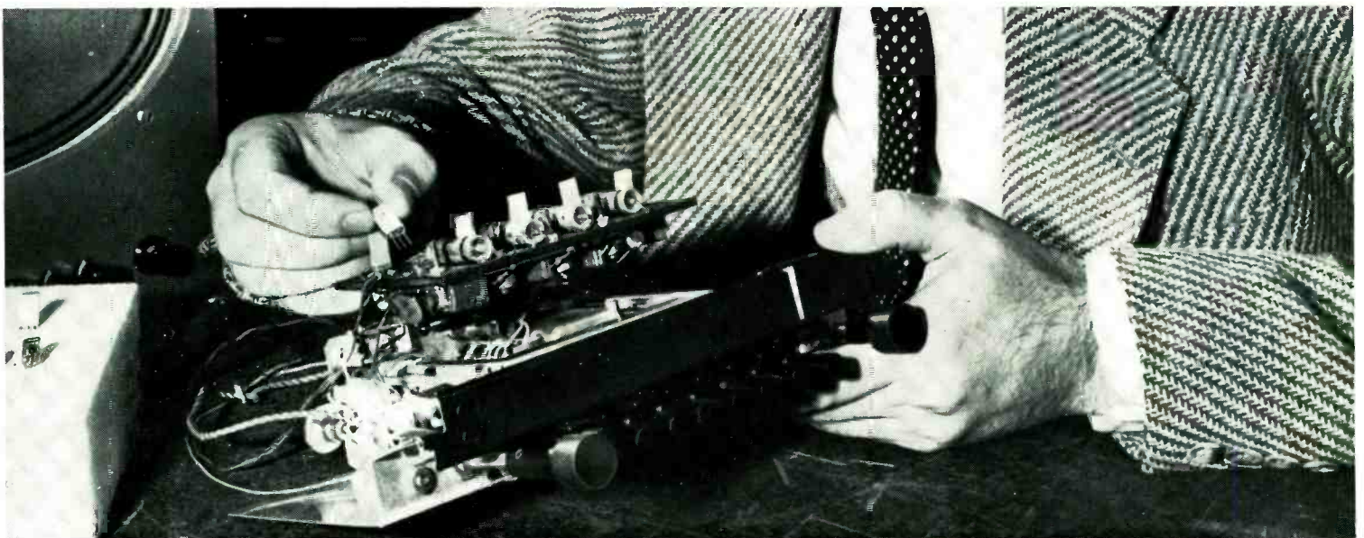
FIG. 11. An auto radio operating solely from 11 developmental transistors. Eliminates the usual high-voltage power supply. Transistors operate from 6-volt storage battery. Receiver operates at 10% of usual battery drain.
