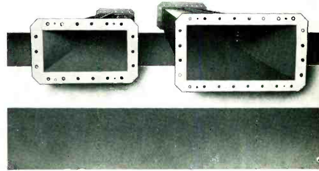
FIG. 6. End view of Waveguide Rigid Sections. Cross-section of WR-1150 (left) is 5\frac{3}{4}'' \times 11\frac{1}{2}'' —18 holes in flanges. Cross-section of WR-1500 is 7\frac{1}{2}'' \times 15'' —24 holes in flanges.
