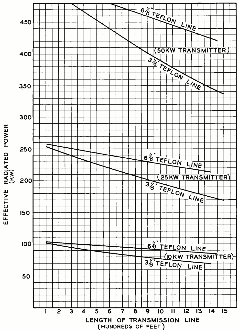
FIG. 6. Curves showing the various values of Effective Radiated Power obtained with various transmitter ratings and transmission line sizes.
