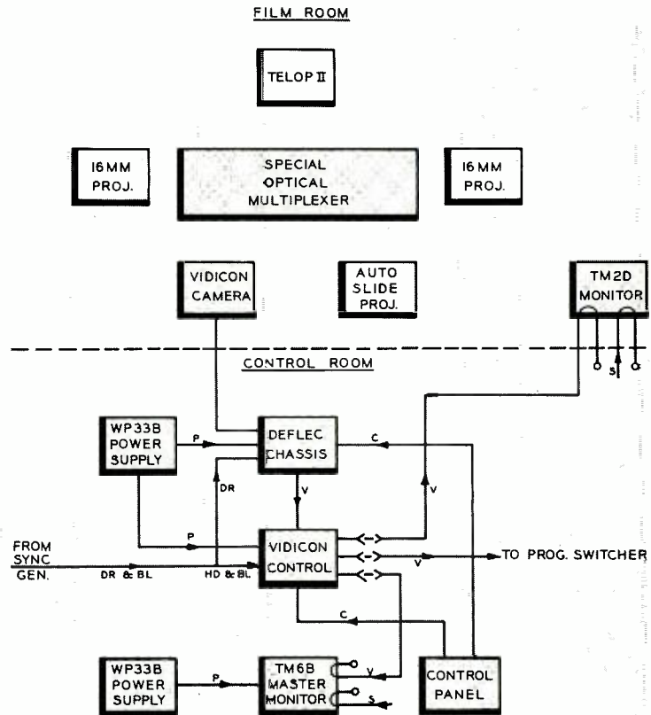
FIG. 10. Simplified system block diagram showing a typical film room setup employing the Vidicon Camera with film projectors, slide projector and multiplexer.
