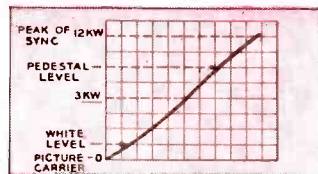
Curve illustrating the linearity characteristic of the RCA TTU-12A transmitter.
