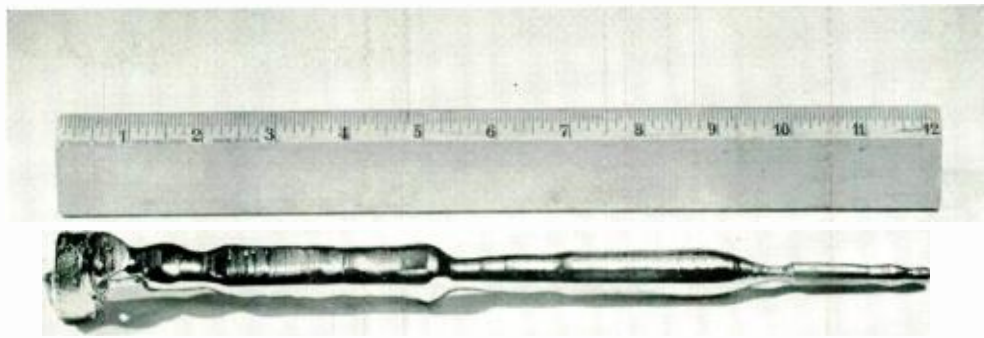
FIG. 12. A single germanium crystal grown in the crystal-growing apparatus of Fig. 3.
