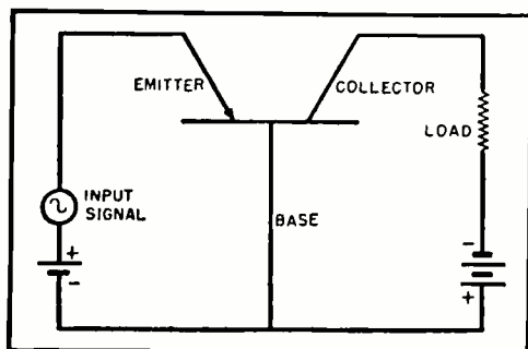
FIG. 18. Transistor amplifier circuit.
