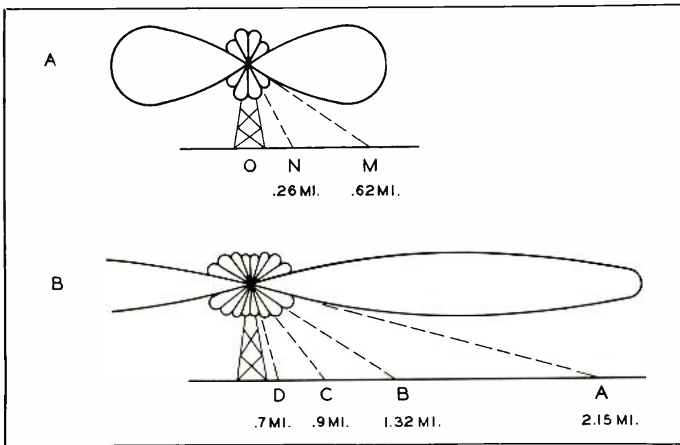
FIG. 3. Pattern curves which illustrate the areas of minimum signal experience with the usual antenna (note points "O", "N", "M", "D", "C" and "B").
