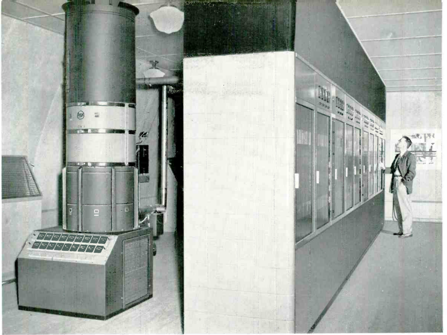
FIG. 5. Full length view of KBTB's new 25-KW VHF transmitter (RCA TT-25BH). At left is one of the high power amplifiers.
