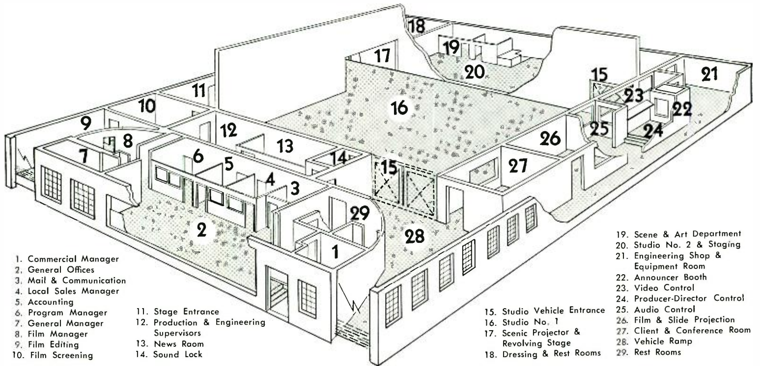
FIG. 1. Operational facilities at KBTV are graphically shown in this cut-away sketch of the station's new building. All facets of the operation are conveniently laid out for ease of operation.
