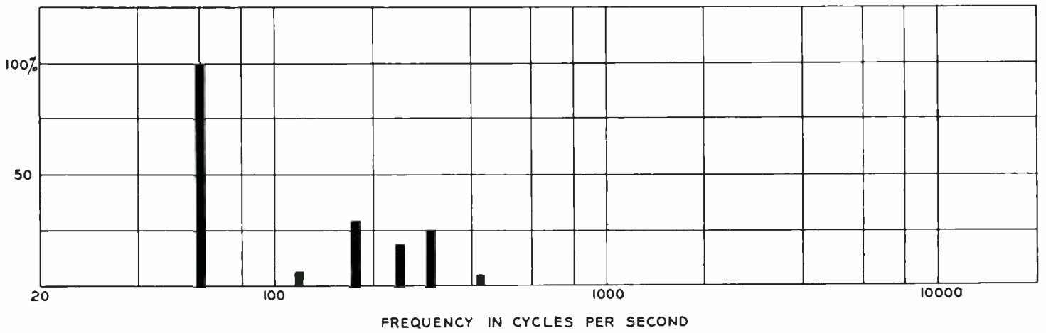
FIG. 6. Field analysis near 80-watt fluorescent fixture.
