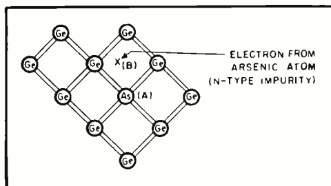
FIG. 15. The effect of "n"-type impurities on the conductivity of germanium crystals.
