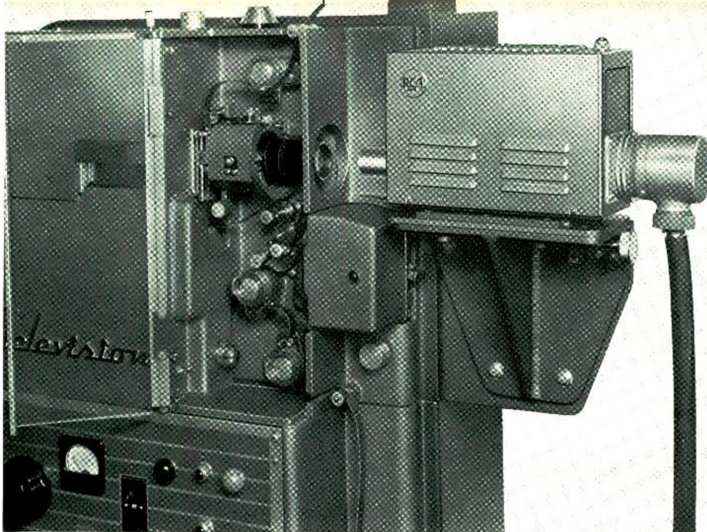
FIG. 1. View of the Vidicon Film Camera shown coupled to an RCA TP-6A Professional 16mm Television Projector.
