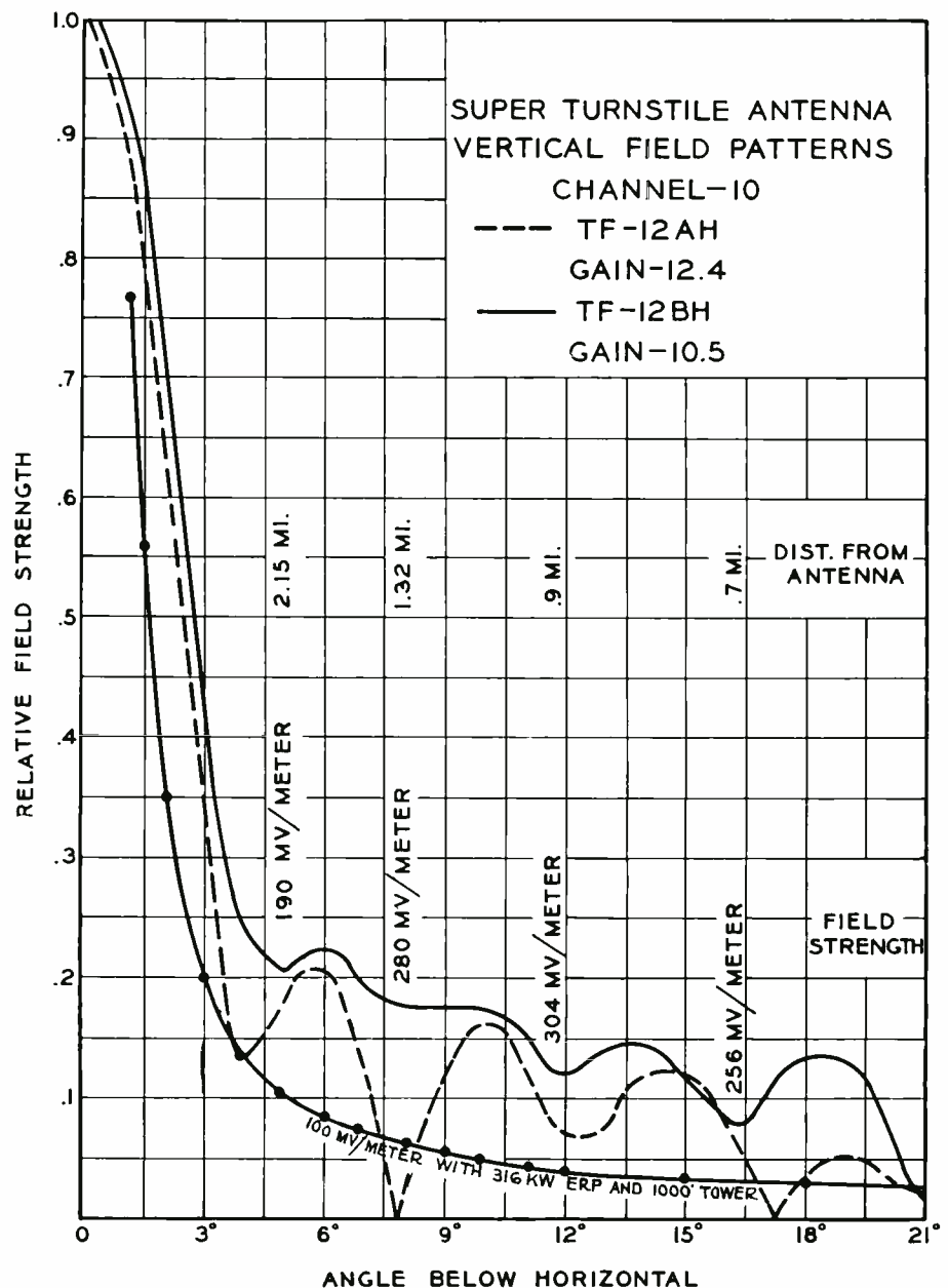
FIG. 4. Curves showing the vertical field patterns of the TF-12BH and TF-12AH antennas. Note how the minimum signal areas are "filled-in" with the TF-12BH.
