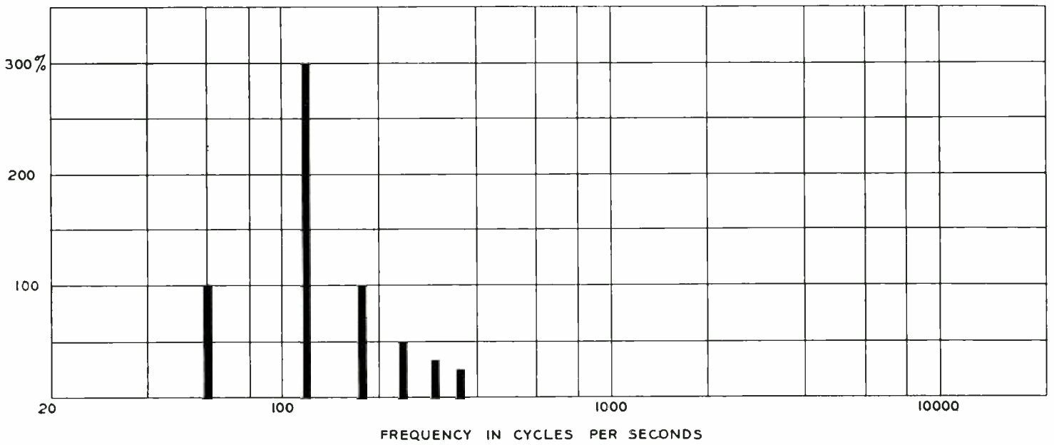
FIG. 5. Field analysis near power amplifier.
