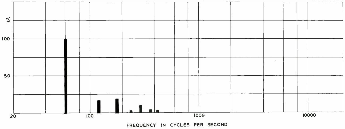
FIG. 4. Field analysis in a typical Broadcast studio.
