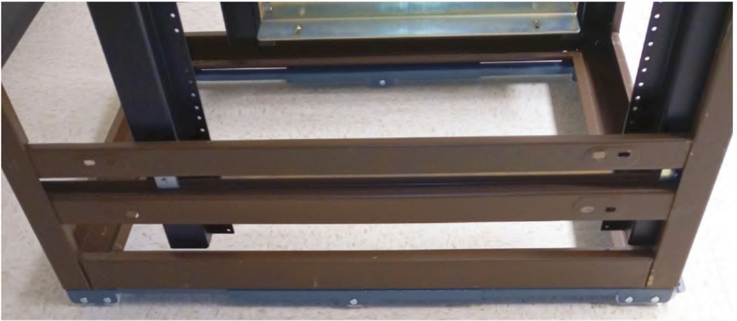
Above The completed rolling base, adjusted for the size of the rack.
