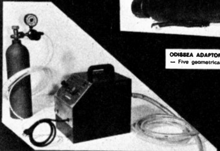
SMOKE MACHINE cod. 800/8 — Input V 220 HZ 50 — Absorption W 750 — The smoke is obtained with a special oil sterilized and shovied by a CO/2 adjustable casting
