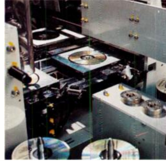
Label imprinting process
