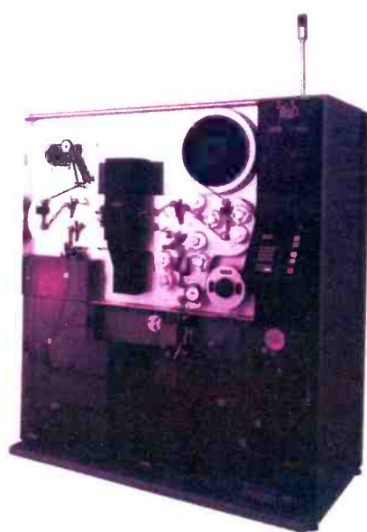
Otari's T-700II TMD (Thermal Magnetic Duplication) videotape high-speed duplicator.
