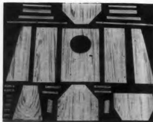
Pieces supplied precut, ready for assembly into compact corner horn model Baronet, takes eight-inch speaker, costs $26 as a kit. Electro-Voice, Inc. Fig. 3a.
