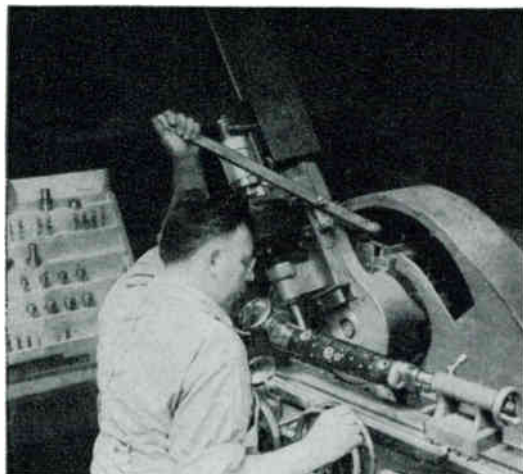
Bassoon maker drills holes at angles, using a specially built machine.
