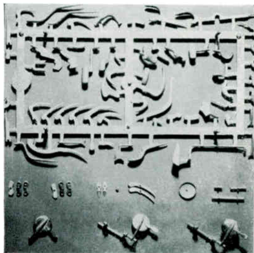
One set of 35 alto-sax keys cast at one operation. After 1100 other manufacturing operations, a finished set of keys results.
