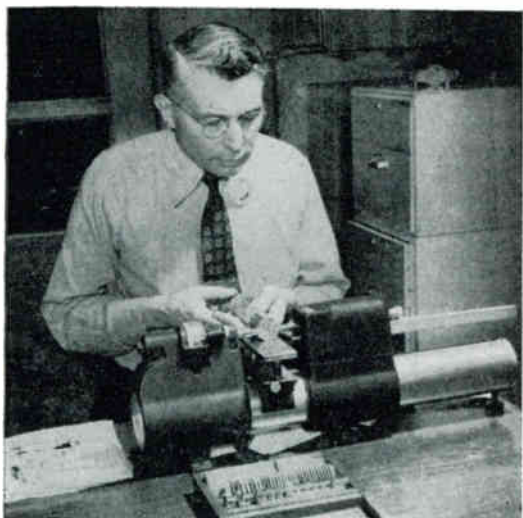
Pratt-Whitney supermicrometer checks gauges to one ten-millionth of an inch.
