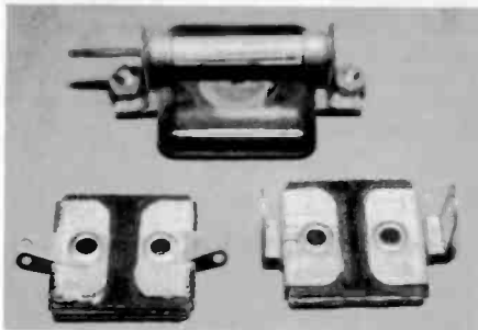
Figure 1. Three examples of early mica capacitors: From left to right: a 0.006 mF of open construction; a 0.002 mF with clips for mounting a grid leak resistor, and a Micamold brand molded case capacitor with a grid leak in place.
