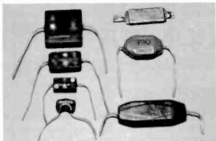
Figure 4. These examples of mica capacitors from RCA and other manufacturers are described in the text.
