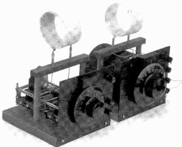
Figure 2. The two finished, home-brew units: the main tuner is shown at the right. The 2-gang variable capacitor can be seen in the antenna tuner on the left.
