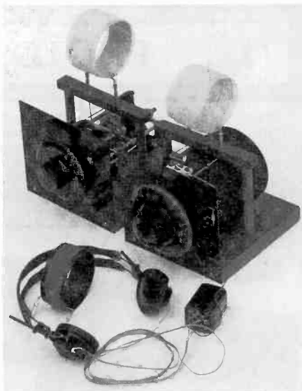
Figure 3. The complete crystal set with the out-board audio-matching transformer.
