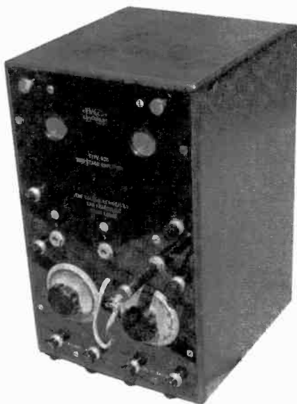
KENNEDY TYPE 525 AMPLIFIER – This 2-tube amplifier was manufactured by the Colin B. Kennedy Co. of St. Louis, Missouri. It was made to connect to the 1921 Kennedy Models 110 and 220 1-tube receivers. ( Dave Crocker – Mashpee, MA )
