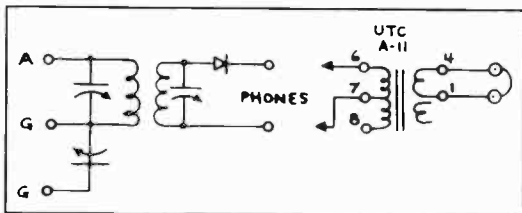
Figure 1. The schematic diagram for the crystal set shows the antenna tuner on the left. Note the two ground connections. Their use is explained in the text. The tuner/detector is shown at the center and the outboard audio matching transformer and headset connection are shown on the right. One winding of the transformer is not used.
