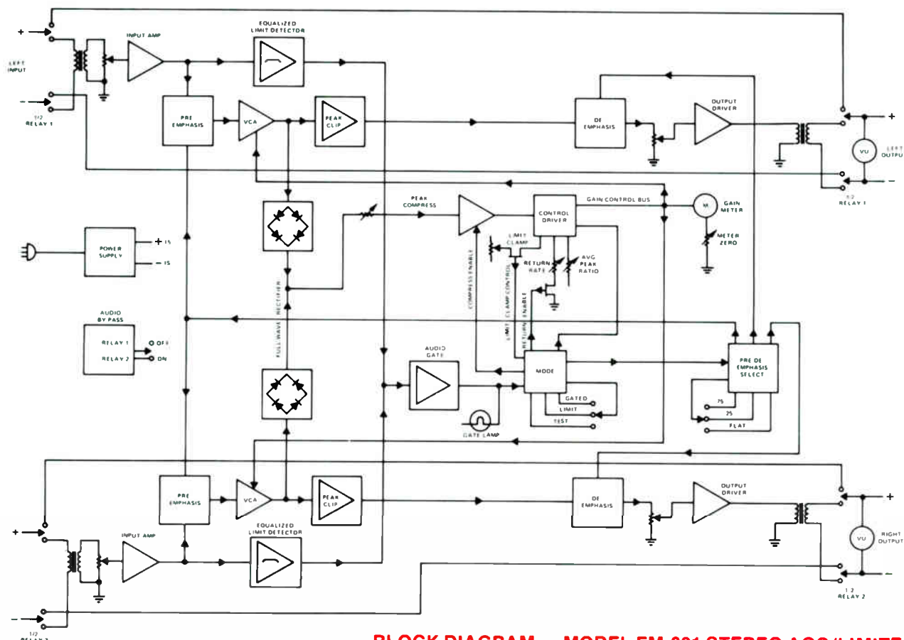
BLOCK DIAGRAM — MODEL FM-601 STEREO AGC/LIMITER
