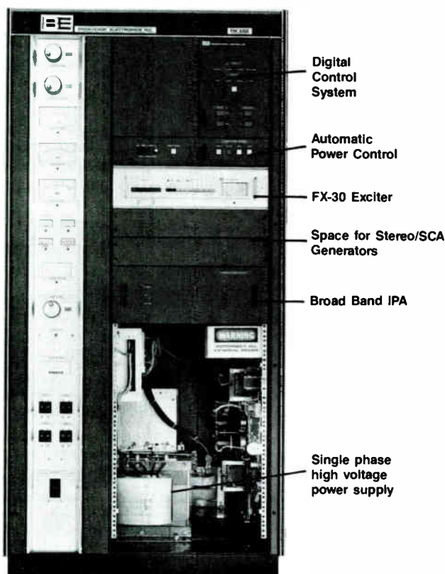
Front view Model FM-3.5A Transmitter.
