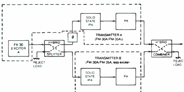
FIGURE 1 - BLOCK DIAGRAM, FM-70A/FM-60A
