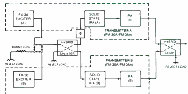
FIGURE 2 - BLOCK DIAGRAM, FM-70A/FM-60A WITH DUAL-EXCITER OPTION
