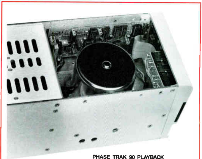
PHASE TRAK 90 PLAYBACK DC Servo Motor Assembly
