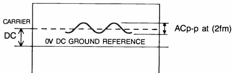
SCOPE DISPLAY OF HALF WAVE ENVELOPE DETECTOR OUTPUT
