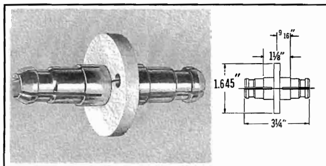
TYPE NO. 302-825 (Part No. 097 7084 00) — Anchor insulator-connector assembly, silver plated. Weight: 3 1/2 oz.
