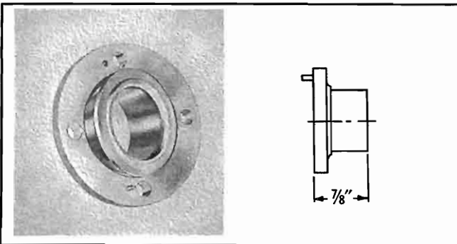
TYPE NO. 322-815 (NPN) — Adapter assembly, flanged to unflanged line, soft solder type, pressurized. No anchor insulator-connector, "O" ring or hardware. Weight: 5 1/2 oz.
