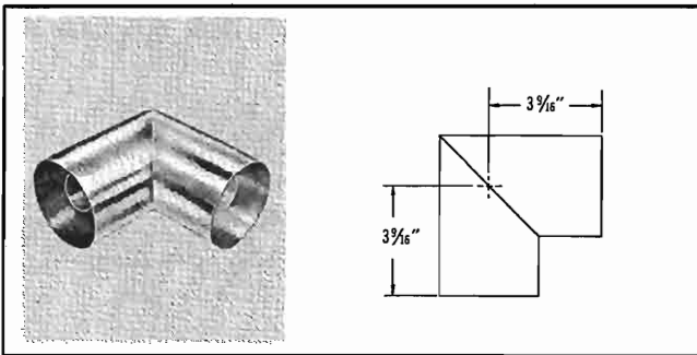
TYPE NO. 493-935 (NPN) — Elbow assembly, 90 degree, female, no flanges, equal legs. Unsupported inner conductor. Weight: 3 lbs.
