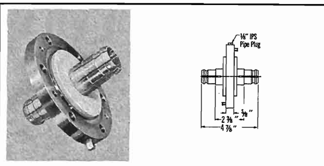
TYPE NO. 500-935 (NPN) — Gas barrier, zinc plated, with "O" ring and 2 1/4" long hardware. Incorporates 1/8" IPS gas inlet port. Weight: 3 lbs. 13 oz.
