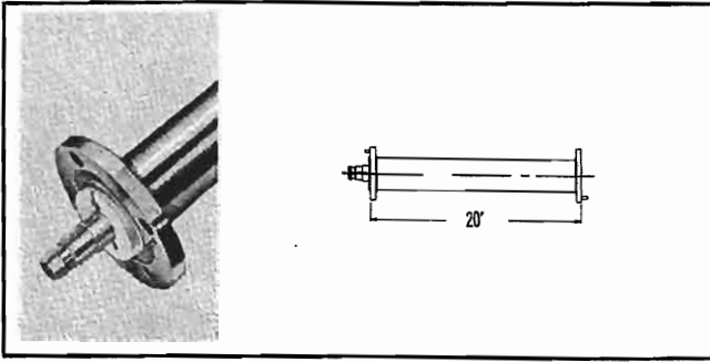
TYPE NO. 100-925 (NPN) — Line assembly, 20 ft. exact length, flanged both ends. Includes anchor insulator-connector assembly, "O" ring and hardware. Weight: 13 lbs. 3 oz.
