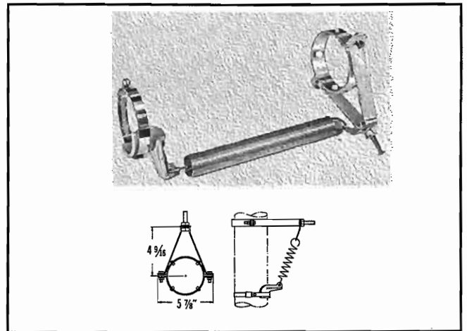
TYPE NO. 203-835 (NPN) — Hanger, spring suspension, direct attached, single line. Mounts through \frac{1}{8} " dia. hole. Line clamps and hardware supplied. Weight: 2 lbs. 12 oz.
