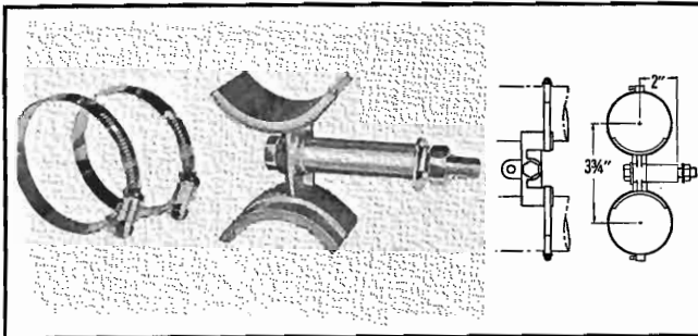
TYPE NO. 202-825 (NPN) — Hanger, fixed, direct attached, dual line. Mounts through 1/8" dia. hole. Line clamps and hardware supplied. Weight: 1 lb. 6 oz.
