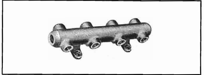
Type No. 39-150 MANIFOLD, has 10 ports 1/8" IPS female. (NPN).
