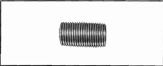
Type No. 34-150 NIPPLE, close, 1/8" IPS, brass. (NPN).
