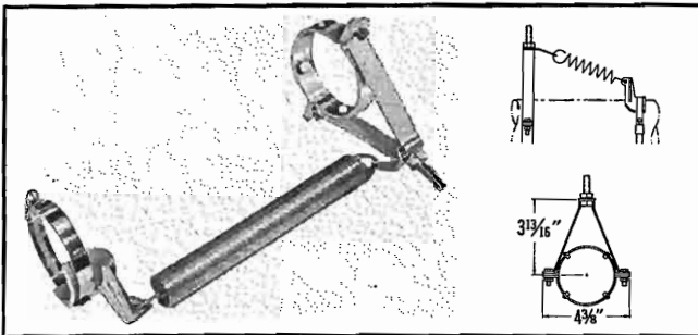
TYPE NO. 203-825 (NPN) — Hanger, spring suspension, direct attached, single line. Mounts through 1/8" dia. hole. Line clamps and hardware supplied. Weight: 2 1/2 lbs.
