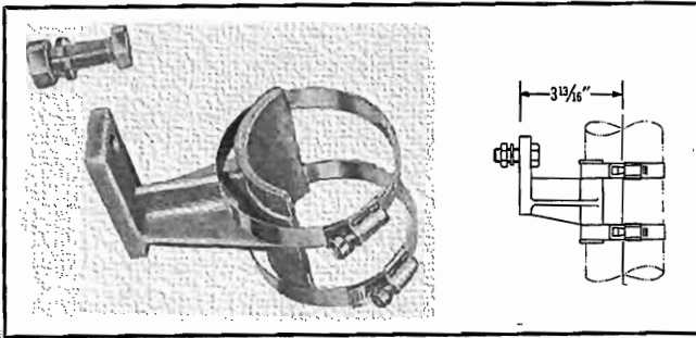
TYPE NO. 201-825 (NPN) — Hanger, fixed, direct attached, single line. Mounts through 1/8" dia. hole. Line clamp and hardware supplied. Weight: 1 lb. 4 oz.
