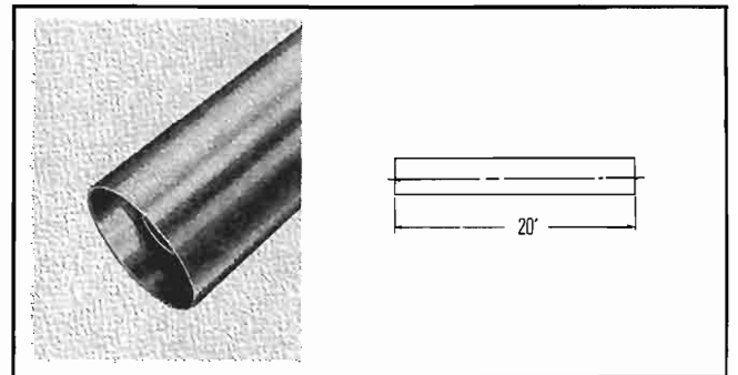
TYPE NO. 101-925 (NPN) — Coaxial line assembly, 20 ft. exact length, no flange. Weight: 121 1/2 lbs.
