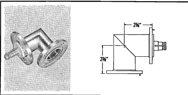
TYPE NO. 494-925 (NPN) — Elbow assembly, miter, 90 degree, male-female, swivel flanges. Includes one affixed male anchor insulator, "O" ring and hardware. Weight: 1 lb. 15 oz.
