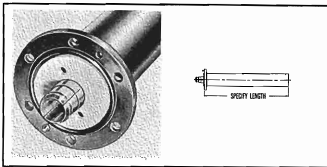
TYPE NO. 105-835 (NPN) — Line assembly, length to be specified, flanged one end. Includes anchor insulator-connector assembly, "O" ring and hardware. Weight: 3 lbs. + 2 1/2 lbs./ft.
