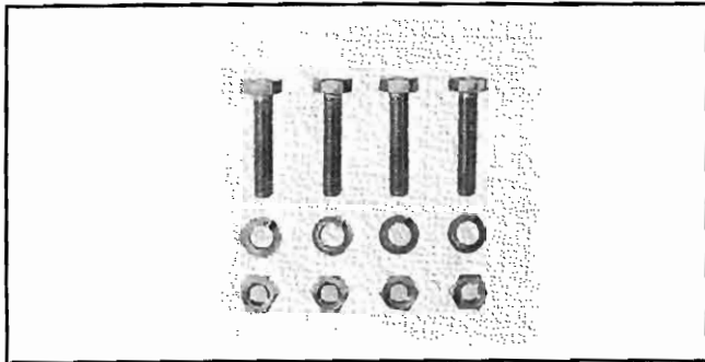
TYPE NO. 315-825 (NPN) — Hardware set for 1 5/8" flanges. Consists of 4 ea. stainless steel bolts, nuts and lockwashers, 5/16"-18 x 1 1/2" lg. Weight: 3 1/2 oz.
