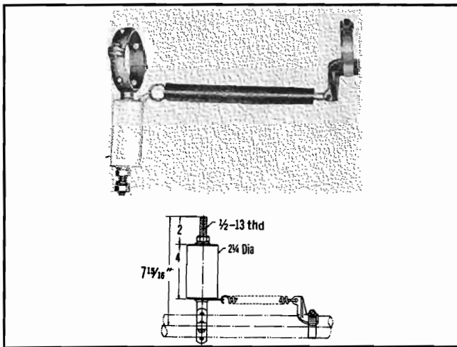
TYPE NO. 213-825 (NPN) — Hanger, insulated, direct attached. Mounts through \frac{1}{8} " dia. hole. Hardware supplied. Weight: 3 lbs. 11 oz.
