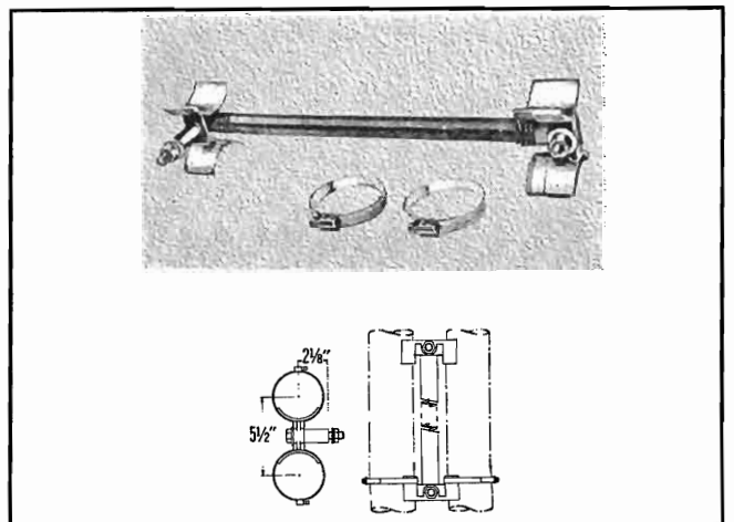
TYPE NO. 204-835 (NPN) — Hanger, spring suspension, direct attached, dual line. Mounts through \frac{1}{8} " dia. hole. Line clamps and hardware supplied. Weight: 4 lbs. 12 oz.
