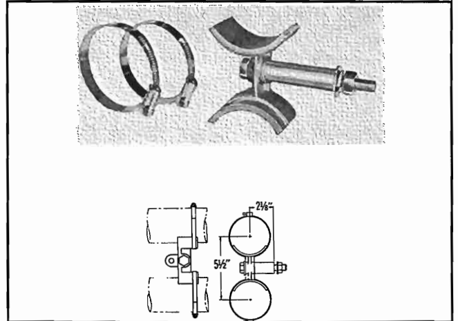
TYPE NO. 202-835 (NPN) — Hanger, fixed, direct attached, dual line. Mounts through \frac{1}{8} " dia. hole. Line clamps and hardware supplied. Weight: 2 lbs. 2 oz.
