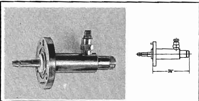
TYPE NO. 521-815 (NPN) — Adapter, EIA flange to type "N" female (UG-23D/U). Includes anchor insulator-connector, "O" ring and hardware. Incorporates 1/8" IPS port. Weight: 11 oz.
