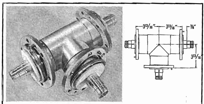
TYPE NO. 420-835 (NPN) — Tee assembly, reinforced, swivel flanges on all three legs, 3 13/16" center lines, affixed male anchor insulators all legs, includes "O" rings and hardware. Weight: 10 1/2 lbs.
