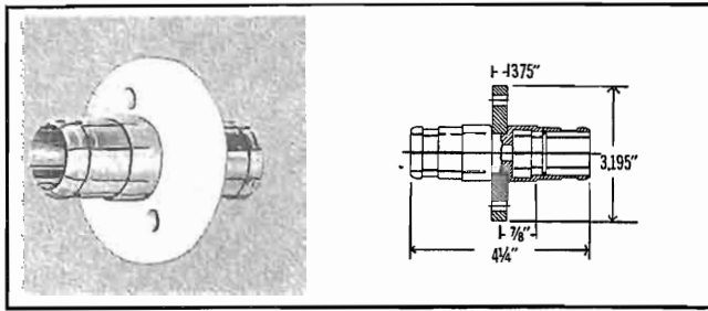
TYPE NO. 302-835 (NPN) — Anchor insulator-connector assembly, spring loaded, silver plated. TYPE NO. 303-835 (NPN) — Same as 302-835 except contact area is finished with Prodelube #8. Weight: 12 oz.
