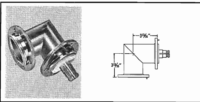
TYPE NO. 494-935 (NPN) — Elbow assembly, miter, 90 degree, male-female, swivel flanges. Includes one affixed anchor insulator-connector, "O" ring and hardware. Weight: 4 lbs. 9 oz.
