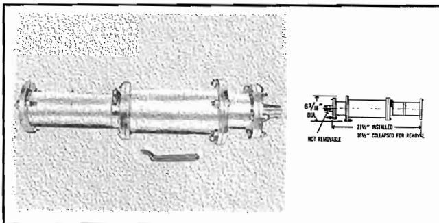
TYPE NO. 120-835 (NPN) — Breakaway section, EIA flanged both ends, permits separating the transmission line at any convenient point. Pressure tight. Weight: 14 lbs.
