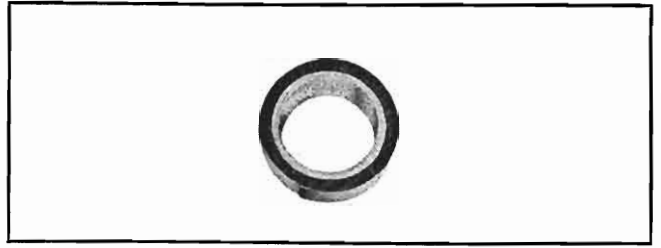
Type No. 38-150 POLYETHYLENE TAPE (3/4" wide x 20 ft.) used for weather-proofing connectors. Polyethylene tape is the only plastic which should be used on Spir-O-line cable and connectors. (NPN).
