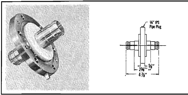
TYPE NO. 500-835 (Part No. 097 6725 00) — Gas barrier, with “O” ring gasket and 2 3/4” long hardware. Incorporates 1/8” IPS gas inlet port. Weight: 3 lbs. 13 oz.
