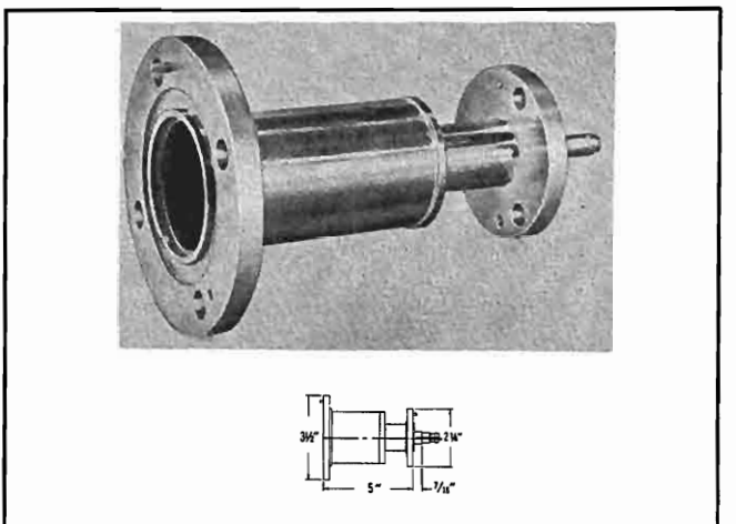
TYPE NO. 811-825 (NPN) — Reducer, step type, 1 5/8" to 7/8" 50 ohm, fixed flanges. Includes one 7/8" anchor insulator-connector assembly, "O" ring and hardware. Weight: 1 lb. 12 oz.
