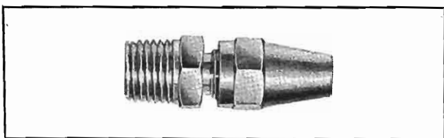
Type No. 26-150 FLARE FITTING, 1/4" OD copper tube, 1/4" IPS male (includes flare nut). (NPN).
