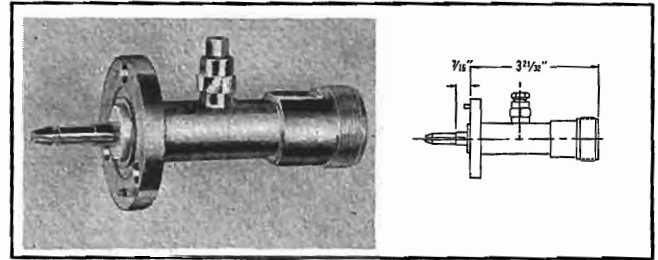
TYPE NO. 536-815 (NPN) — Adapter, EIA flange to "LC" female (UG-215/U). Includes one anchor insulator-connector, "O" ring and hardware. Incorporates 1/8" IPS port. Weight: 14 oz.
