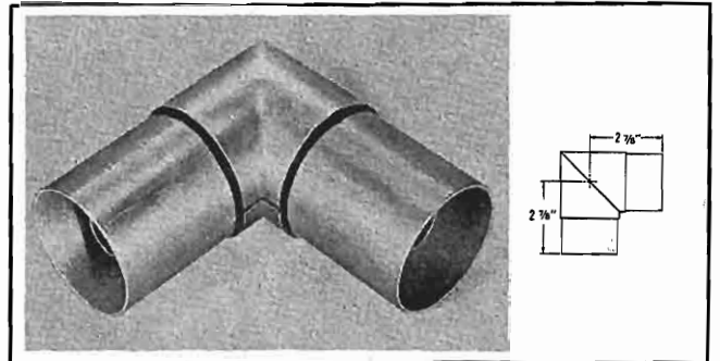
TYPE NO. 493-825 (NPN) — Elbow assembly, miter, 90 degree, female, reinforced, no flanges, equal legs. Inner conductor each leg cutback 1/8" from face of outer conductor. Weight: 15 oz.
