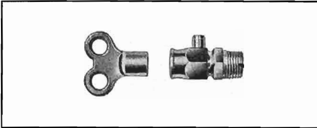
Type No. 33-150 BLEEDER VALVE, with key has 1/8" IPS male thread used wherever necessary when purging transmission line. (NPN).
