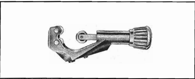
Type No. 35-150 TUBE CUTTER, for tube sizes 1/4" OD to 1 3/8" OD. (NPN).
