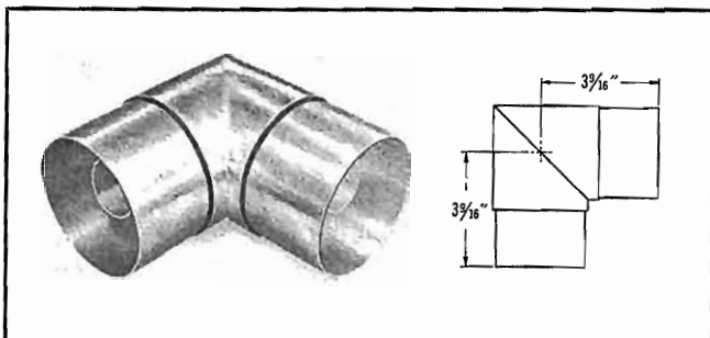
TYPE NO. 493-835 (NPN) — Elbow assembly, miter, 90 degree, female, reinforced, no flanges, equal legs. Inner conductor cut-back 1/8" from face of outer conductor. Weight: 3 lbs.
