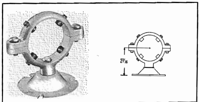
TYPE NO. 211-825 (NPN) — Hanger, slip type, flange mount supports transmission indoors or outdoors. Permits expansion. Weight: 14 1/2 oz.
