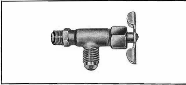
Type No. 32-150 NEEDLE VALVE, right angle type, has 1/8" IPS male thread, and side outlet is 1/4" OD copper tube. (NPN).
