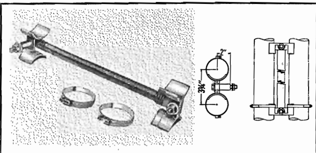
TYPE NO. 204-825 (NPN) — Hanger, spring suspension, direct attached, dual line. Mounts through 1/8" dia. hole. Line clamps and hardware supplied. Weight: 3 lbs.
