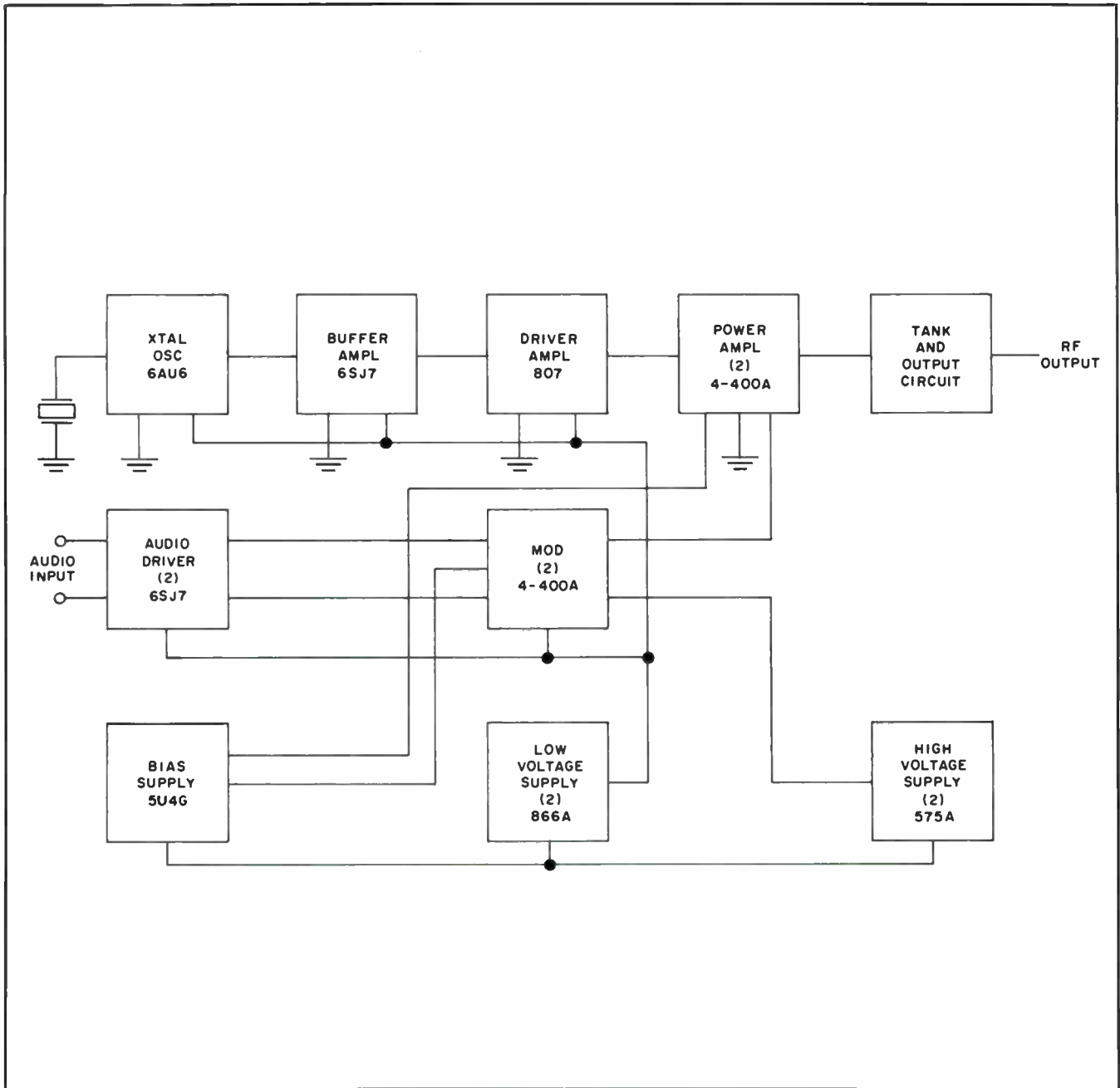
BLOCK DIAGRAM 20V-3
