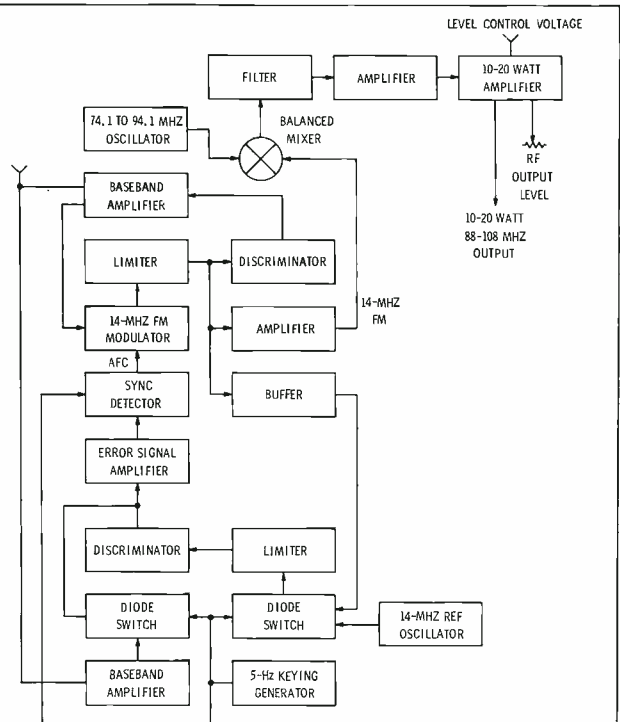
BLOCK DIAGRAM 310Z-1
