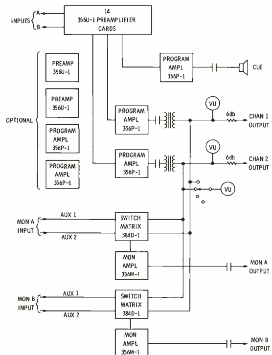
BLOCK DIAGRAM 212T-1
