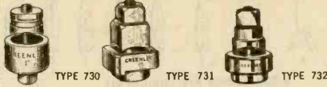
Type 730 Round Table Punches
