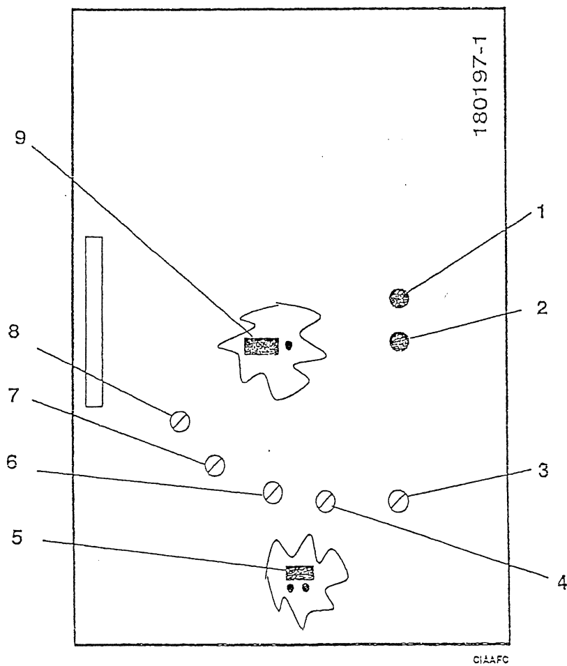
Figure 3-6 Audio/AFC, A3.
