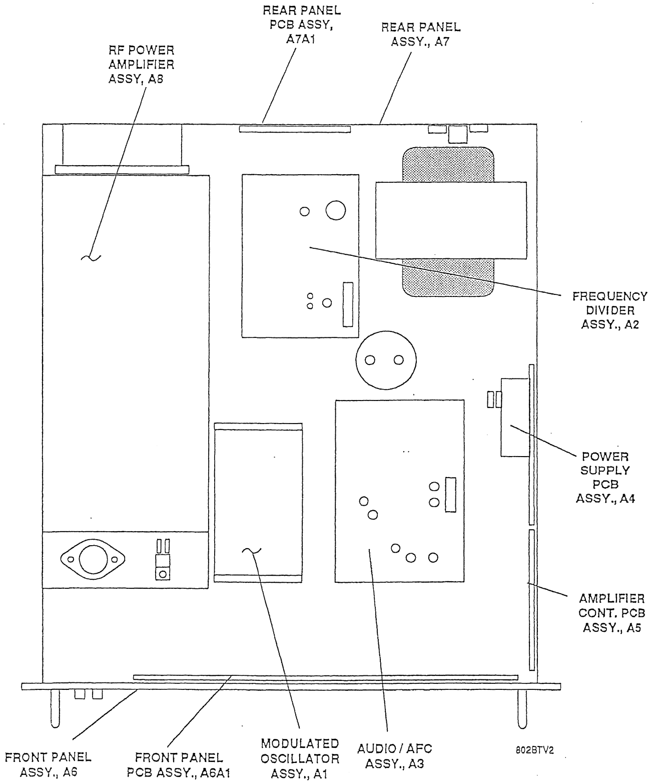
Figure 4-1 Type 802B FM Exciter Assembly Locator.
