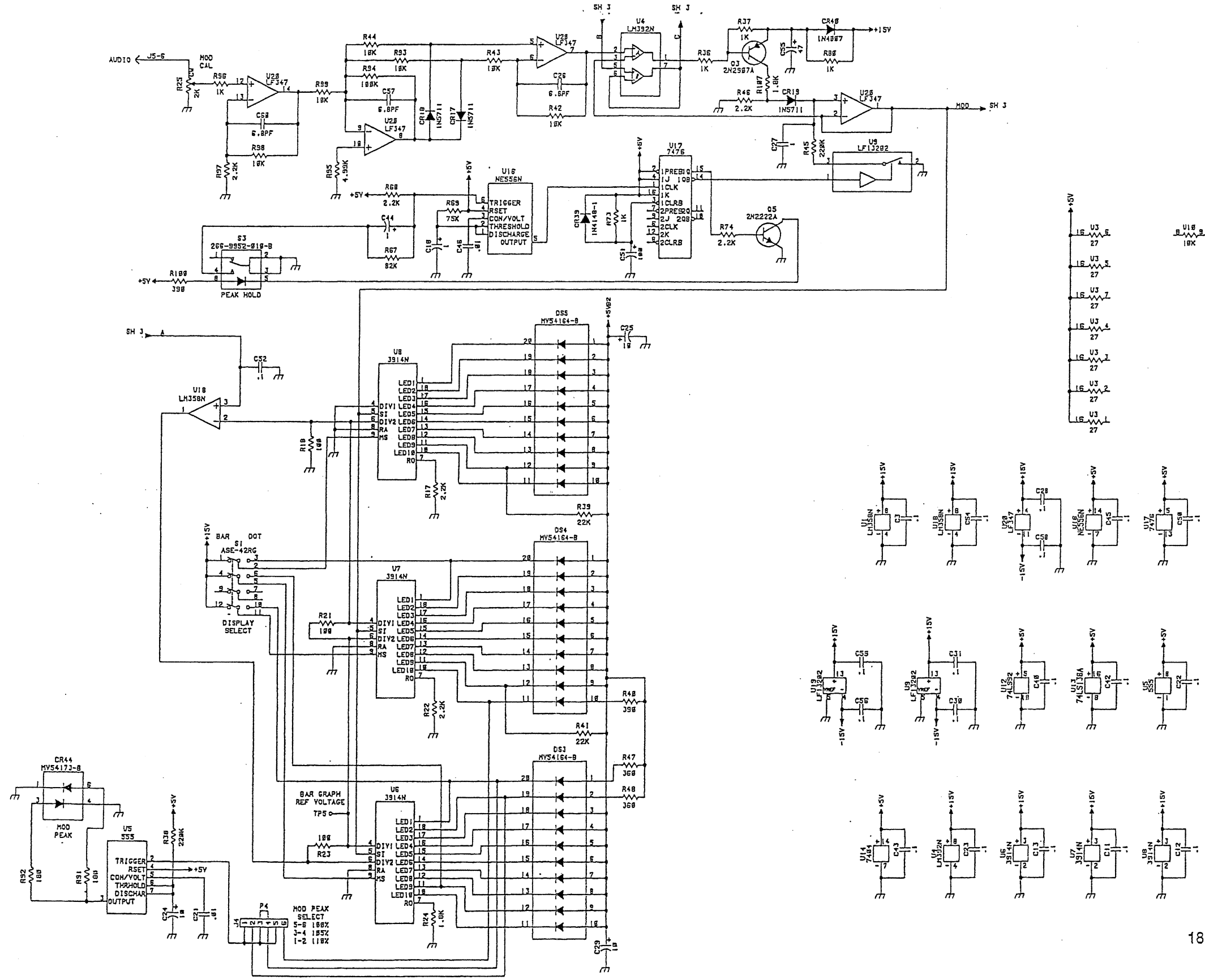
Figure 7-7 Front Panel PCB (Sheet 2).
