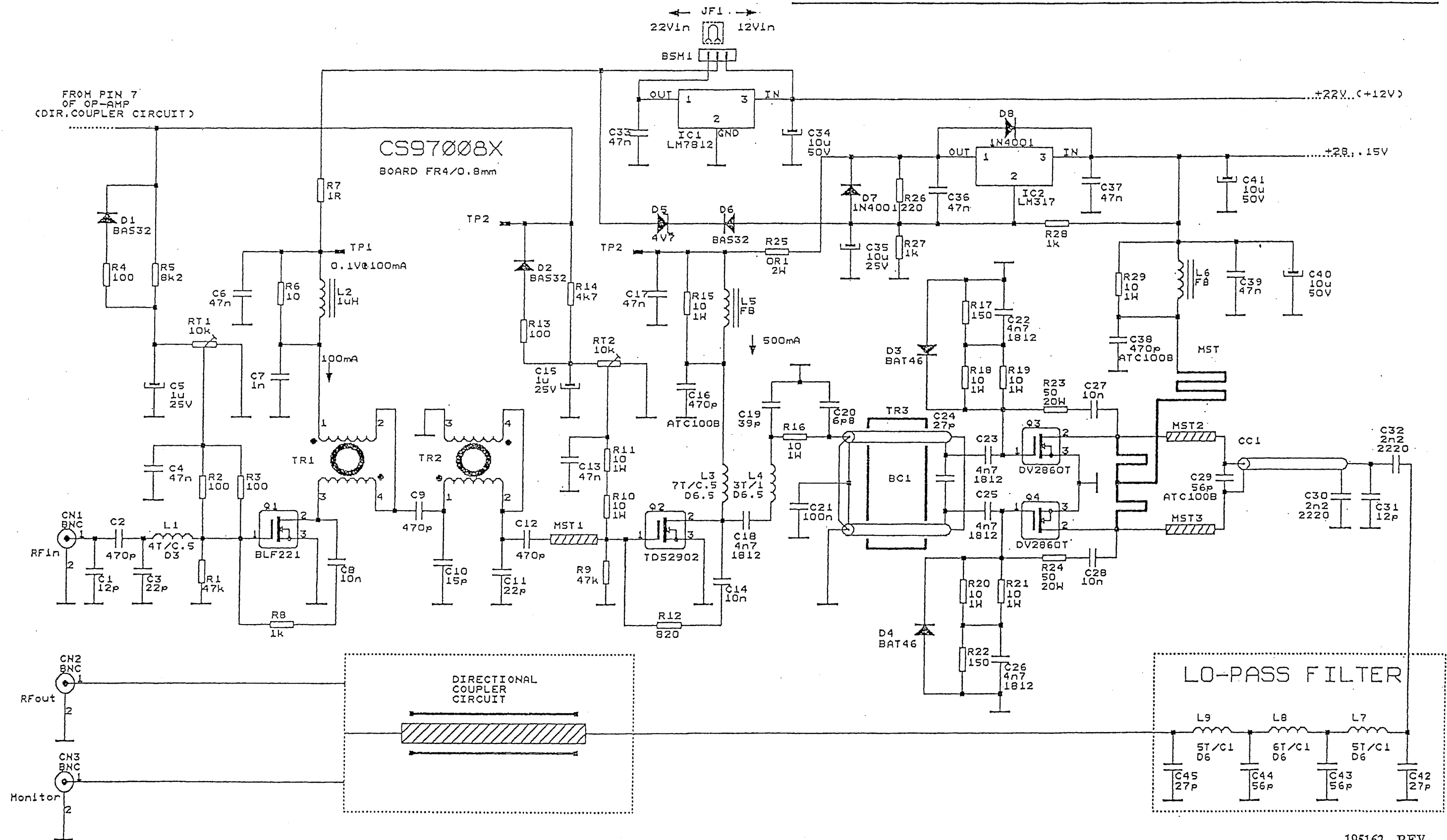
Figure 7-9 50 Watt Amplifier Card.
