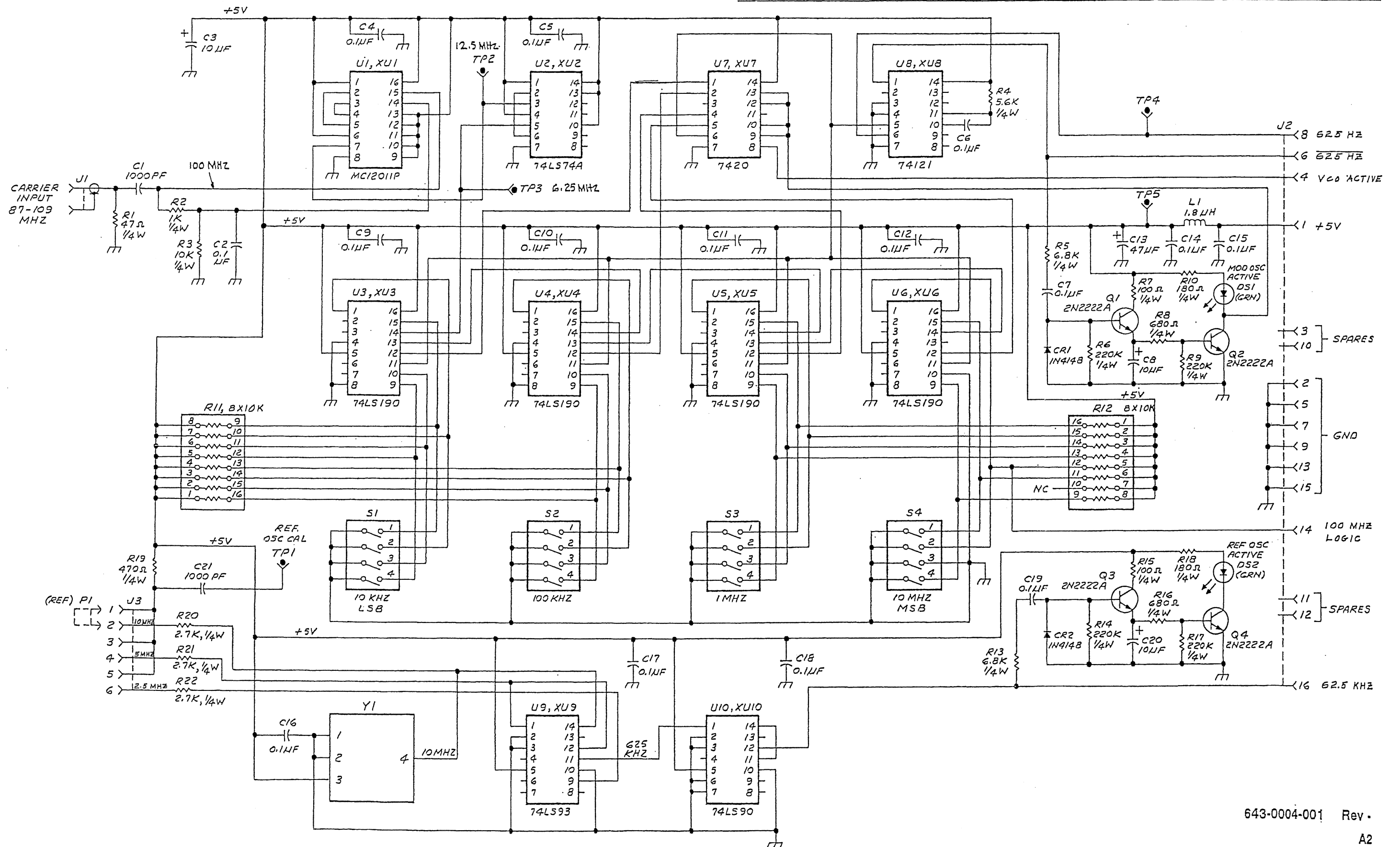
Figure 7-3 Frequency Divider PCB.
