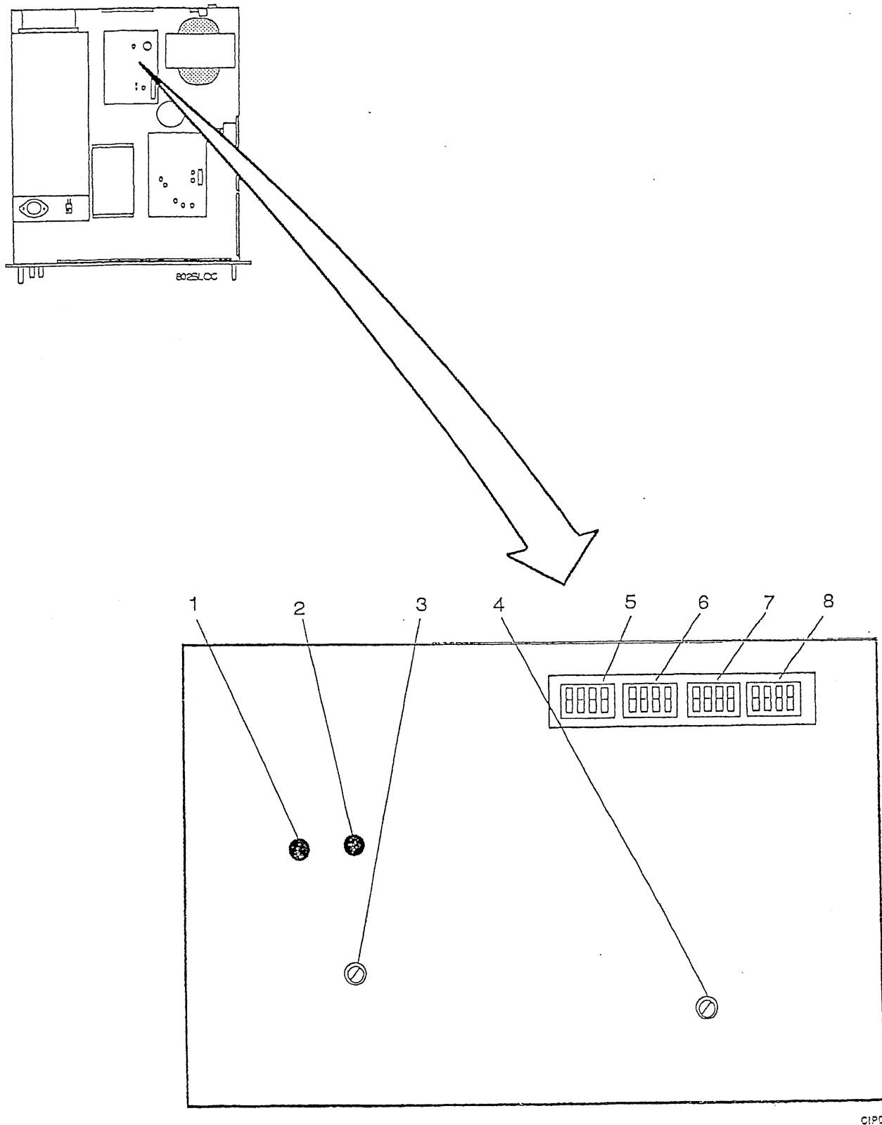
Figure 3-5 Frequency Divider, A2.
