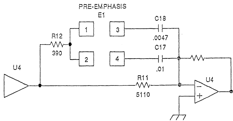
PARTIAL SCHEMATIC, AUDIO AFC
