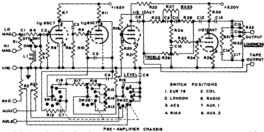
PRE-AMPLIFIER CHASSIS
