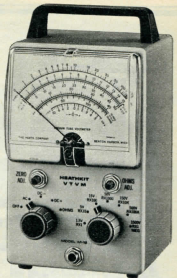
Heathkit IM-18 — our most popular VTVM
