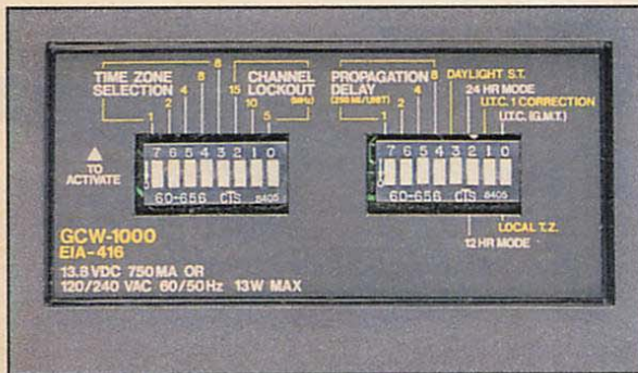
Case bottom dip switches for time correction adjustments
