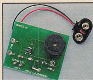
Audio oscillator circuit
