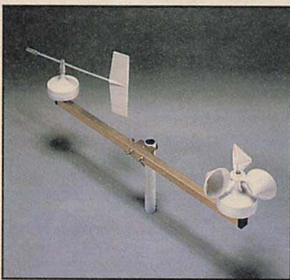
Precision boom assembly includes wind vane and cups for respectively measuring wind direction and speed.
