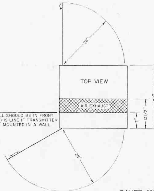
BAUER MODEL 707 AM BROADCAST TRANSMITTER
