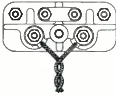
Set for 200/250 volts Diagram 9
