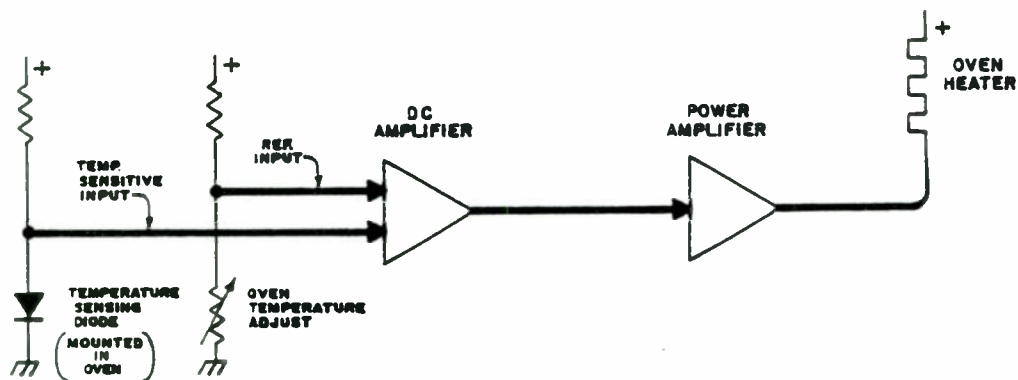
PCL-505 AUTOMATIC FREQUENCY CONTROL (MONAURAL OR COMPOSITE)
