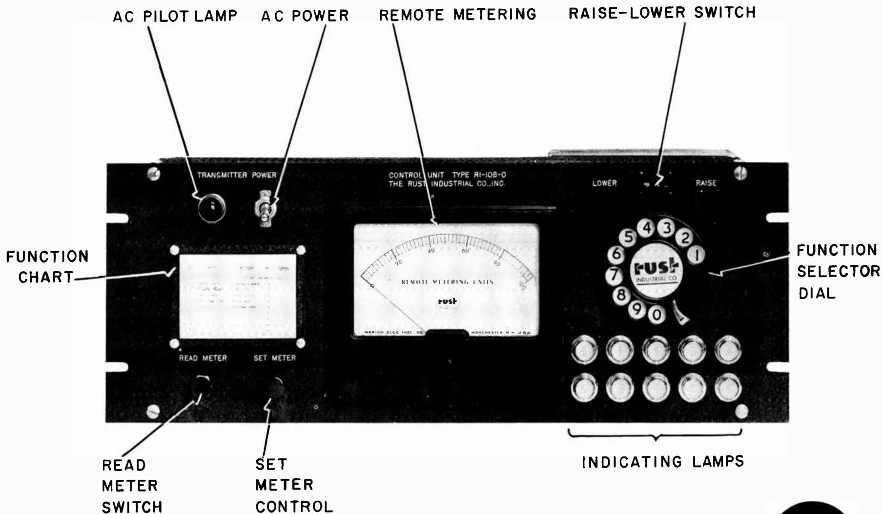
COMPONENT LOCATIONS FRONT OF RI-1080 UNIT
