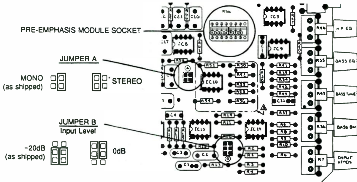
Fig. 2: Jumper Positions and Component Locations, Card #4
