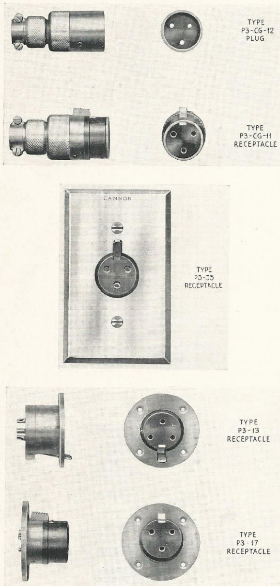
Figure 13—Plugs and Receptacles
