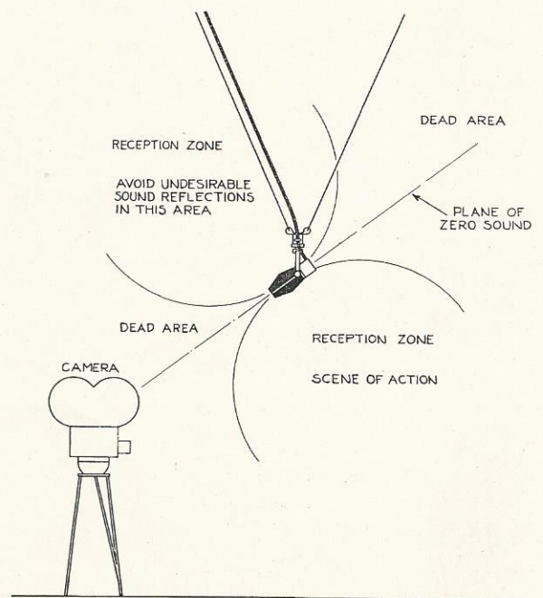
Figure 12—Camera Location for Sound Motion Picture Work
