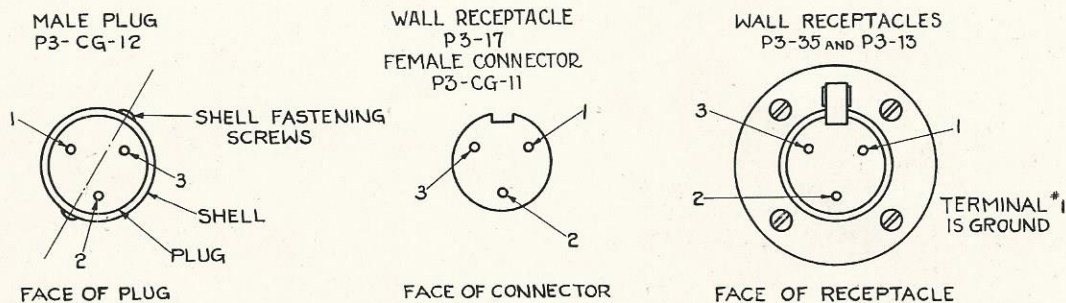
Figure 6—Plug and Receptacle Connections
