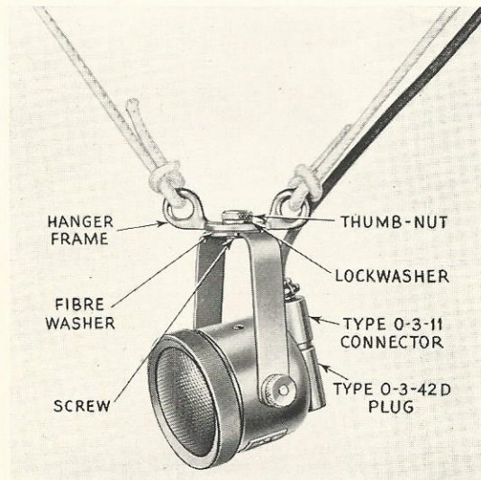
Figure 3—Type 50-A Microphone Suspended from a Type UP-4277 Suspension Hanger
