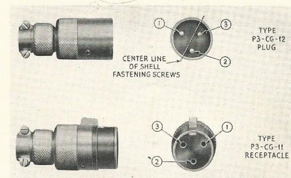
Figure 4—Plugs and Receptacles Frequently Used for Microphone Connections
