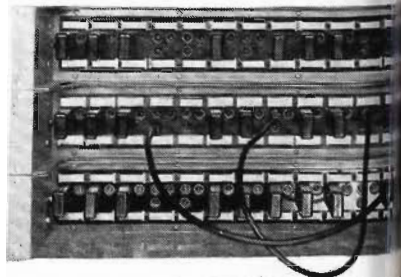
Video Jack Panel, MI-26245. For patching and/or sync signals. Includes 12 groups of contact assemblies (3 per group). Video jack plugs and cords.
