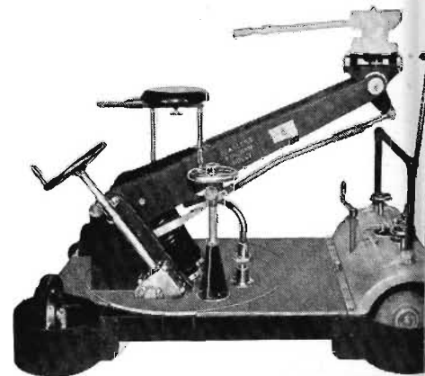
"MAGIC LOCK" BOOM STAND, KS-4A— The handiest microphone boom ever designed for TV studios. Convenient locking devices enable operator to control it with one hand. No set screws. No release mechanisms. No slipping. Each adjustment locks into position. Moves in a 180-degree arc and a base radius of 26 inches. Silent in operation.
