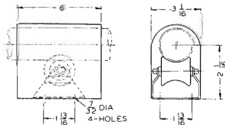
ROLLER MI-19312-35
