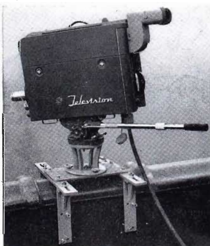
Parapet Clamp Support, MI-26189, as used with Hi-Hat to support RCA Field Camera
