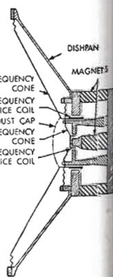
DETAILS OF RCA DUO-CONE DESIGN
