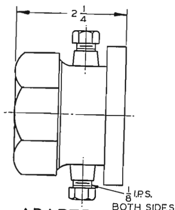
ADAPTER MI-19310-4
