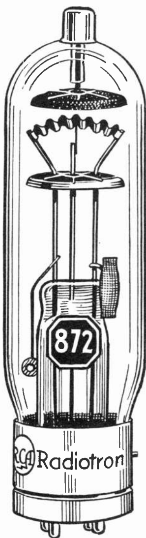
RCA-872
