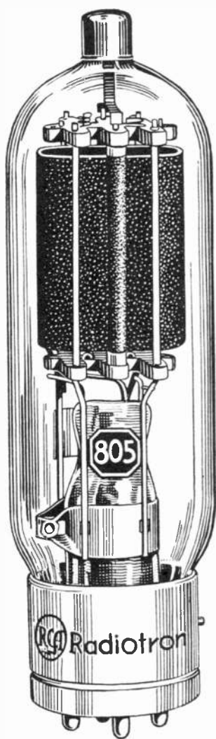
RCA-805
