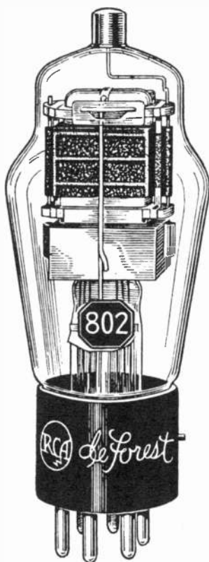
RCA-802
