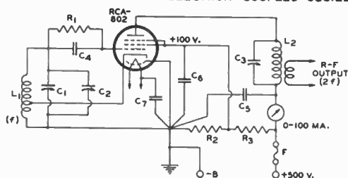
ELECTRON-COUPLED OSCILLATOR
