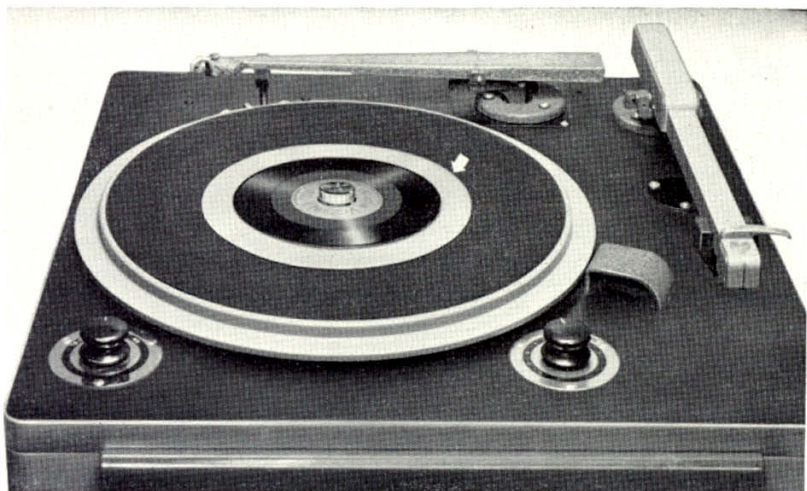
Arrow above points to the MI-11886, 45 RPM Adaptor, mounted on the 70-D Turntable
