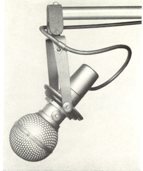
BK-5A Microphone with Wind Screen, MI-11011, and Boom Unit, MI-11012.
