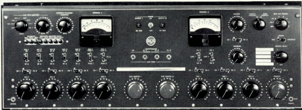
Etched front panel of the BC-6A Console showing entire operating facilities.
