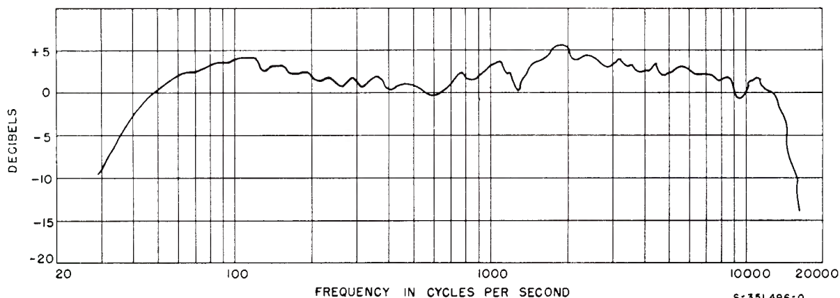
Frequency Response Curve of LC-1A Speaker.
