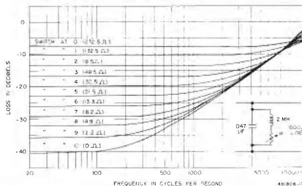
Frequency characteristic of Type BE-2A Line Equalizer.
