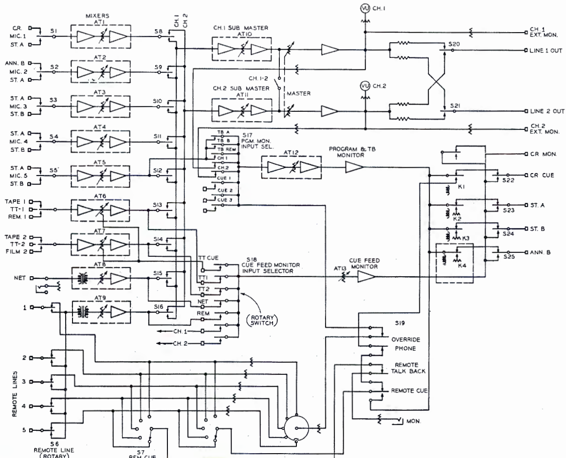
Simplified block diagram of the BC-6A Dual-Channel Audio Consolette.
