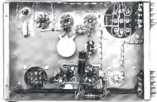
View of BA-12A Utility Amplifier Chassis showing component wiring
