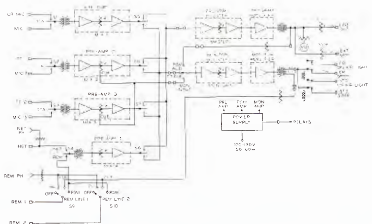
Simplified block diagram of BC-5A Console.
