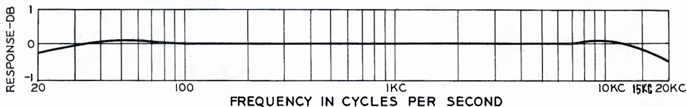
FREQUENCY RESPONSE MI-11246-A PROGRAM AMPLIFIER TYPE - BA-23A
