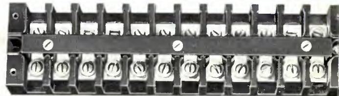
Power Terminal Block MI-456B with cover removed.
