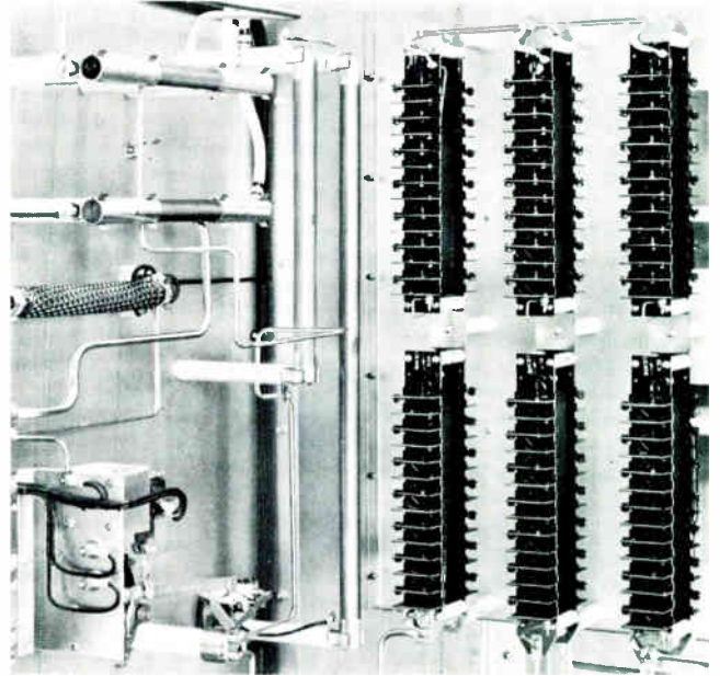
Silicon rectifiers are modularized for easy maintenance.
