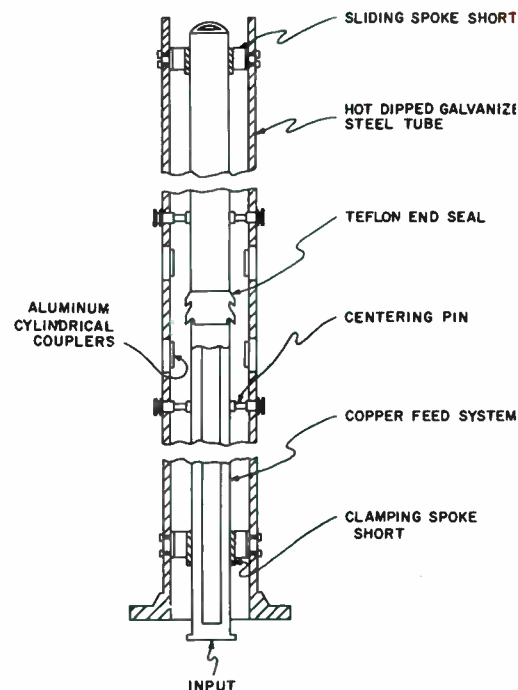
Cross section of typical UHF Pylon Antenna.
