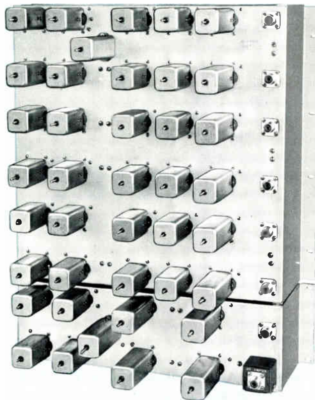
Rear view of Phase Equalizer Equipment showing one Amplitude Equalizer unit mounted in lower right corner on the Low Frequency Chassis.
