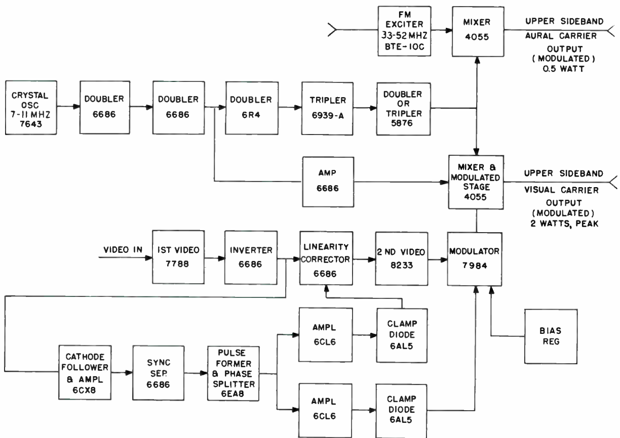
Aural/Visual Exciter/Modulator Block Diagram.
