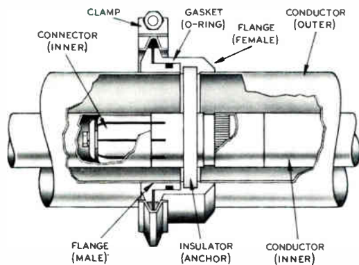
Universal Line Connector Assembly Cutaway.
