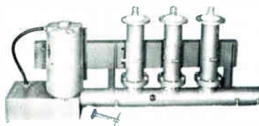
Motor Driven Coaxial Switch.
