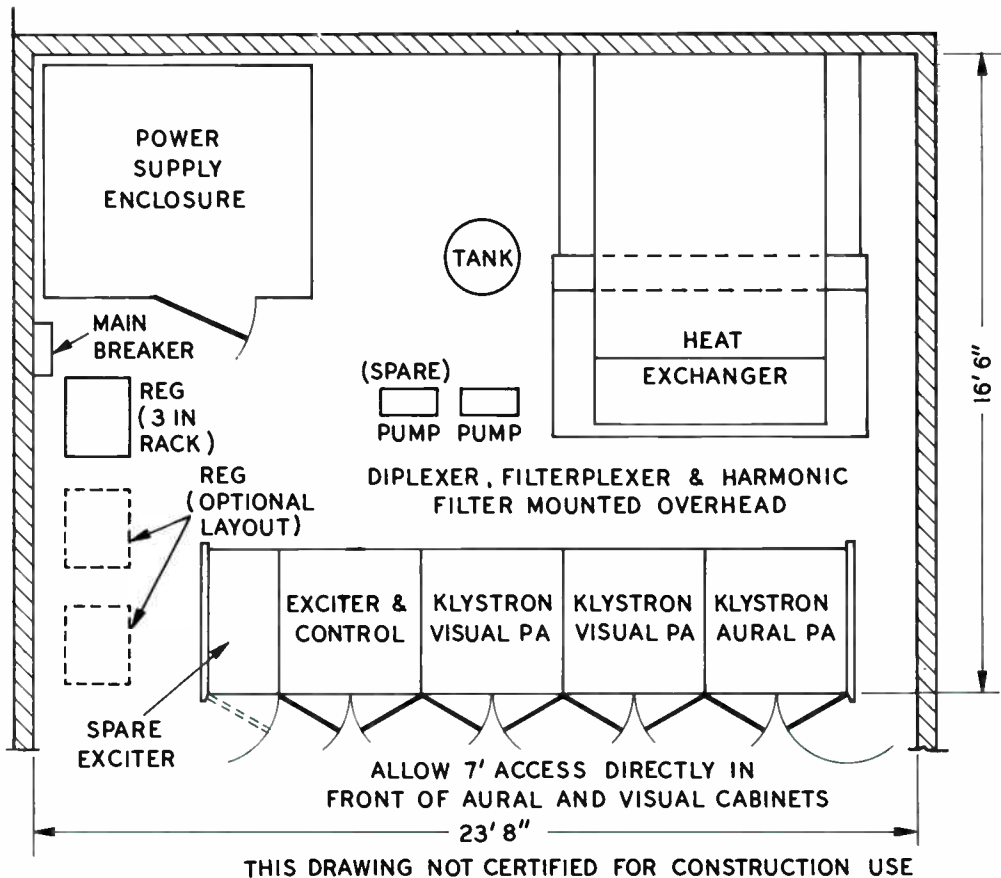
Space Saving Floor Plan of TTU-50C1 UHF Television Transmitter.
