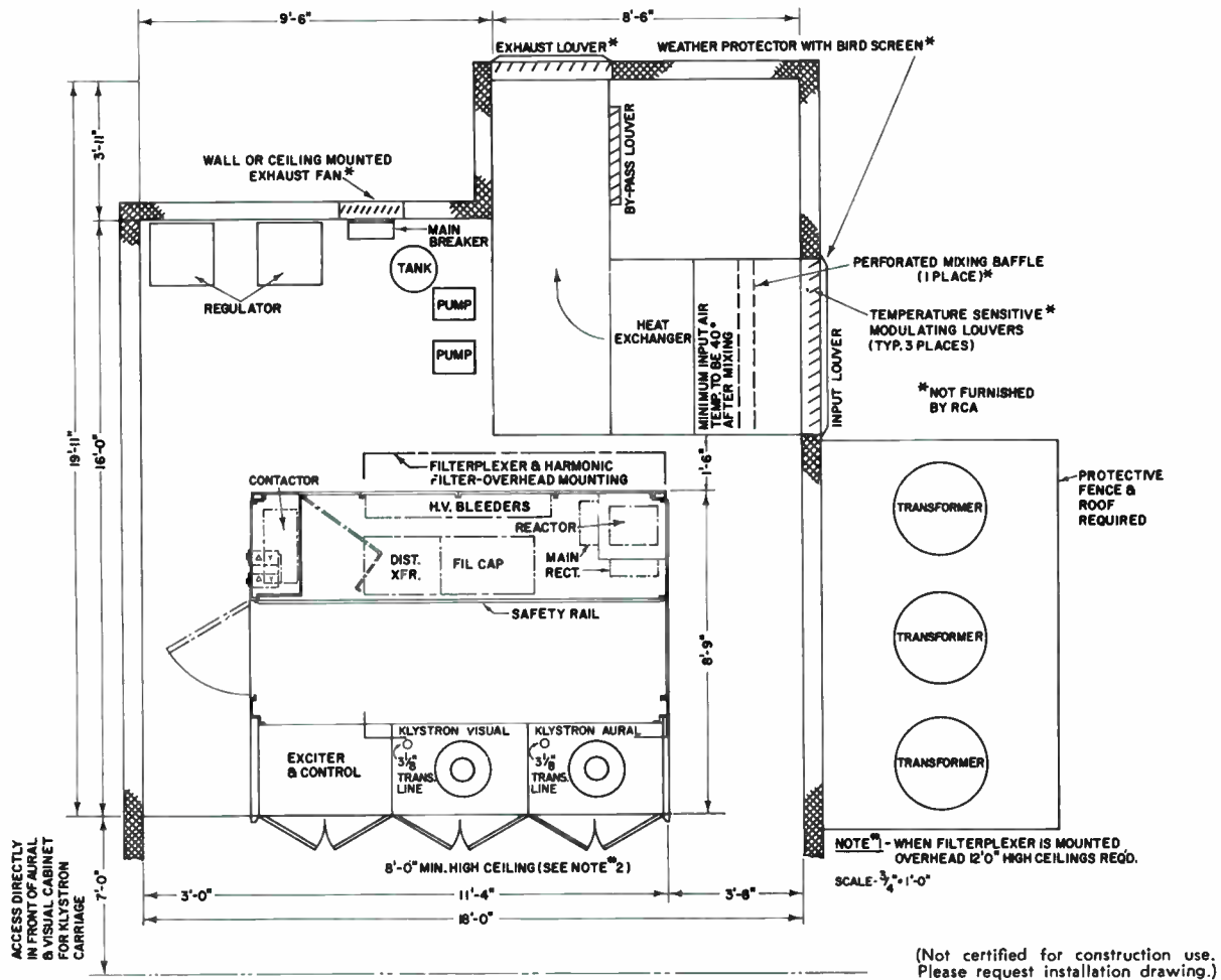
Space Saving Floor Plan of TTU-30A UHF Television Transmitter.
