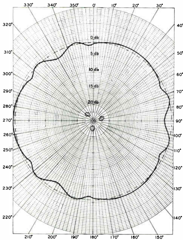
FIG. 14. Mounted Around Tower Channel 14, 10 ft. 0" face
