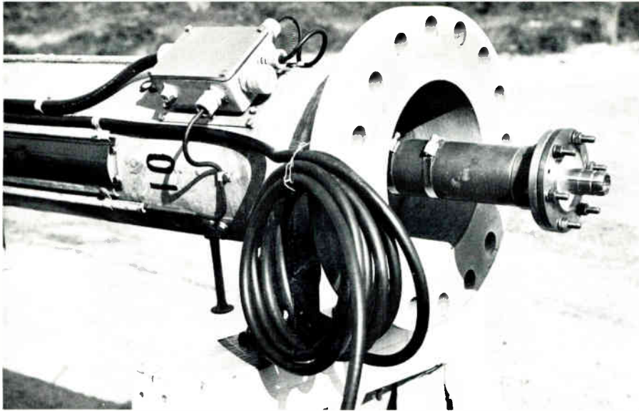
Base of UHF antenna showing deicer, deicer junction box and beacon cable. The antenna input is also shown.
