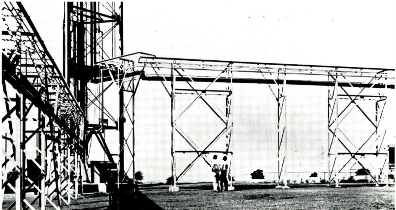
TV tower showing horizontal transmission line runs protected by ice shields.
