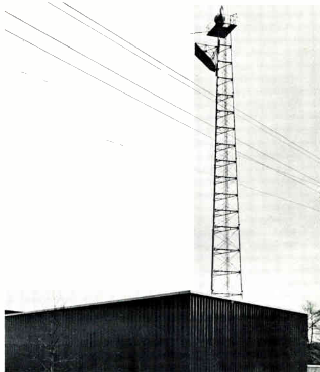
Self-supporting 135-foot microwave tower at Station WAVE-TV showing two receiving dishes on platform—one fixed and one rotatable. The reflector handles a 7000 MHz STL microwave and also a 2000 MHz STL, both with roof-mounted antennas.
