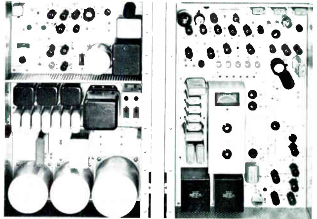
Exciter/modulator employing premium 10,000 hour tubes.
