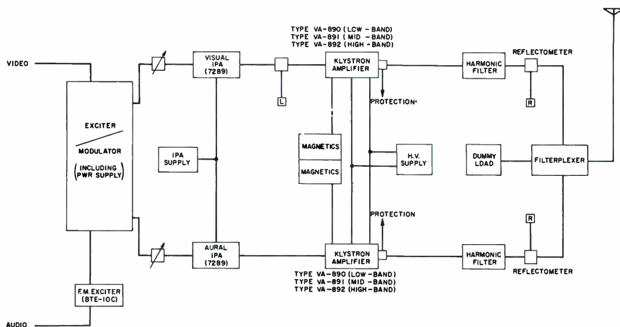
Block Diagram of TTU-30A UHF Television Transmitter.
