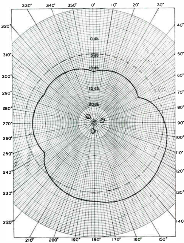
FIG. 10. Top Mounted Horizontal Directive Gain 2.43, 3.9 dB.
