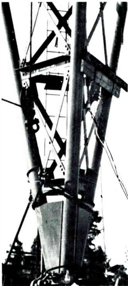
Typical anchorage for pivoted base type of guyed tower. Connected at a single point, the tower will remain upright and plumb even if the foundation shifts unevenly.
