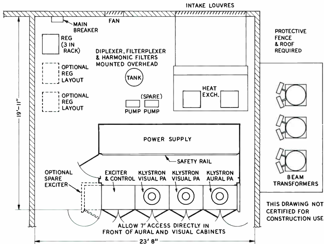
Space Saving Floor Plan of TTU-50C UHF Television Transmitter.
