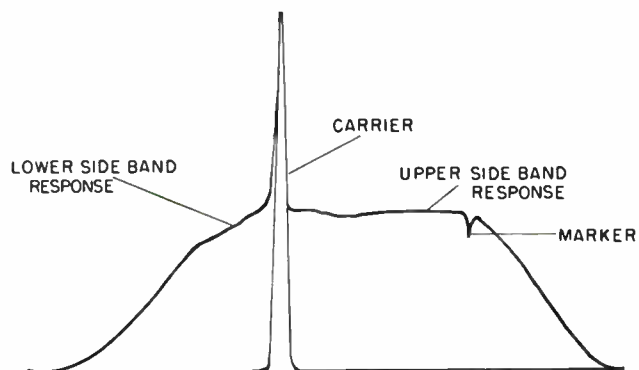
Typical response pattern of a TV transmitter using BW-5C Sideband Analyzer, illustrating the wave shape of lower and upper sidebands.
