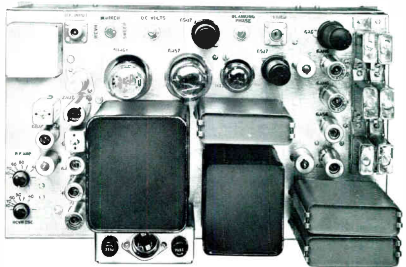
Rear View of Sideband Response Analyzer BW-5C.
