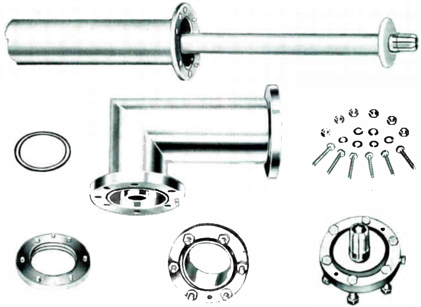
Flanged UHF Bolt Flanged Teflon Coaxial Transmission Line.
