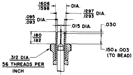
CONNECTOR DETAIL
