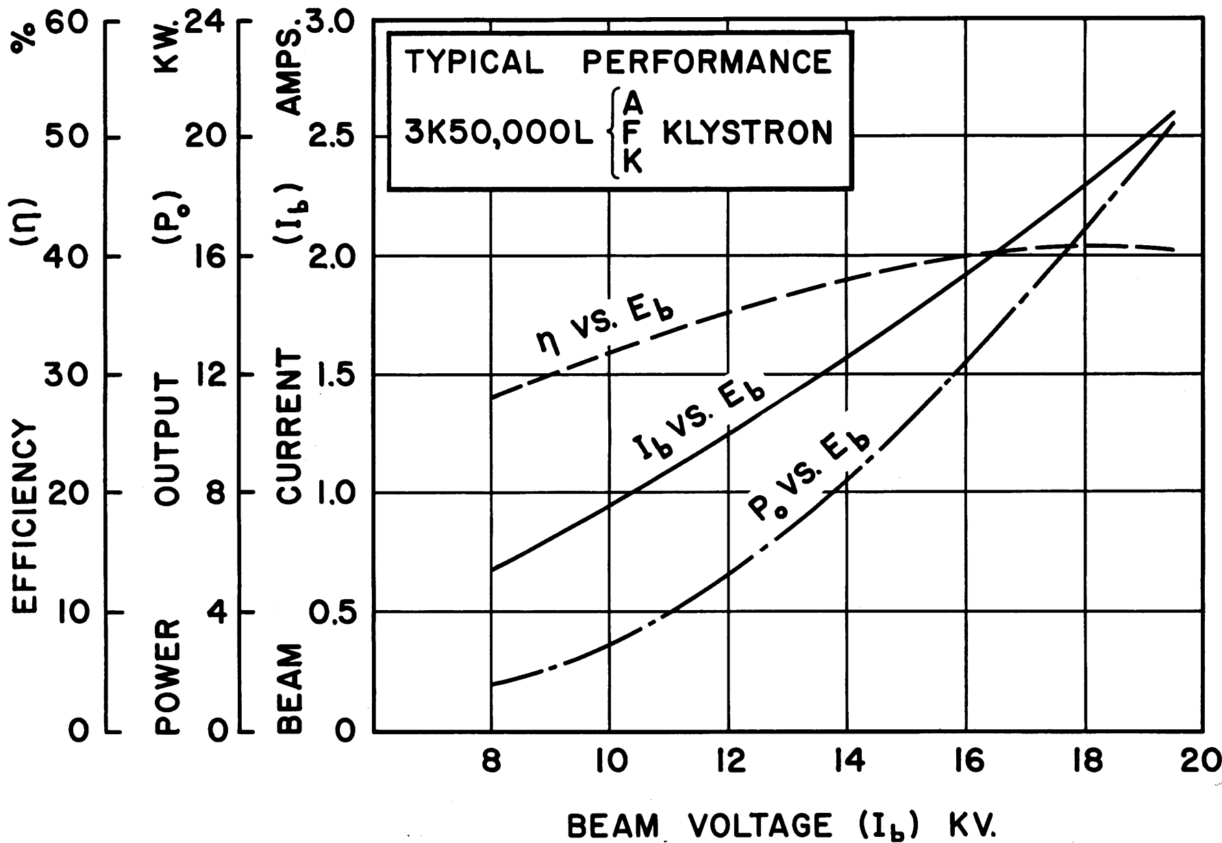
BEAM CURRENT, POWER OUTPUT AND EFFICIENCY VS. BEAM VOLTAGE
