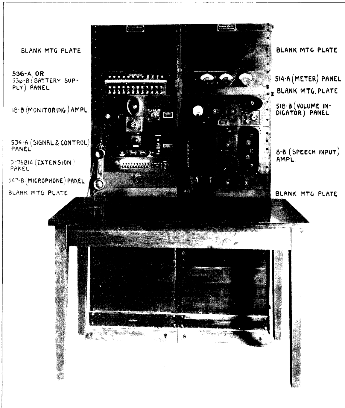
1-E SPEECH INPUT RACKS—23117-C
