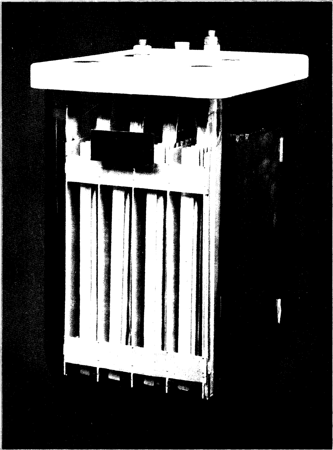
100-A ELECTROLYTIC FILTER CONDENSER—22737
